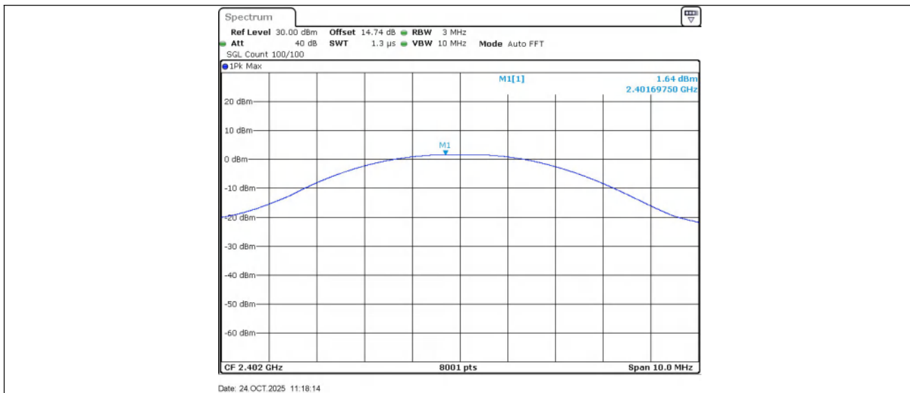
BLE_1M_Ant1_2402
