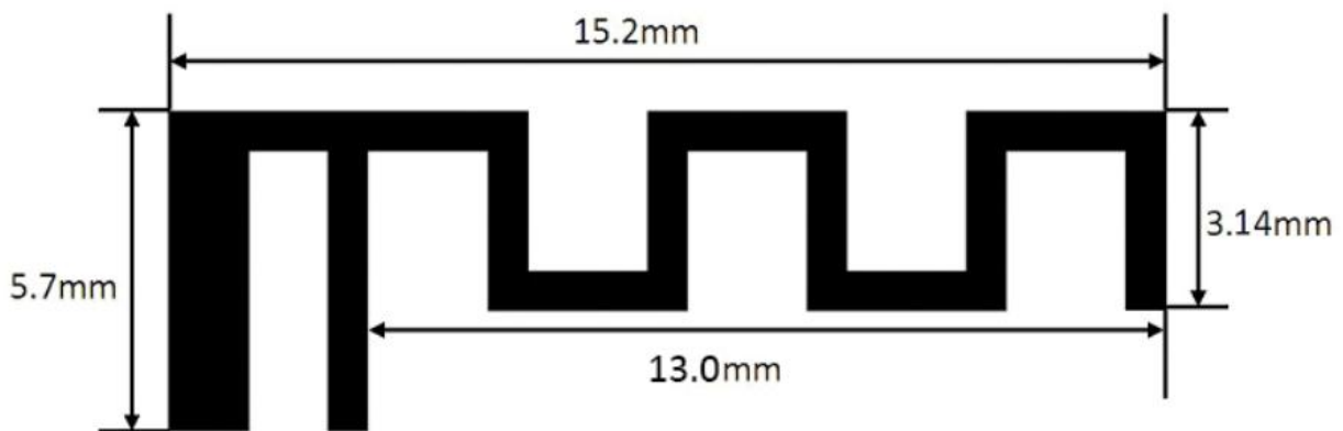
Antenna Photo & Length (mm)
