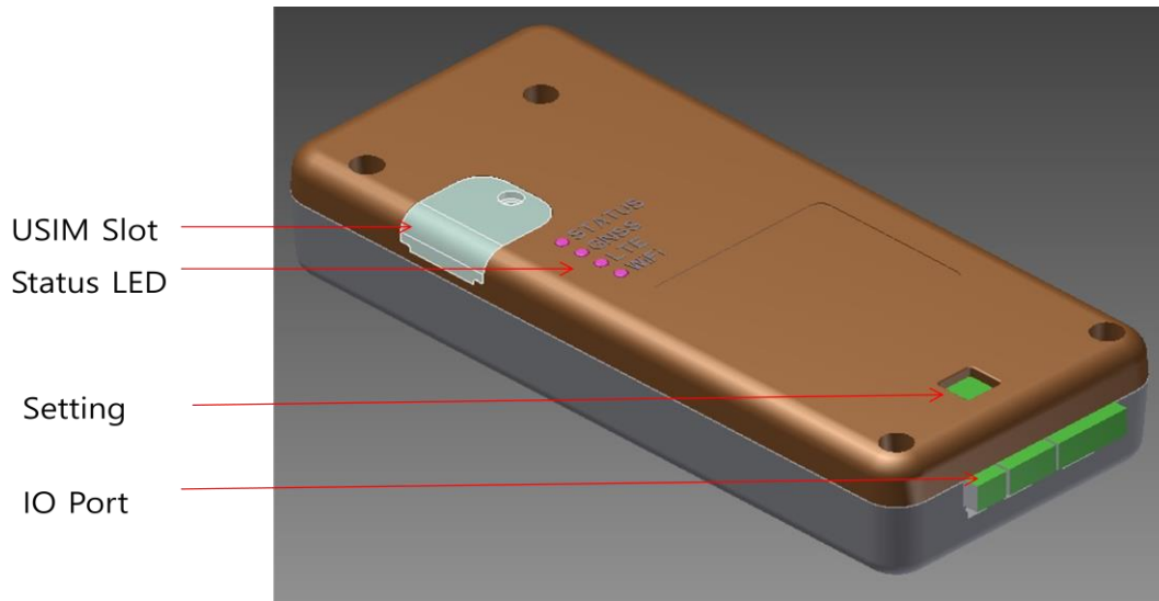
Figure 3 DC-20 Terminal
