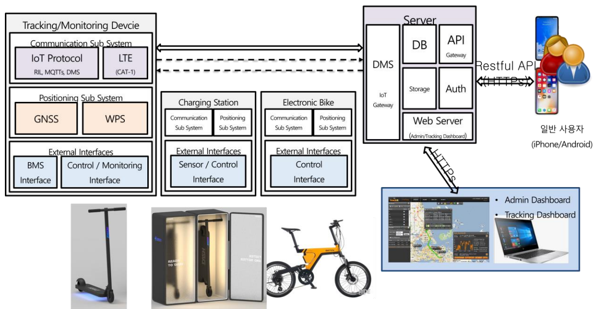
Figure 1 DC-20 System
