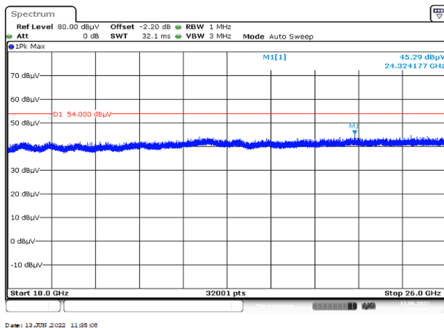
Plot 4: 18 GHz to 26 GHz, TX mode, valid for all channels, vertical & horizontal polarization, 1 Msps
