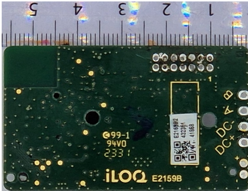
Figure 6: HW version E2159B2, bottom view.
