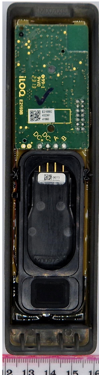
Figure 1: Internal view. Without Potting sealant.
