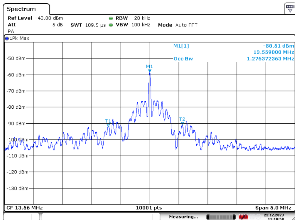
Figure 9: Occupied Bandwidth 99 %
