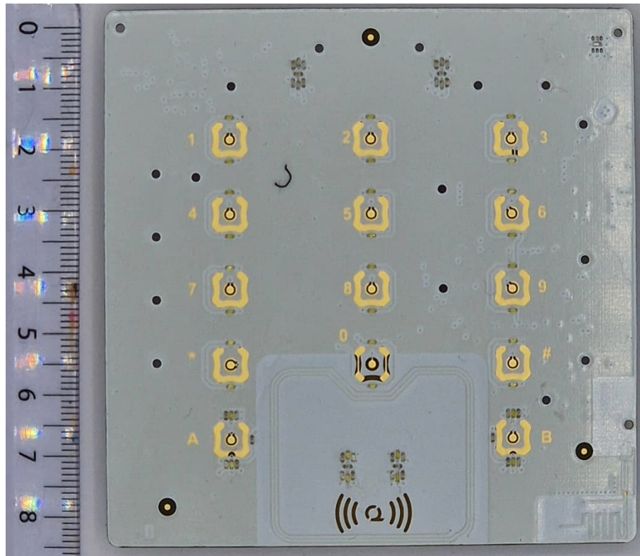
Figure 2: HW version E21336C, top view.
