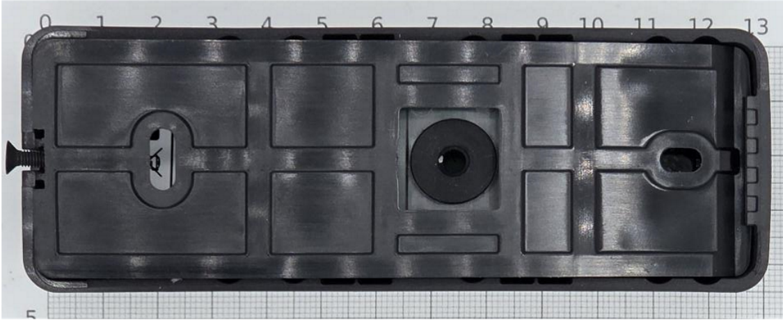
Figure 6: N510.100, Bottom view. Mounting bracket assembled.
