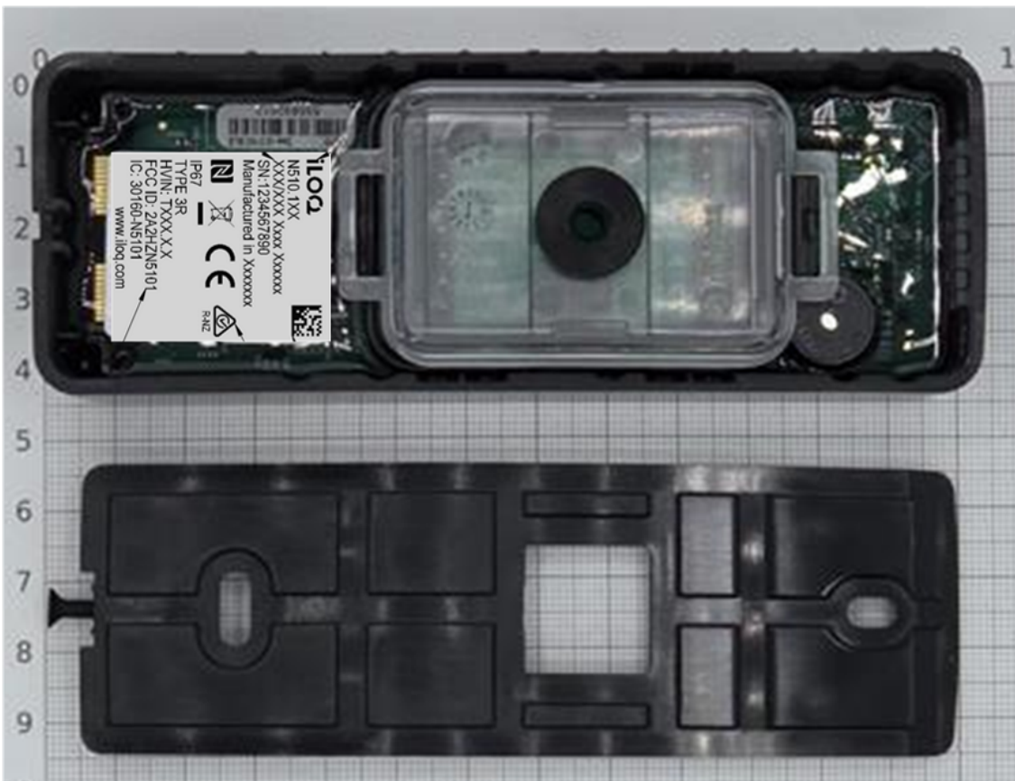
Figure 14: N510.110, Bottom view.
