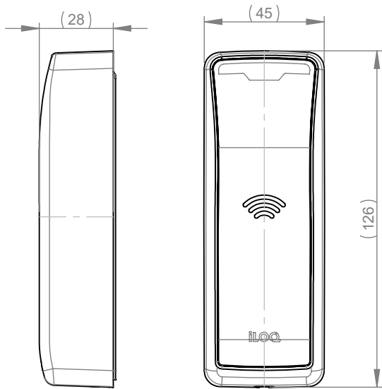
Main reference dimensions
