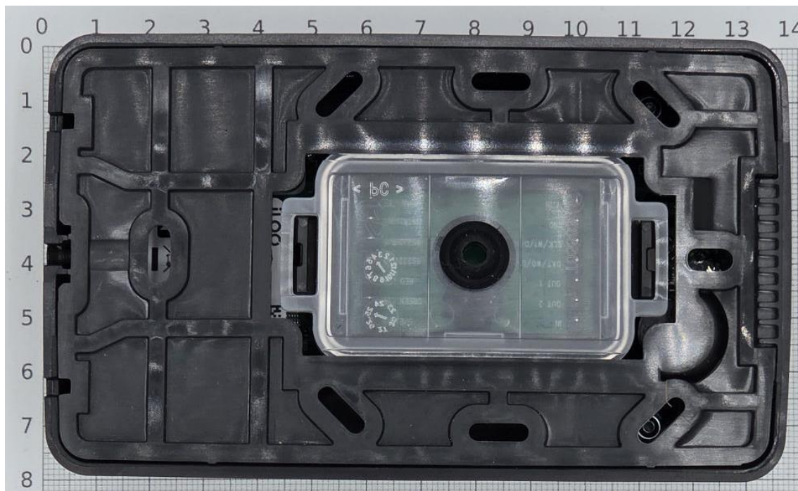
Figure 13: N510.220, Bottom view. Mounting bracket assembled.
