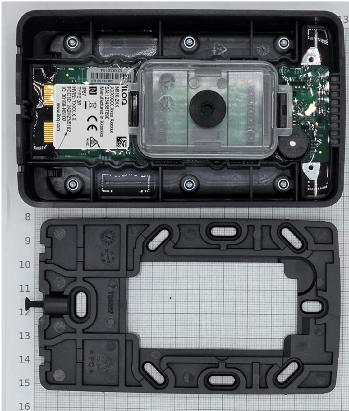
Figure 7: N510.200, Bottom view.
