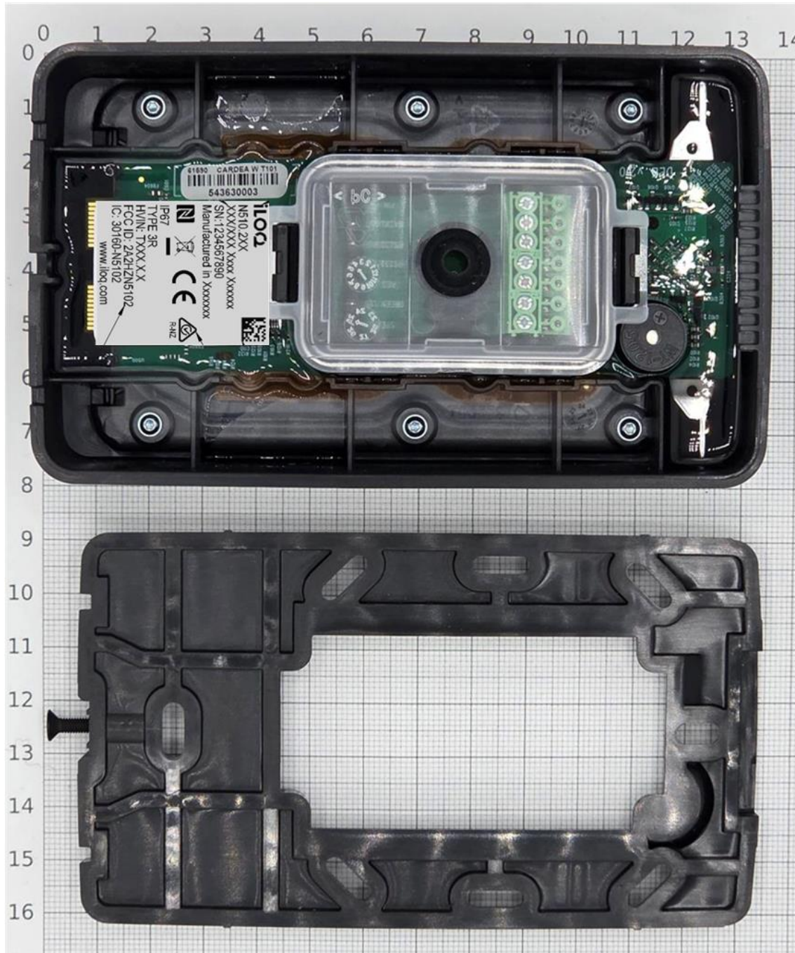
Figure 14: N510.220, Bottom view.
