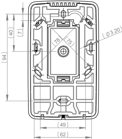
Installation reference dimensions
