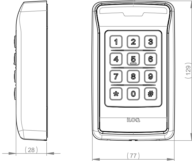
Main reference dimensions
