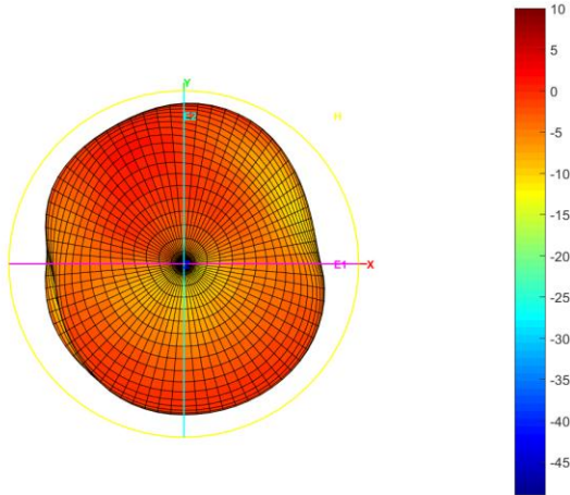
Total_3D_H_2.45GHz
