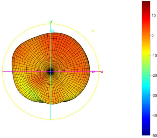
Total_3D_H_5.5GHz
