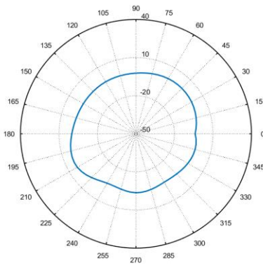
Total_Polar_E1_5.5GHz
