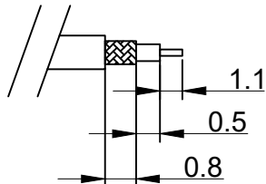
MHF-4L STRIPPING DIM'S
