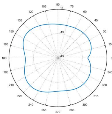
Total_Polar_E1_2.45GHz
