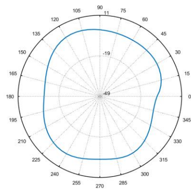
Total_Polar_E2_2.45GHz
