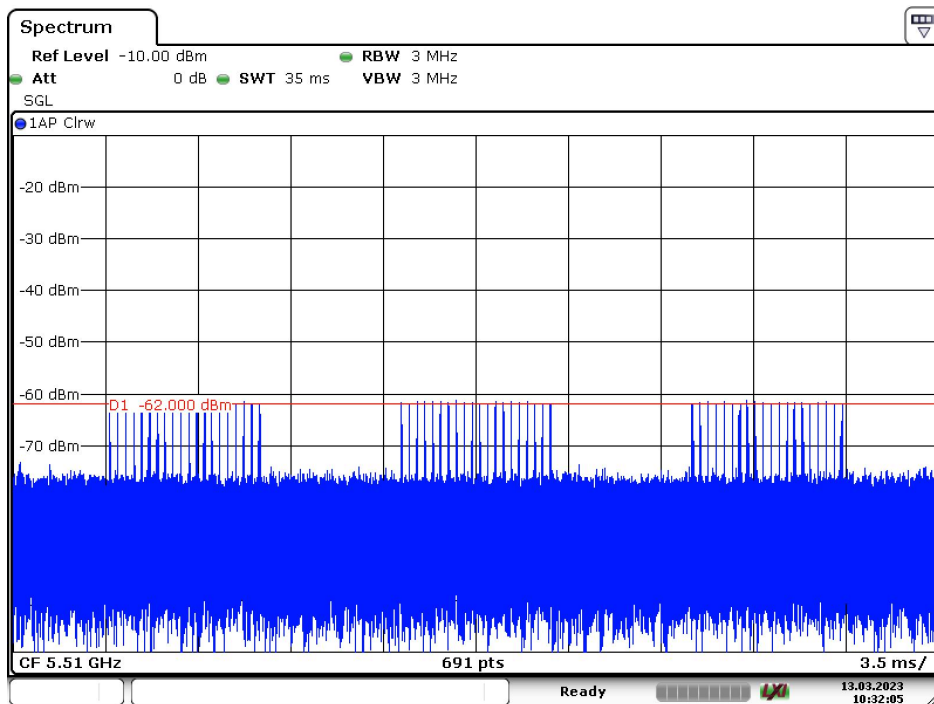
Radar Type 4 – 5510MHz
