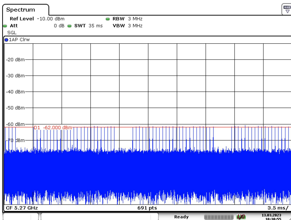
Radar Type 3 – 5270MHz
