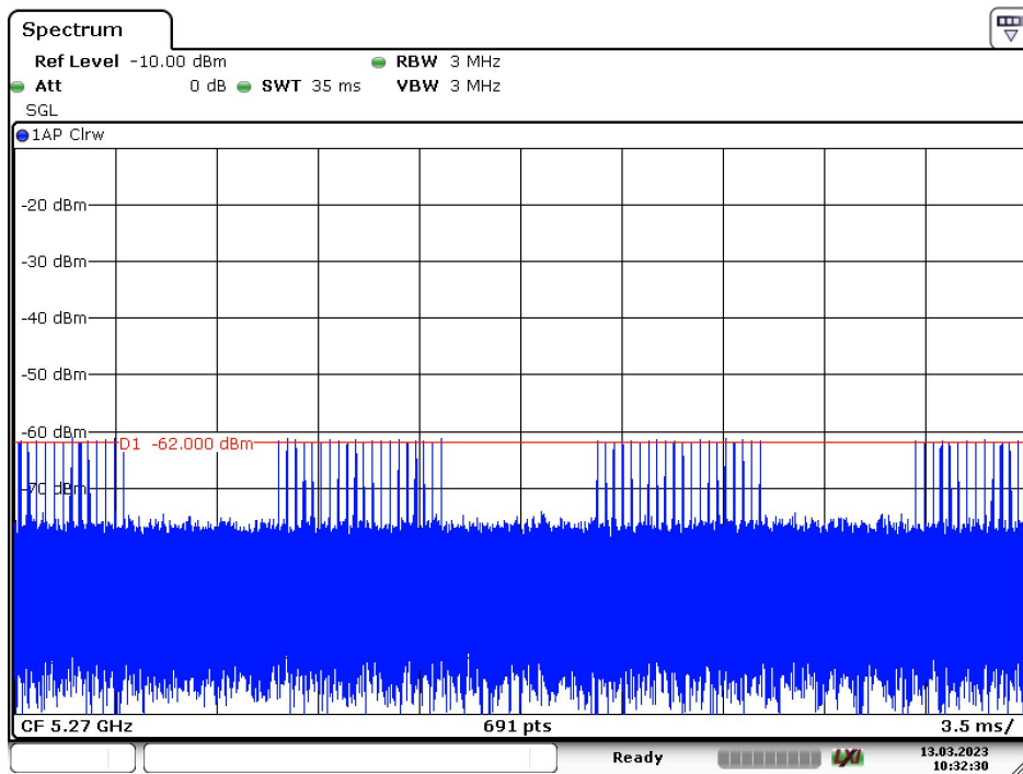
Radar Type 4 – 5270MHz
