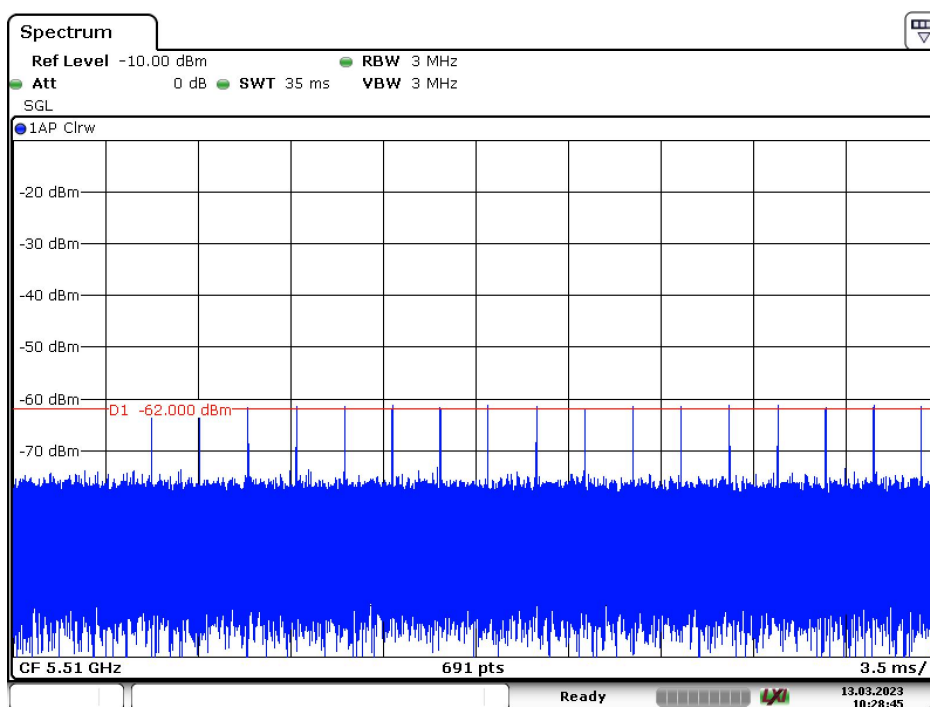
Radar Type 2 – 5510MHz
