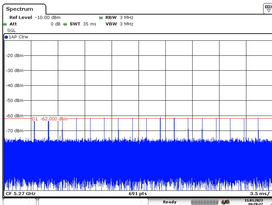
Radar Type 2 – 5270MHz
