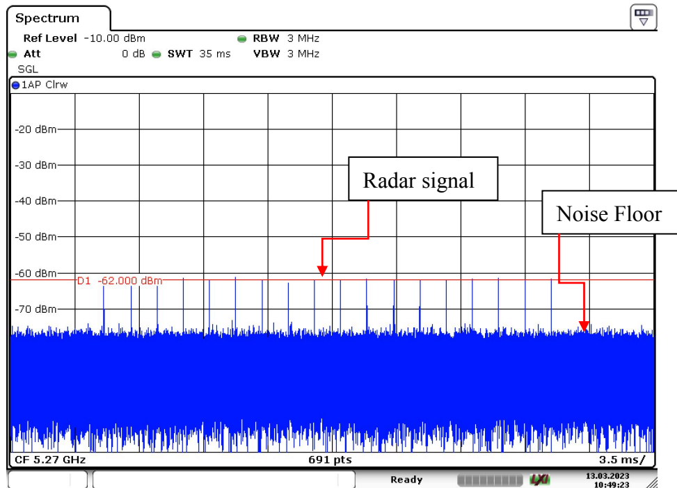
Radar Type 0 – 5270MHz
