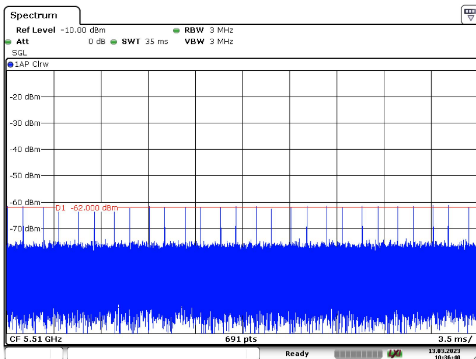
Radar Type 6 – 5510MHz
