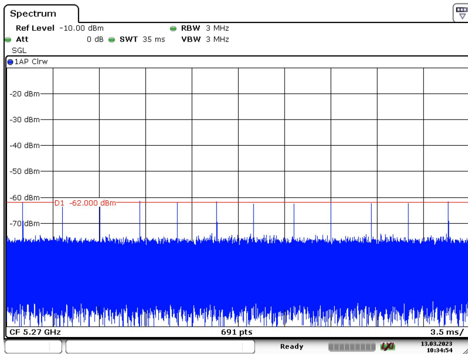
Radar Type 5 – 5270MHz
