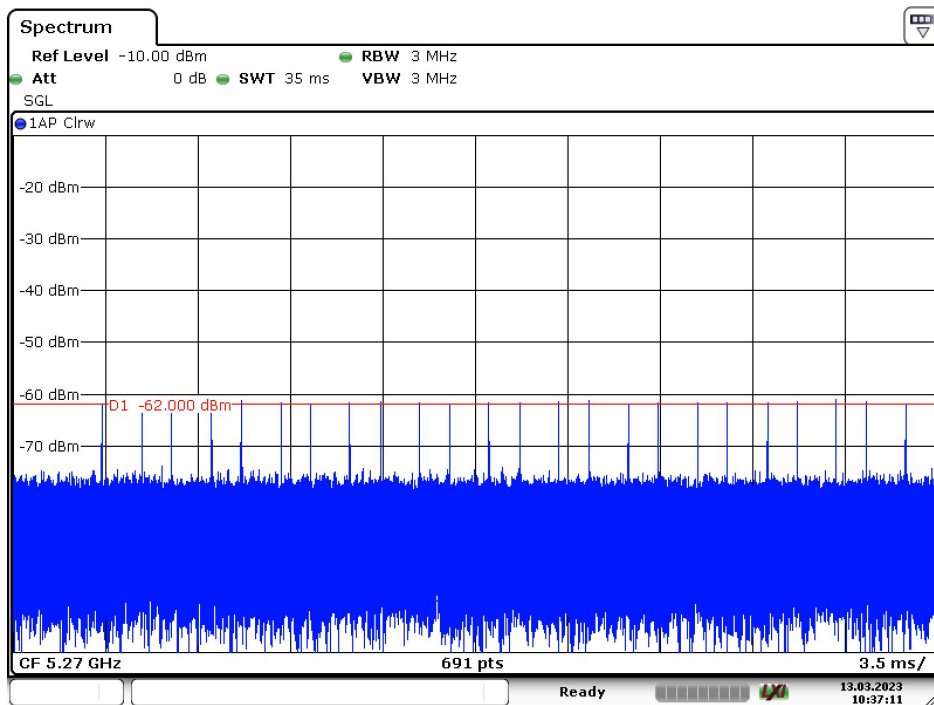
Radar Type 6 – 5270MHz
