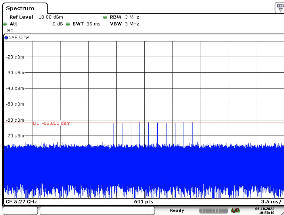
Radar Type 1B – 5270MHz
