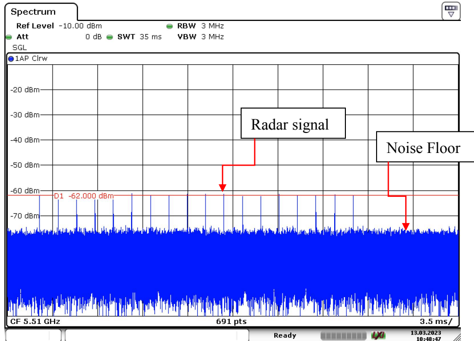
Radar Type 0 – 5510MHz
