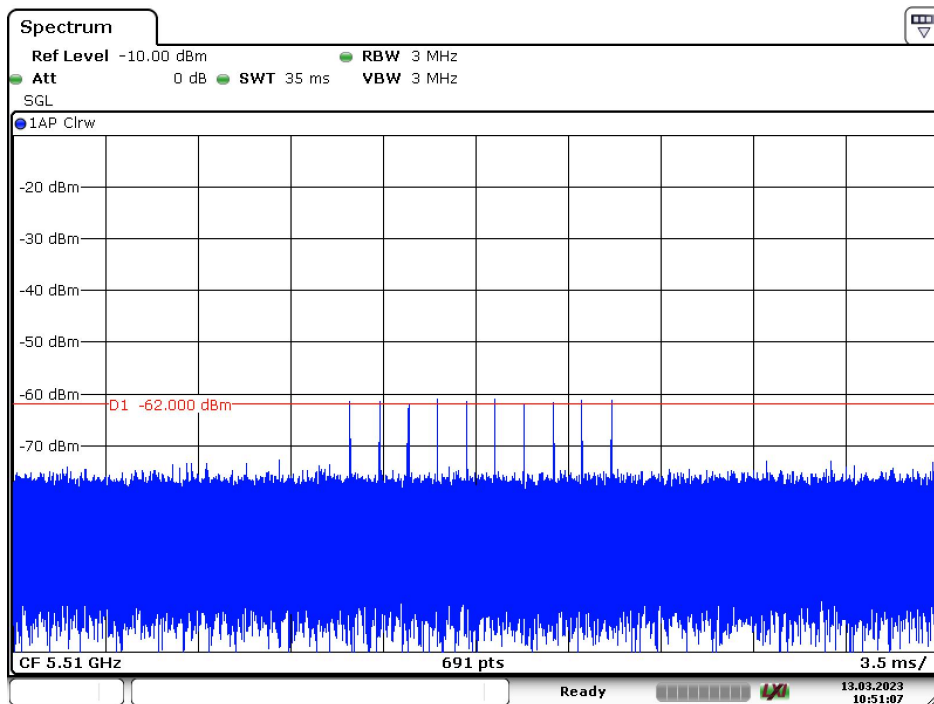
Radar Type 1B – 5510MHz
