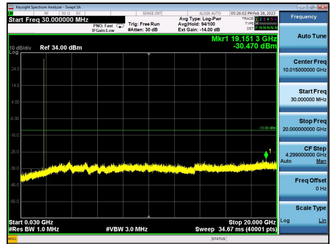
PCS 1900-661, 30MHz ~20GHz
