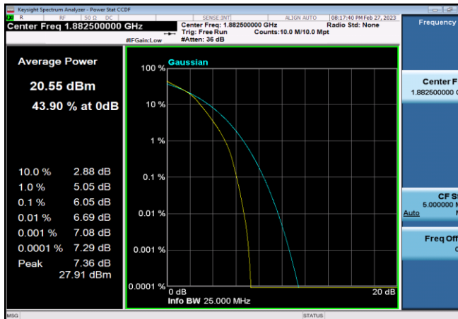
FDD25_MidRange_20MHz_1882.5_fullRB _Q16
