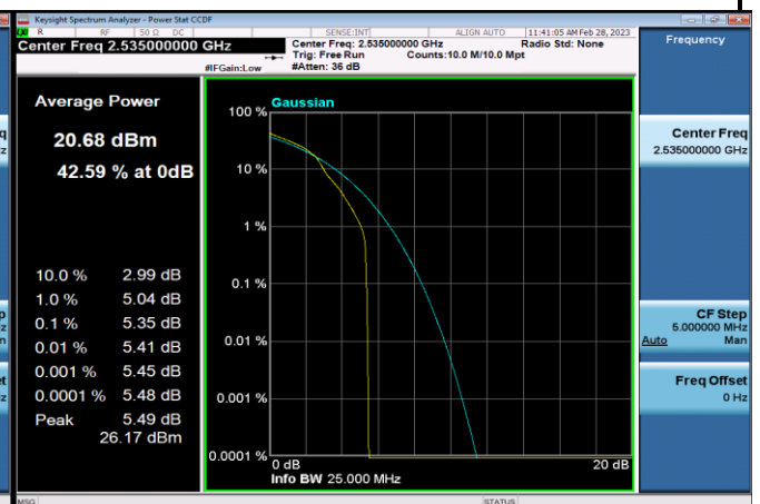
FDD07_MidRange_20MHz_2535_OneRB _high_Q16
