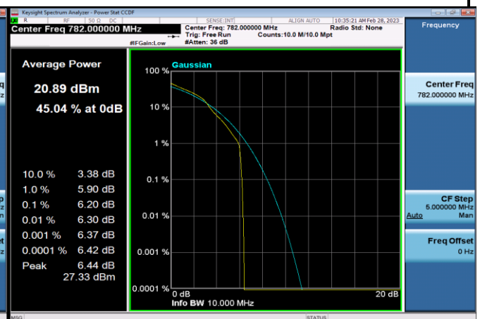
FDD13_MidRange_10MHz_782_OneRB _high_Q16
