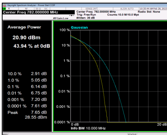
FDD13_MidRange_10MHz_782_fullRB _Q16
