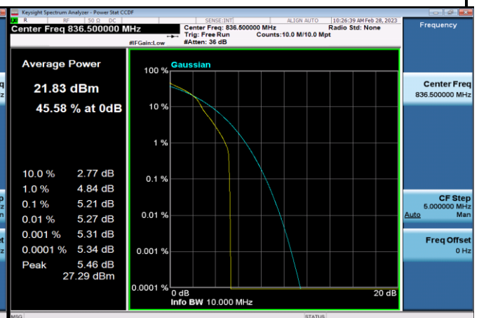
FDD05_MidRange_10MHz_836.5_OneRB _high_Q16
