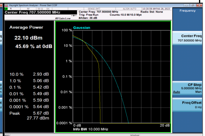
FDD12_MidRange_10MHz_707.5_OneRB _high_Q16
