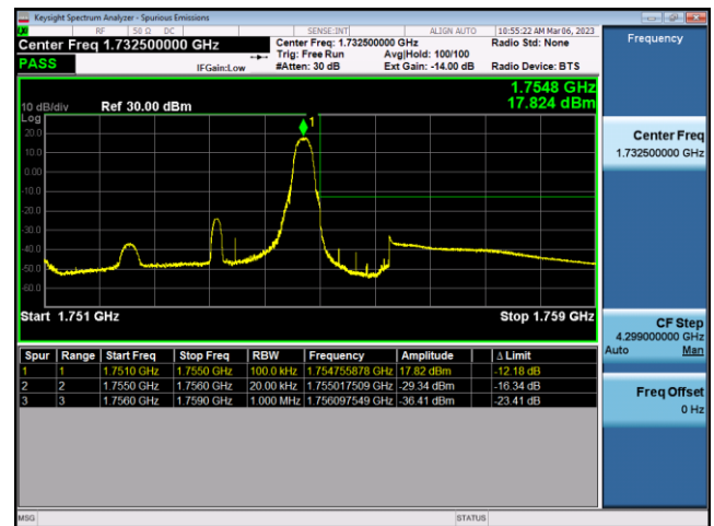
FDD4-3MHz-16QAM-HCH-15RB#0
