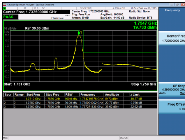
FDD4-3MHz-QPSK-HCH-15RB#0
