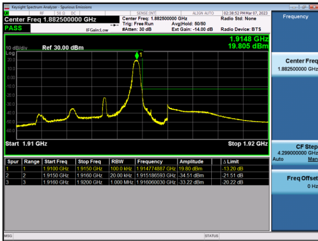
FDD25-3MHz-QPSK-HCH-15RB#0
