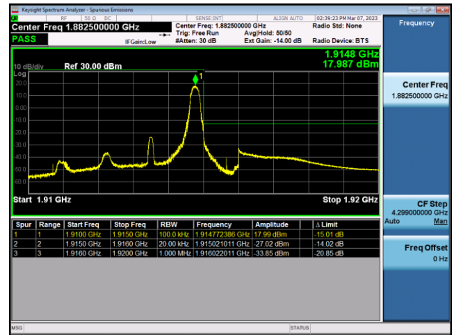
FDD25-3MHz-16QAM-HCH-15RB#0
