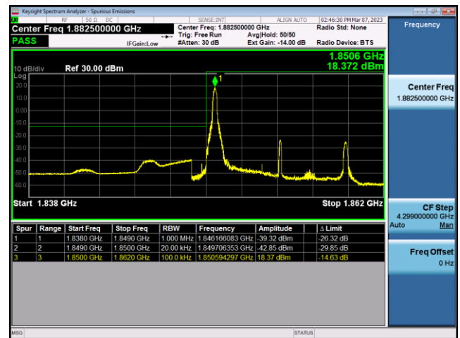
FDD25-10MHz-16QAM-LCH-50RB#0
