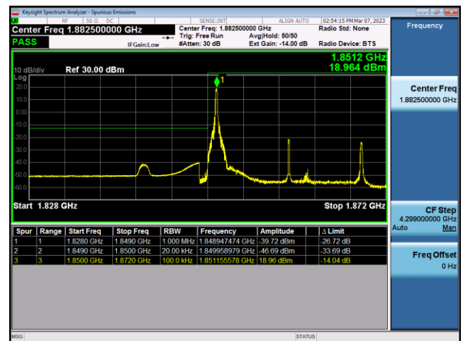
FDD25-20MHz-16QAM-LCH-1RB#0
