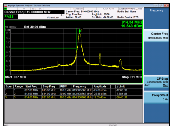
FDD26-Part 90-5MHz-16QAM-LCH-1RB#0
