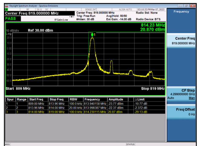
FDD26-Part 90-3MHz-16QAM-LCH-15RB#0
