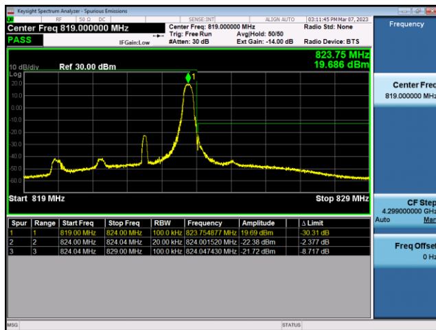
FDD26-Part 90-3MHz-QPSK-HCH-15RB#0
