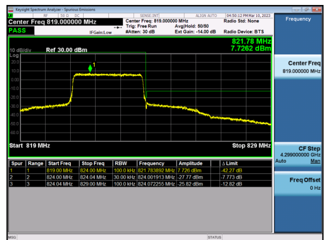
FDD26-Part 90-5MHz-16QAM-LCH-1RB#0
