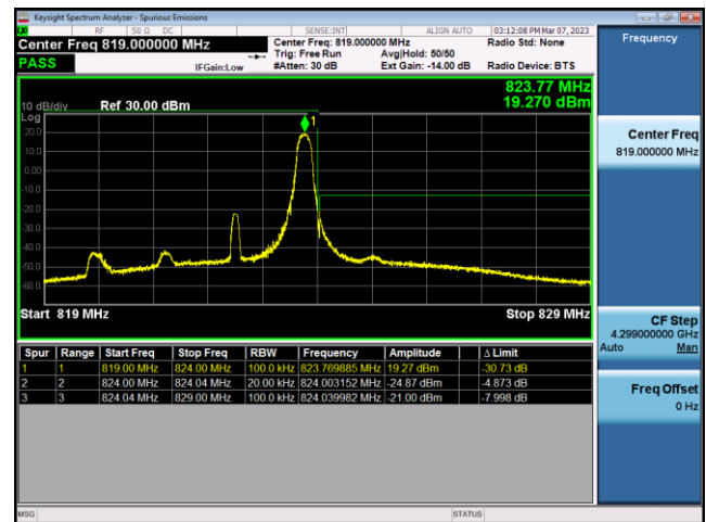
FDD26-Part 90-3MHz-16QAM-HCH-15RB#0
