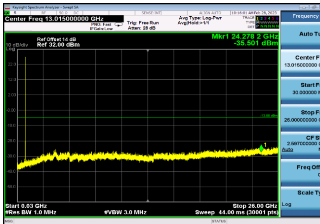
FDD05_LowRange_10MHz_30MHz~26GHz
