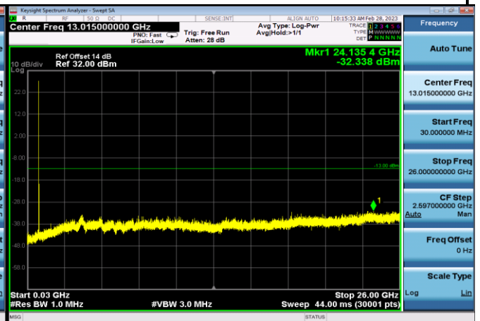
FDD07_HighRange_20MHz_30MHz~26GHz
