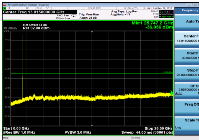
FDD04_LowRange_20MHz_30MHz~26GHz
