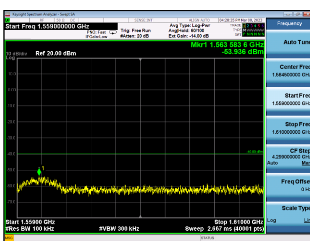
FDD13_MidRange_5MHz_1559MHz~1610MHz
