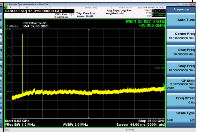
FDD04_HighRange_20MHz_30MHz~26GHz
