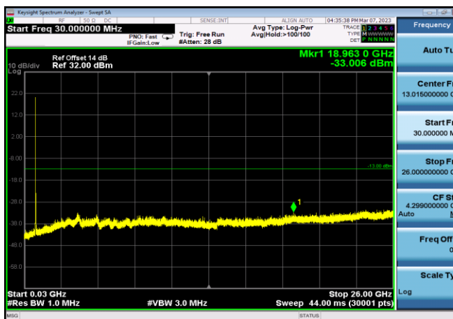
FDD07_LowRange_20MHz_30MHz~26GHz
