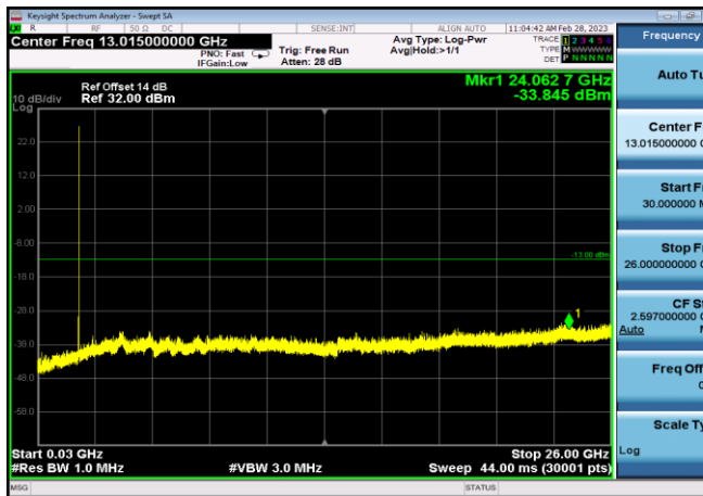
FDD02_MidRange_20MHz_30MHz~26GHz
