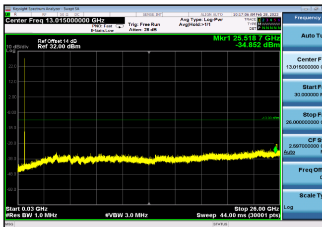
FDD13_MidRange_5MHz_30MHz~26GHz
