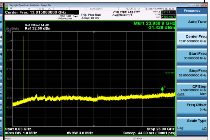
FDD04_MidRange_20MHz_30MHz~26GHz
