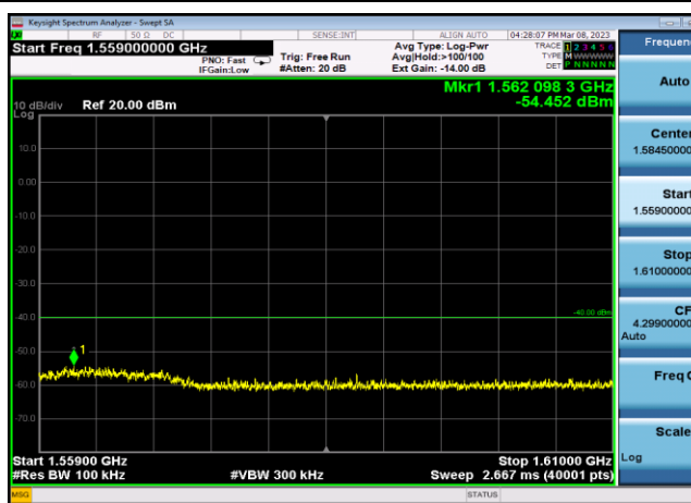
FDD13_MidRange_10MHz_1559MHz~1610MHz
