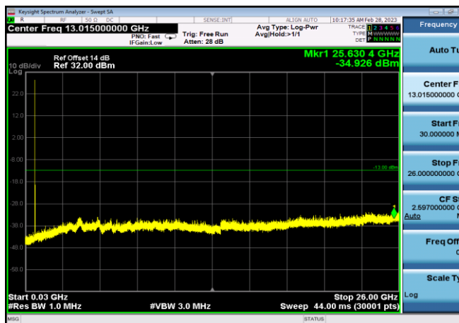
FDD12_MidRange_10MHz_30MHz~26GHz
