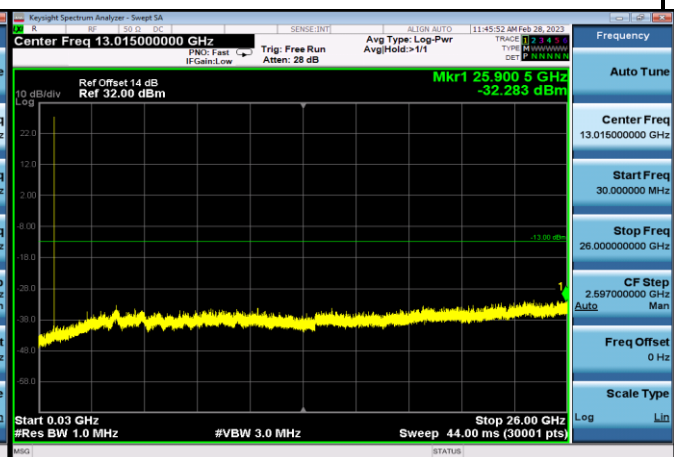
FDD13_LowRange_5MHz_30MHz~26GHz
