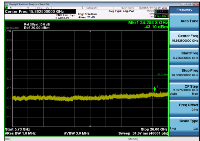
U-NII-2c ,Plot 3,5725MHz~26000MHz-802 .11a(20MHz),5600MHz,Ant1
