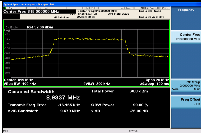
Band26-10MHz-QPSK-26740-50RB#0-8.9337
