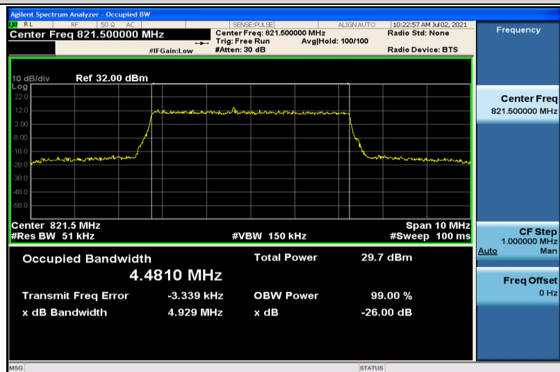
Band26-5MHz-16QAM-26765-25RB#0-4.4810
