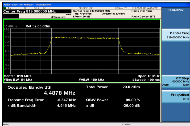
Band26-5MHz-16QAM-26740-25RB#0-4.4878
