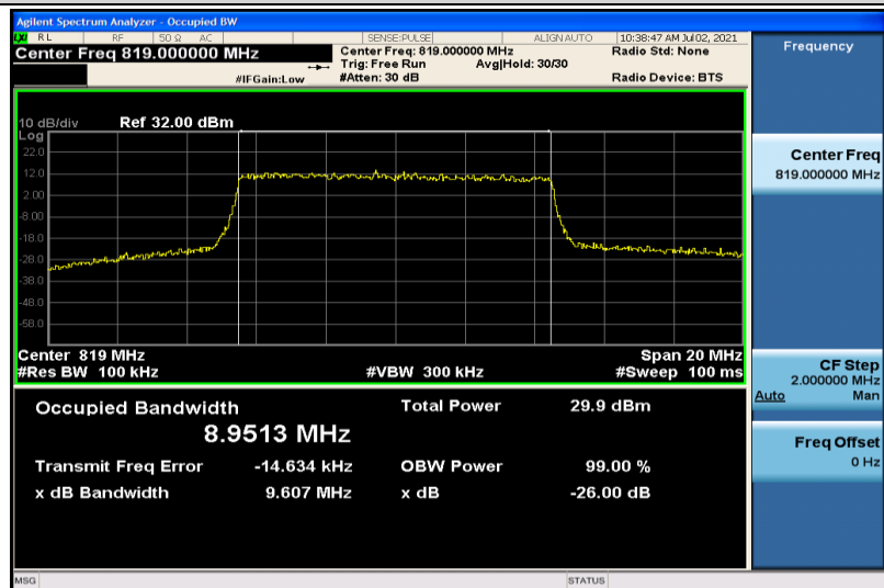
Band26-10MHz-16QAM-26740-50RB#0-8.9513
