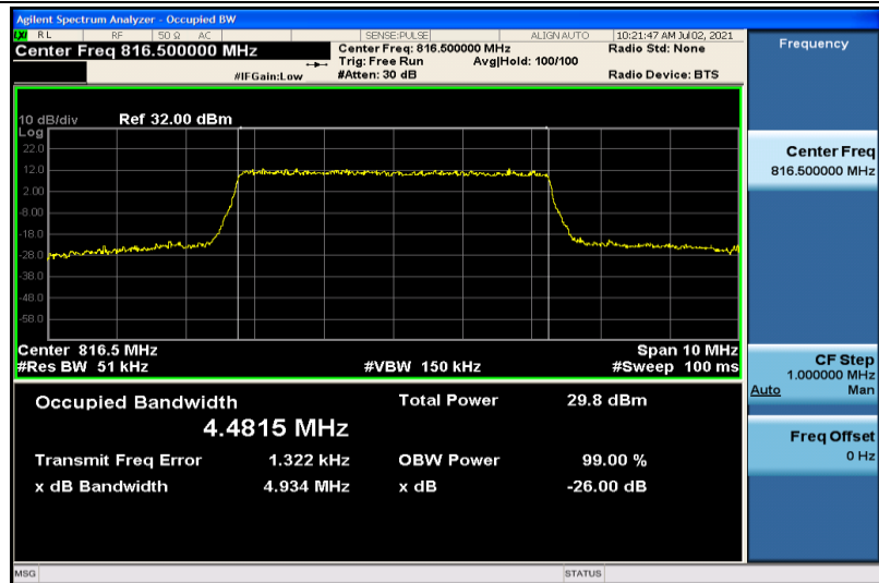
Band26-5MHz-16QAM-26715-25RB#0-4.4815
