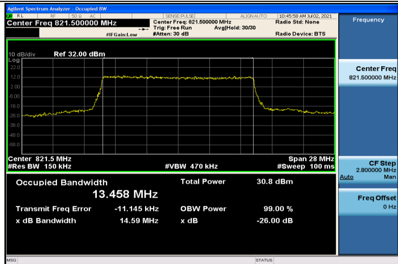
Band26-15MHz-QPSK-26765-75RB#0-13.458
