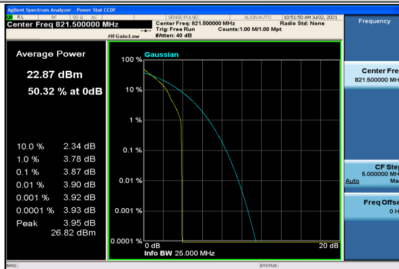
Band26-15MHz-QPSK-26765-1RB#0
