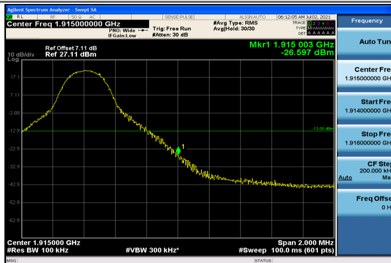
Band25-10MHz-QPSK-26640-1RB#49
