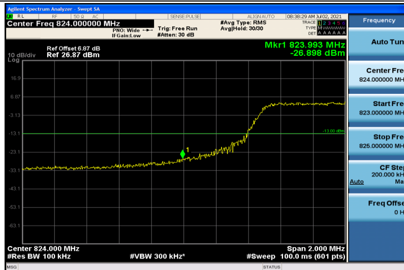
Band26-10MHz-QPSK-26840-50RB#0
