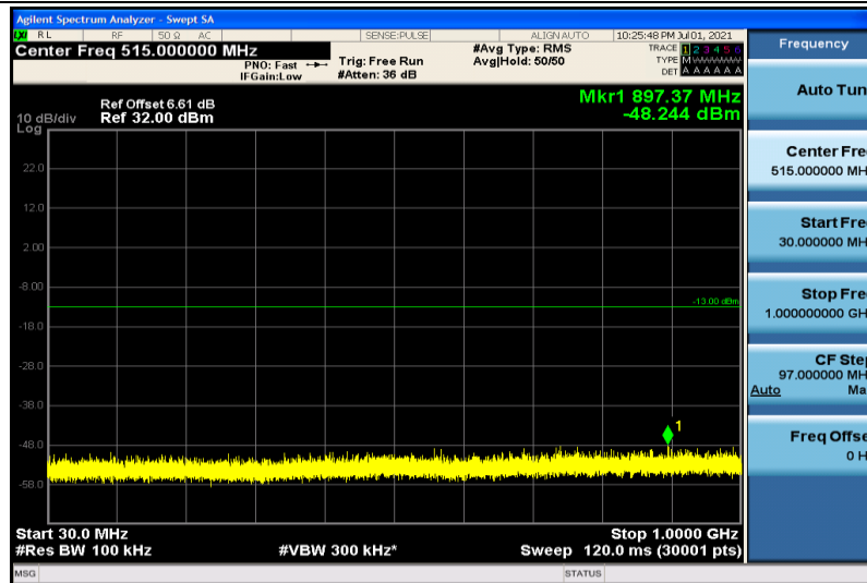
Band2-15MHz-QPSK-18675-1RB#0-30~1000MHz
