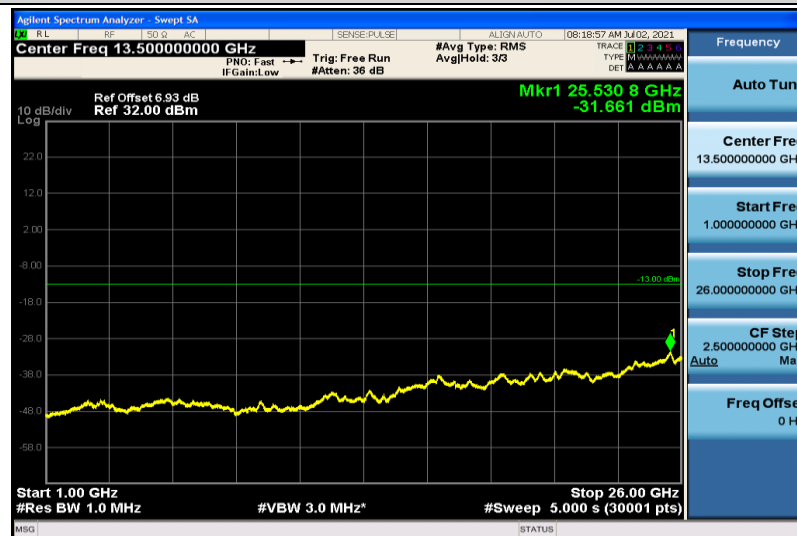
Band26-5MHz-QPSK-26915-1RB#0-1000~26000MHz
