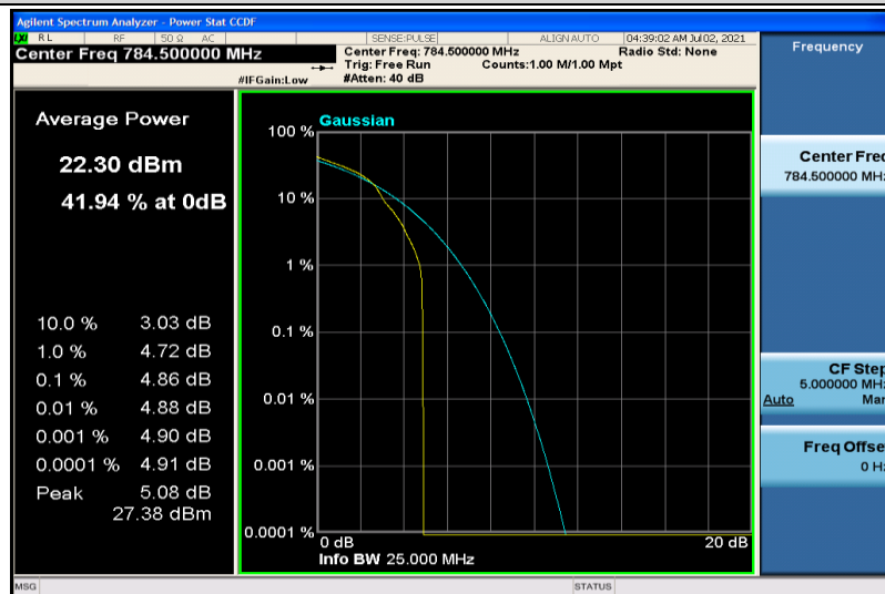
Band13-5MHz-16QAM-23255-1RB#0
