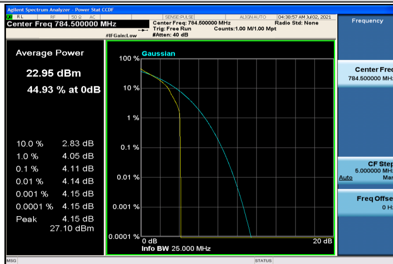
Band13-5MHz-QPSK-23255-1RB#0
