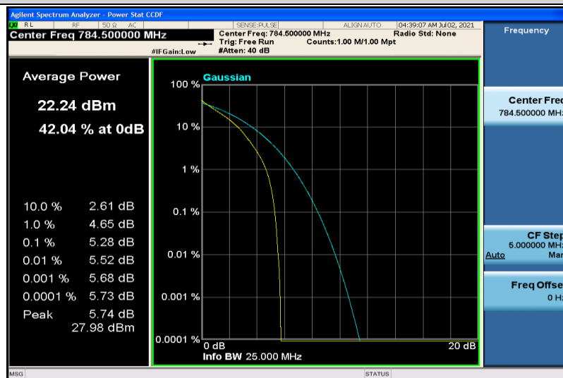
Band13-5MHz-QPSK-23255-25RB#0
