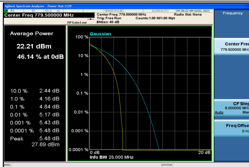
Band13-5MHz-QPSK-23205-25RB#0
