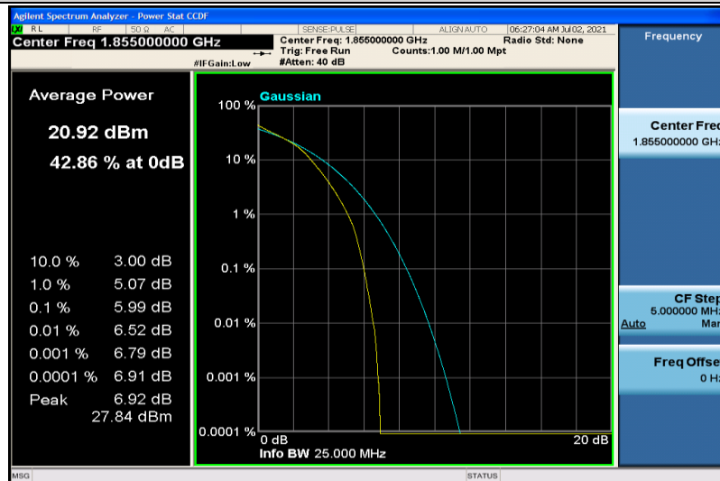
Band25-10MHz-16QAM-26090-50RB#0
