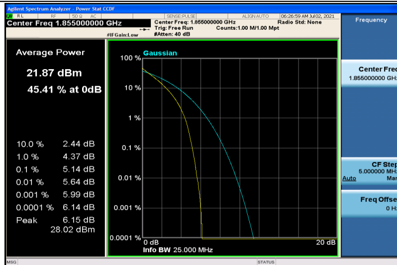
Band25-10MHz-QPSK-26090-50RB#0
