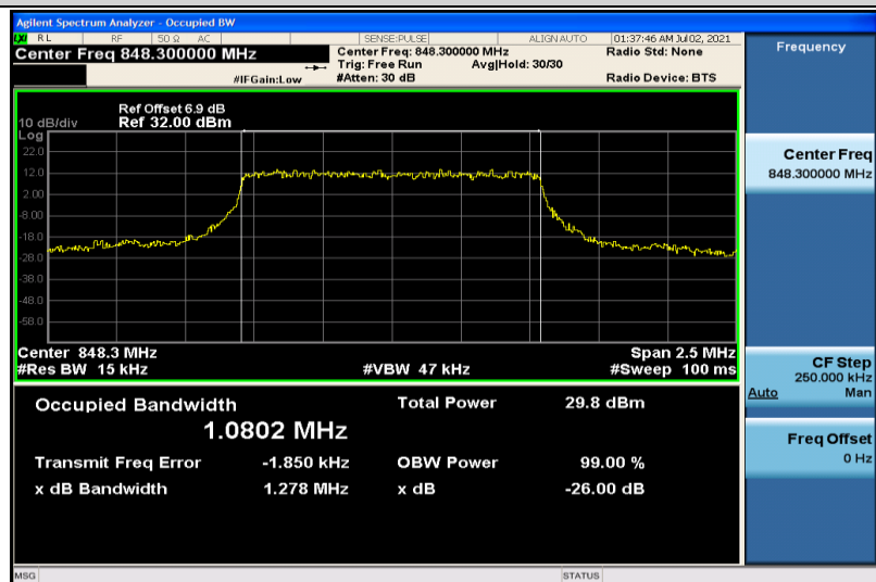
Band5-1.4MHz-QPSK-20643-6RB#0-1.0802
