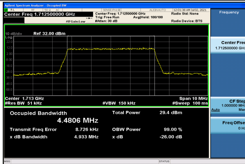
Band4-5MHz-16QAM-19975-25RB#0-4.4806
