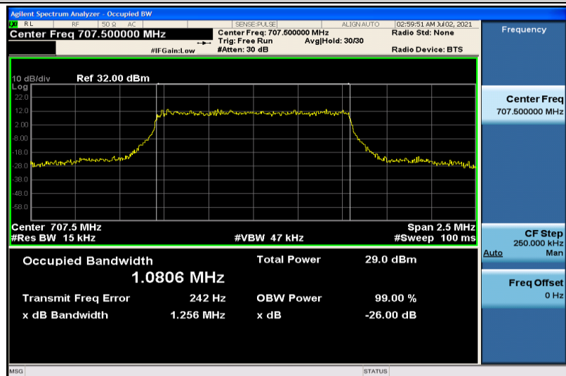
Band12-1.4MHz-16QAM-23095-6RB#0-1.0806
