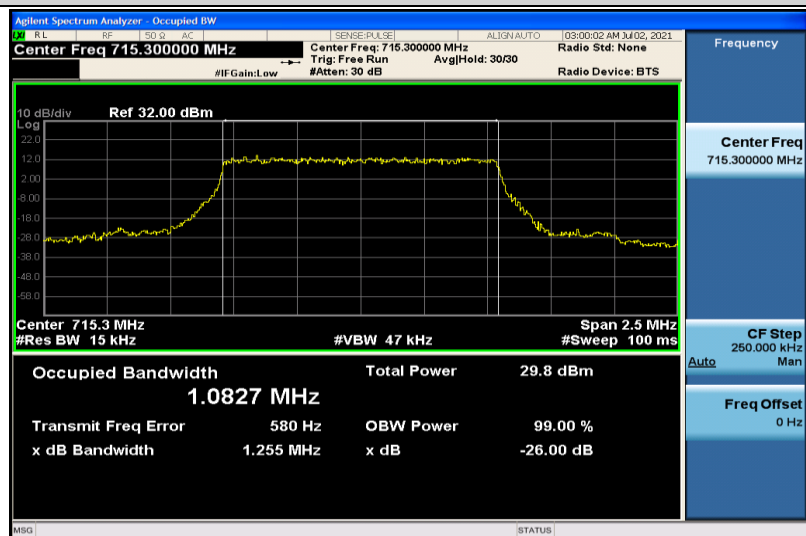
Band12-1.4MHz-QPSK-23173-6RB#0-1.0827
