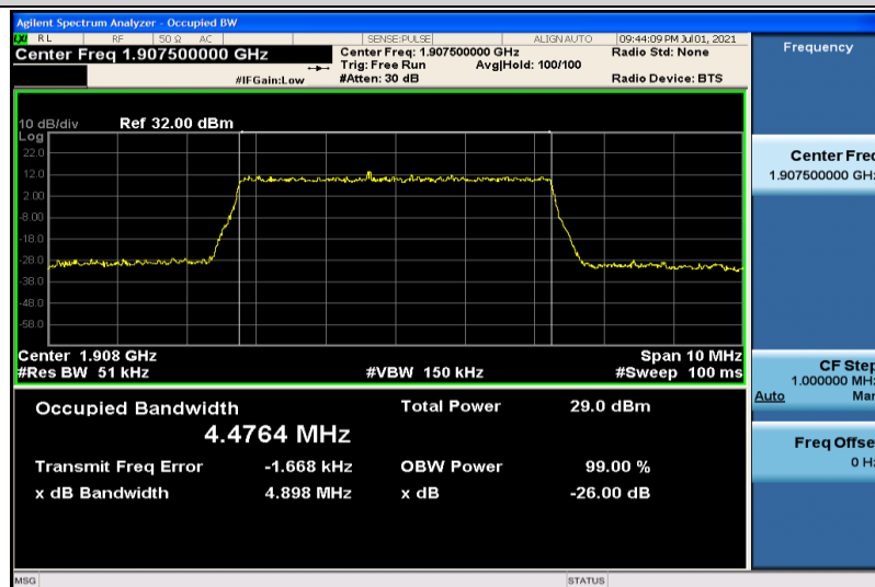
Band2-5MHz-16QAM-19175-25RB#0-4.4764
