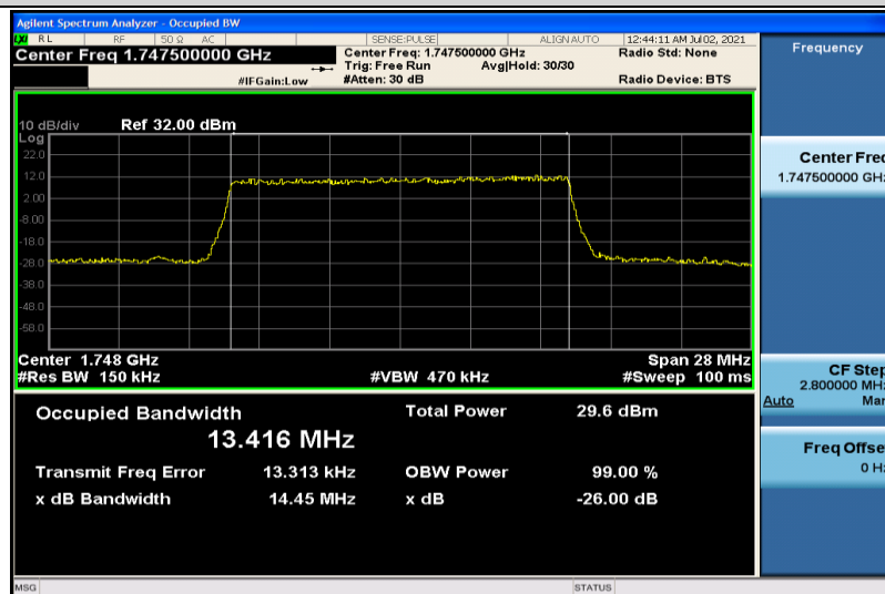
Band4-15MHz-16QAM-20325-75RB#0-13.416
