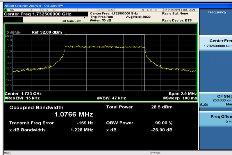
Band4-1.4MHz-16QAM-20175-6RB#0-1.0766
