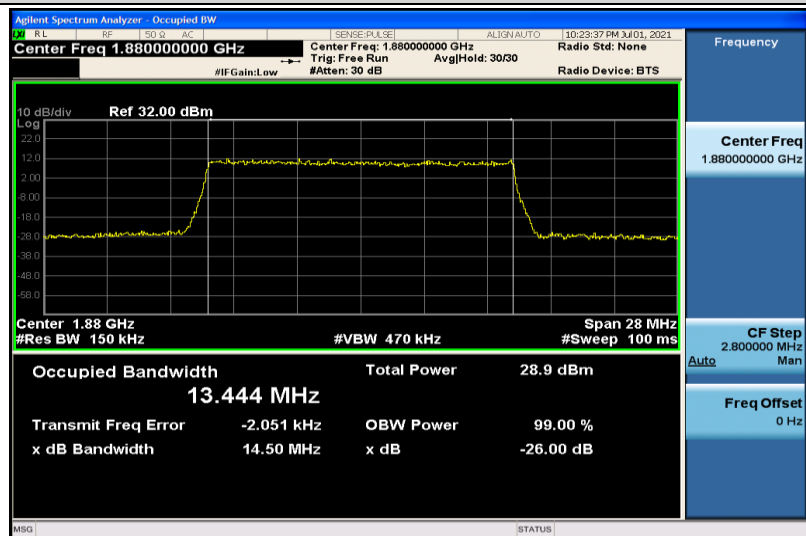
Band2-15MHz-16QAM-18900-75RB#0-13.444
