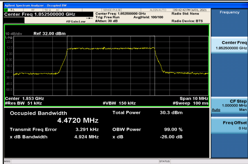
Band2-5MHz-QPSK-18625-25RB#0-4.4720
