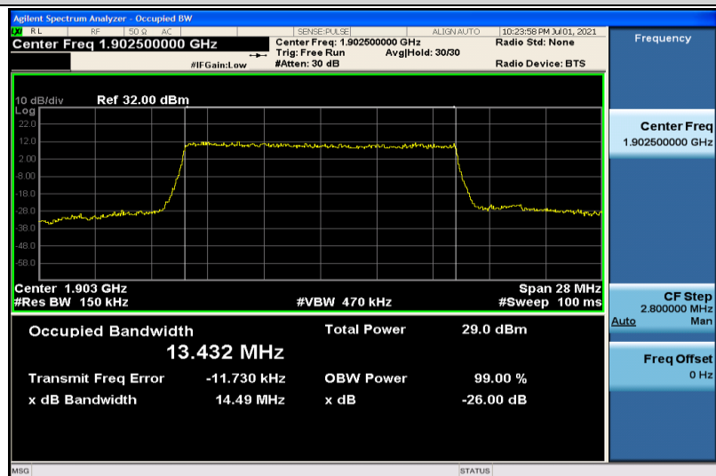
Band2-15MHz-16QAM-19125-75RB#0-13.432
