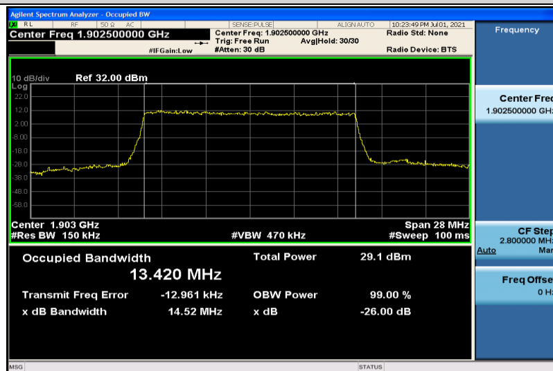
Band2-15MHz-QPSK-19125-75RB#0-13.420
