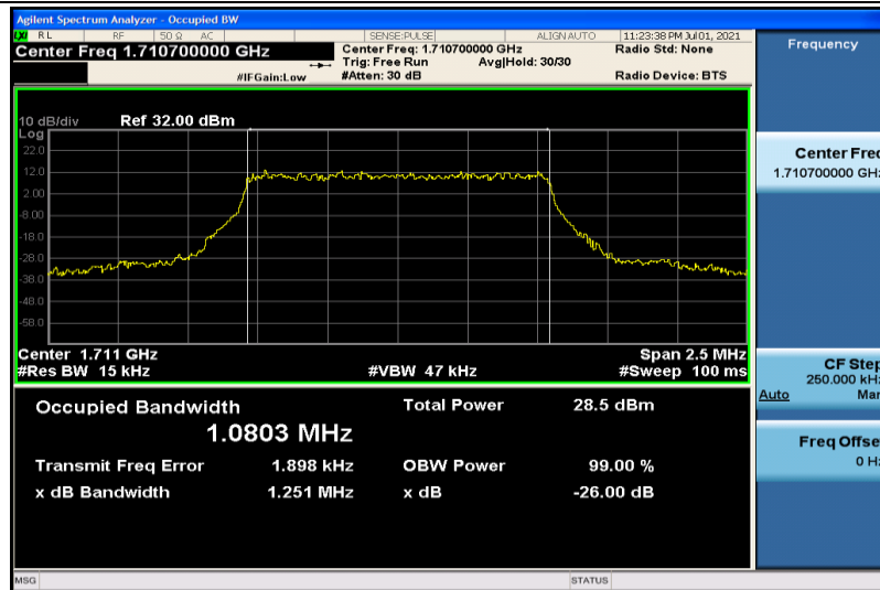
Band4-1.4MHz-16QAM-19957-6RB#0-1.0803
