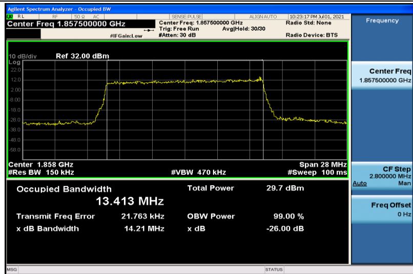
Band2-15MHz-16QAM-18675-75RB#0-13.413
