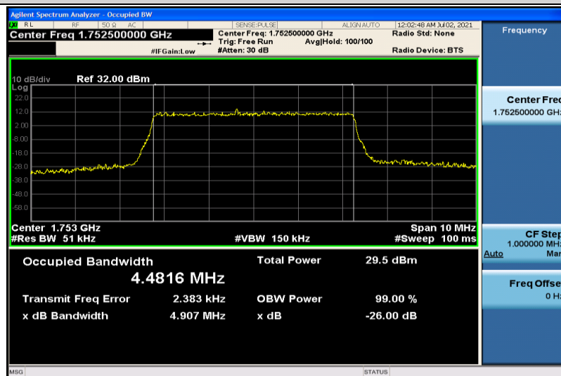
Band4-5MHz-16QAM-20375-25RB#0-4.4816
