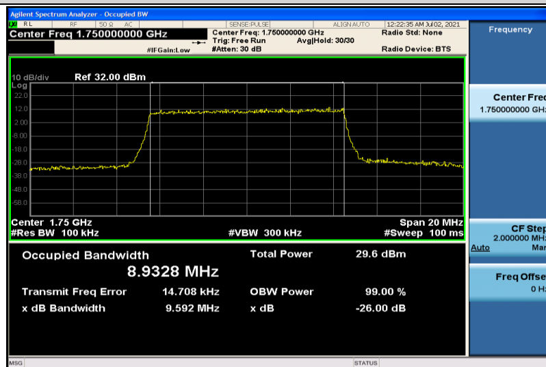
Band4-10MHz-16QAM-20350-50RB#0-8.9328
