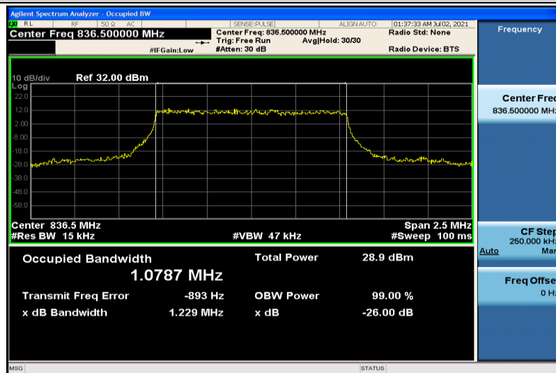
Band5-1.4MHz-16QAM-20525-6RB#0-1.0787
