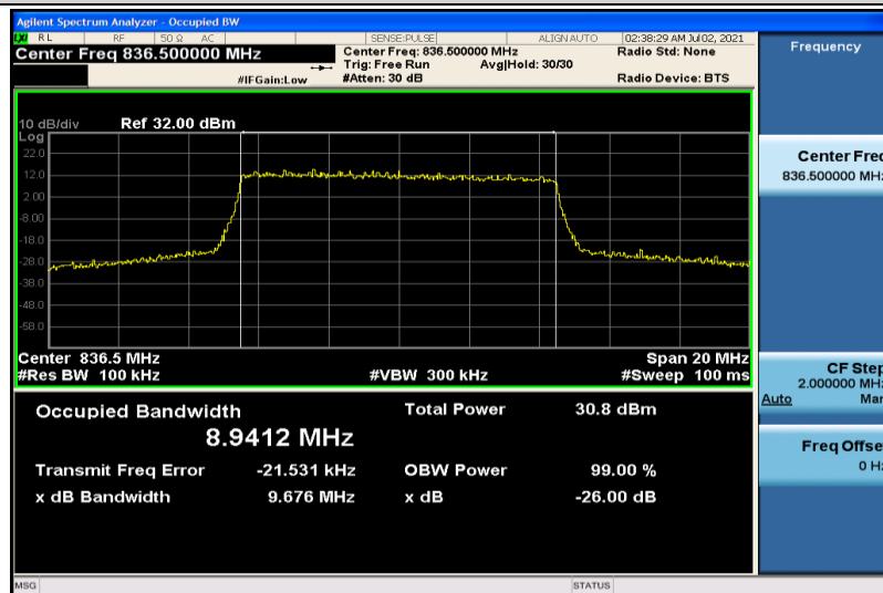
Band5-10MHz-QPSK-20525-50RB#0-8.9412
