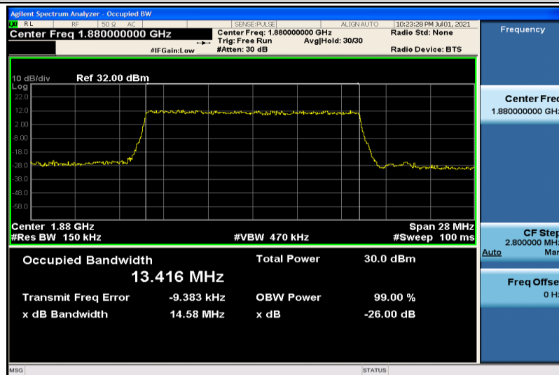
Band2-15MHz-QPSK-18900-75RB#0-13.416
