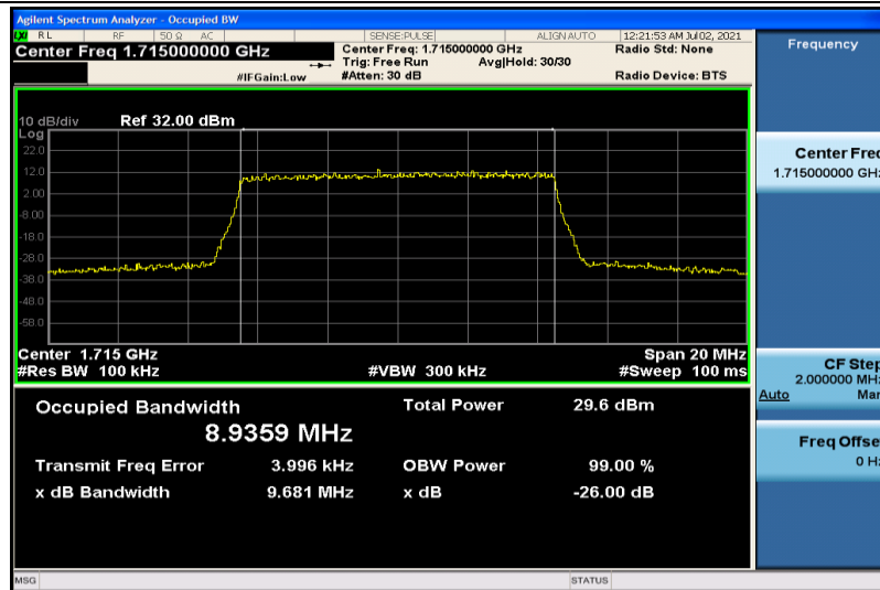
Band4-10MHz-16QAM-20000-50RB#0-8.9359
