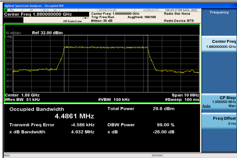
Band2-5MHz-QPSK-18900-25RB#0-4.4861
