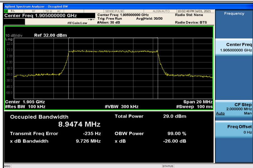
Band2-10MHz-16QAM-19150-50RB#0-8.9474
