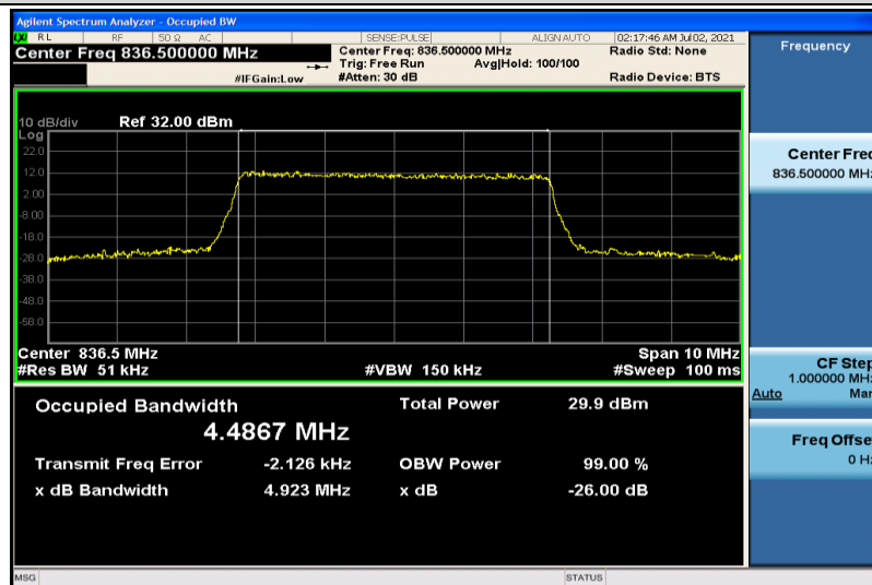
Band5-5MHz-16QAM-20525-25RB#0-4.4867
