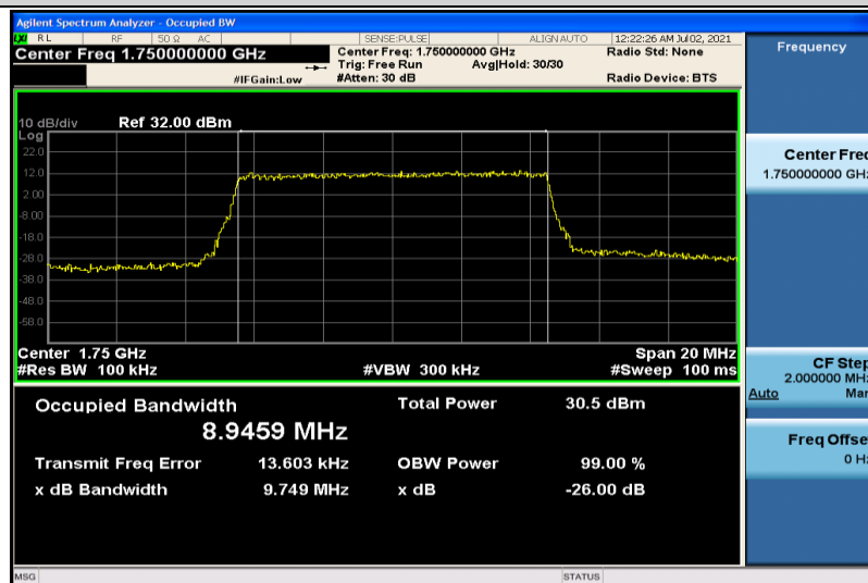
Band4-10MHz-QPSK-20350-50RB#0-8.9459
