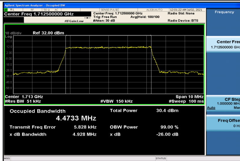
Band4-5MHz-QPSK-19975-25RB#0-4.4733
