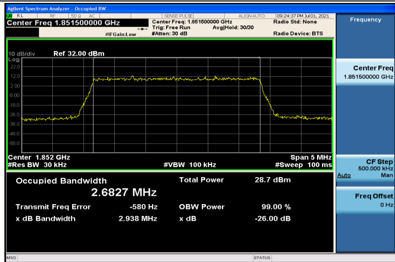
Band2-3MHz-16QAM-18615-15RB#0-2.6827
