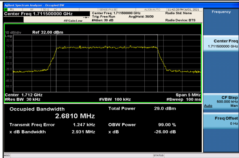
Band4-3MHz-16QAM-19965-15RB#0-2.6810
