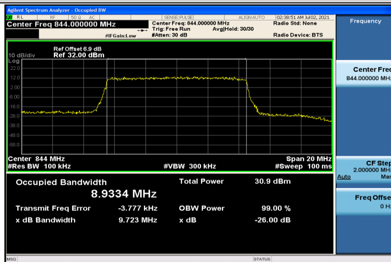
Band5-10MHz-QPSK-20600-50RB#0-8.9334
