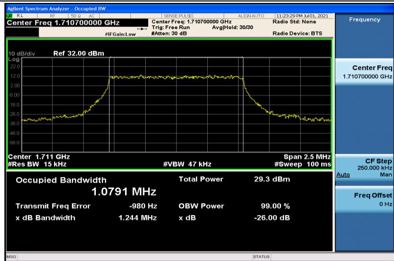
Band4-1.4MHz-QPSK-19957-6RB#0-1.0791
