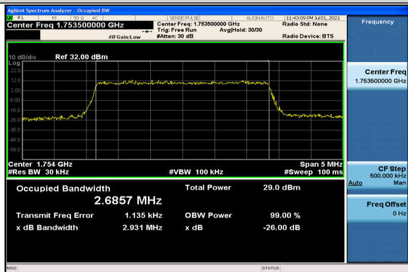
Band4-3MHz-16QAM-20385-15RB#0-2.6857
