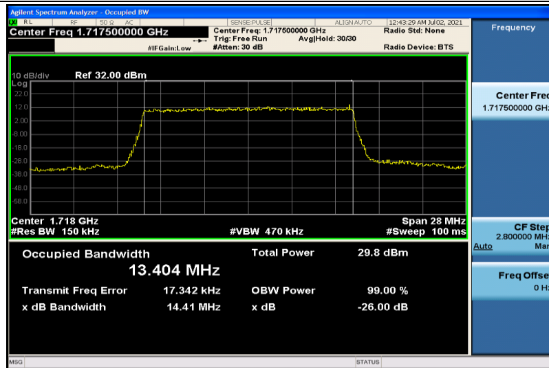
Band4-15MHz-16QAM-20025-75RB#0-13.404
