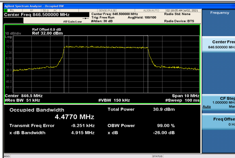
Band5-5MHz-QPSK-20625-25RB#0-4.4770
