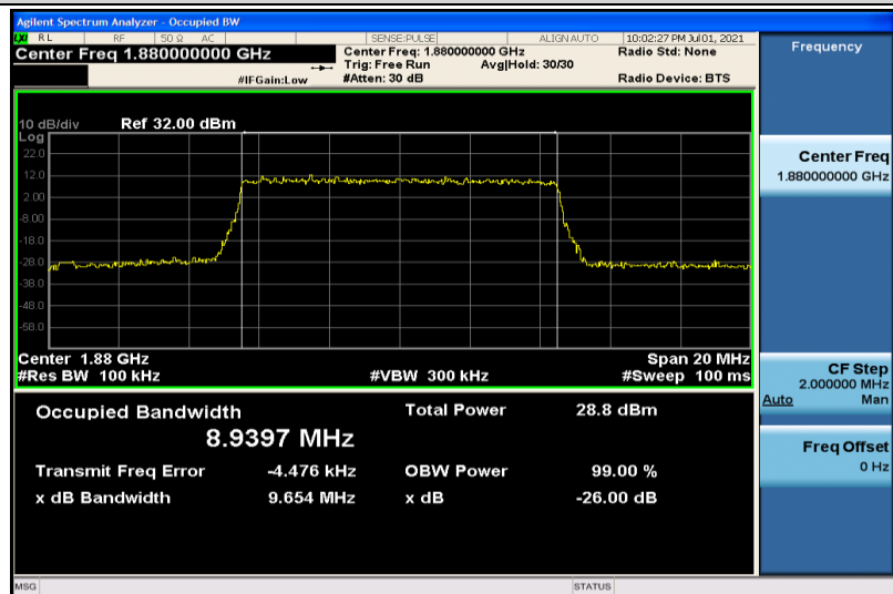
Band2-10MHz-16QAM-18900-50RB#0-8.9397
