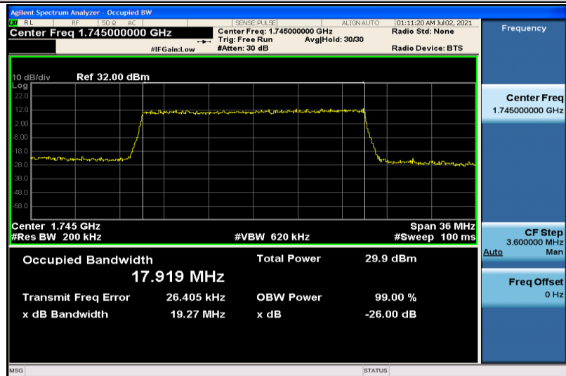
Band4-20MHz-16QAM-20300-100RB#0-17.919
