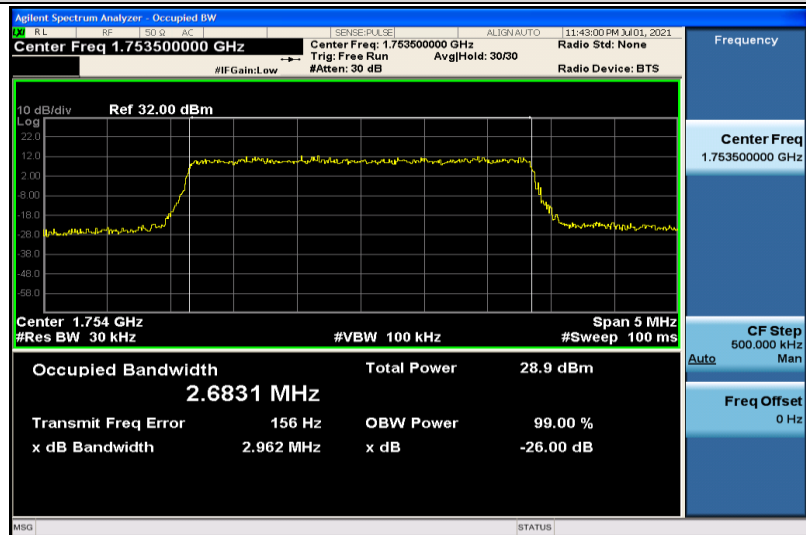
Band4-3MHz-QPSK-20385-15RB#0-2.6831
