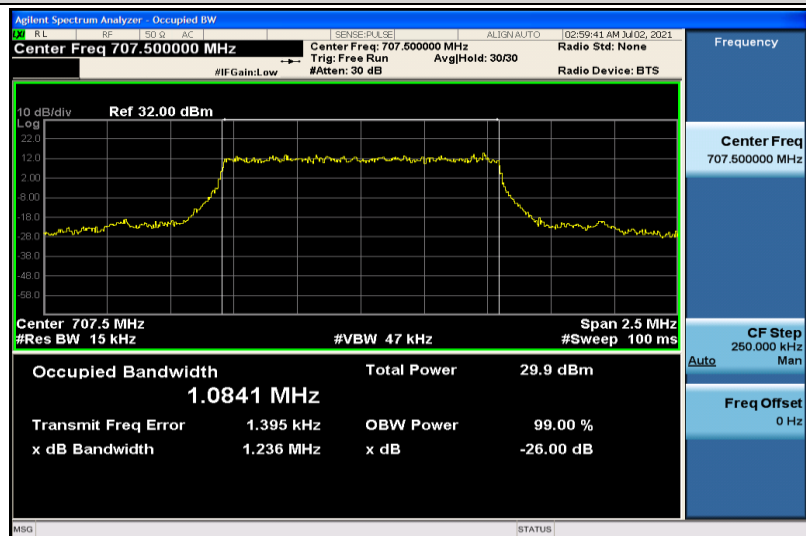
Band12-1.4MHz-QPSK-23095-6RB#0-1.0841
