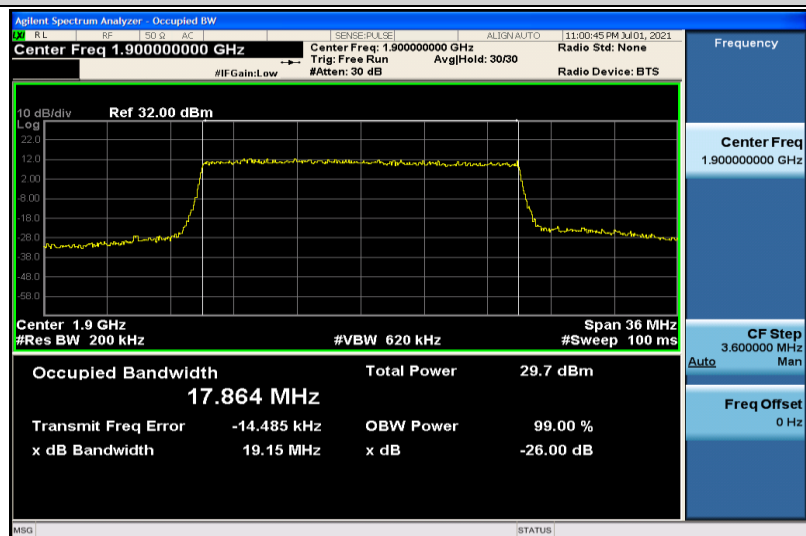
Band2-20MHz-16QAM-19100-100RB#0-17.864
