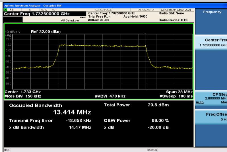
Band4-15MHz-16QAM-20175-75RB#0-13.414
