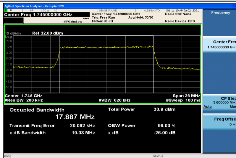
Band4-20MHz-QPSK-20300-100RB#0-17.887
