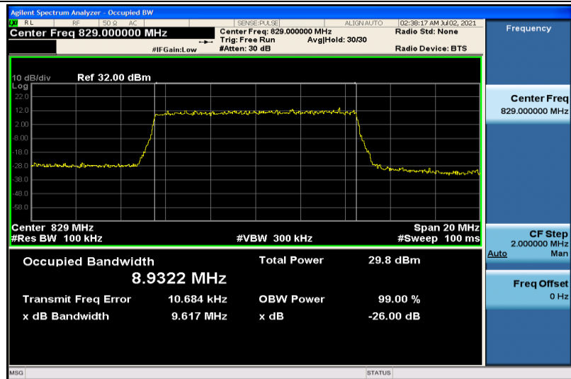
Band5-10MHz-16QAM-20450-50RB#0-8.9322
