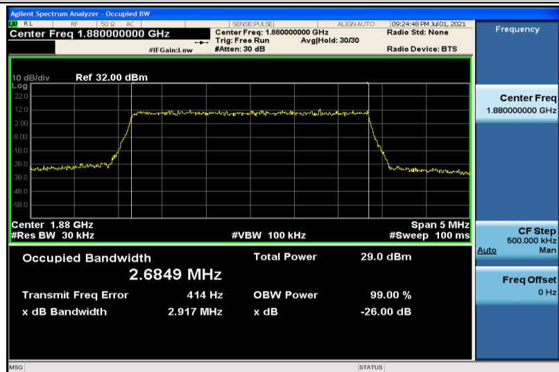
Band2-3MHz-QPSK-18900-15RB#0-2.6849
