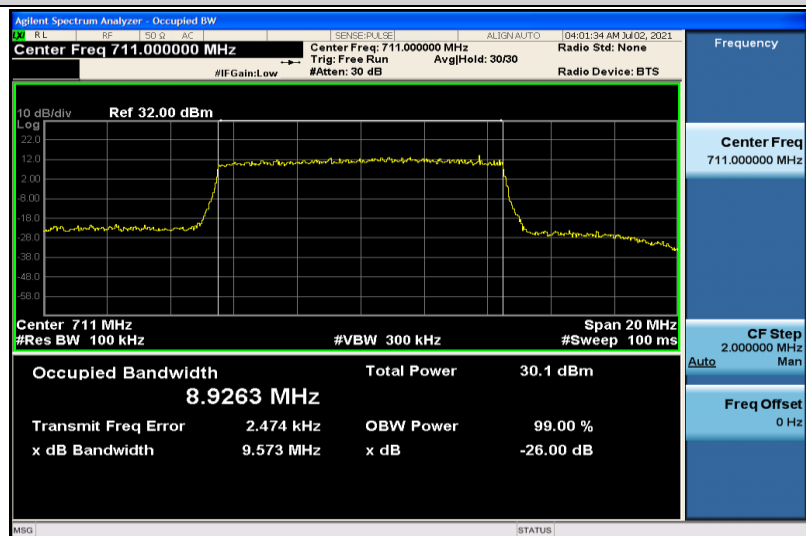
Band12-10MHz-16QAM-23130-50RB#0-8.9263
