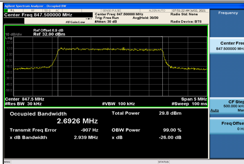
Band26-3MHz-QPSK-27025-15RB#0-2.6926
