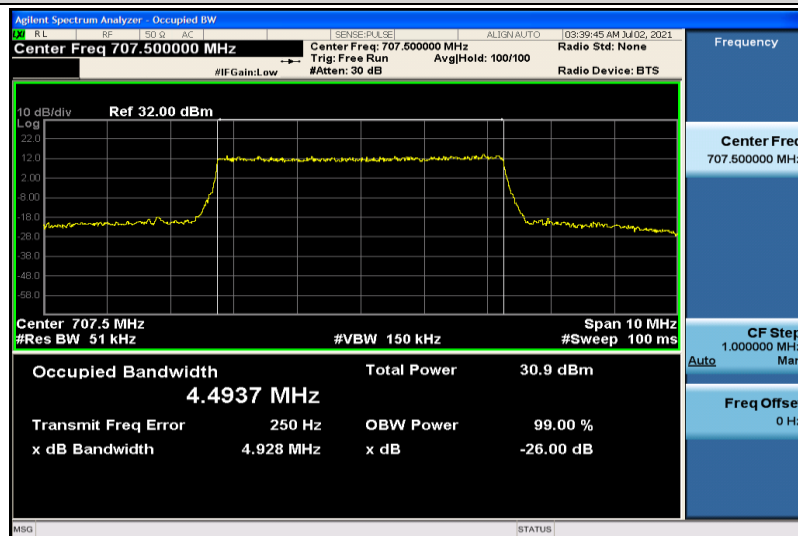
Band12-5MHz-QPSK-23095-25RB#0-4.4937
