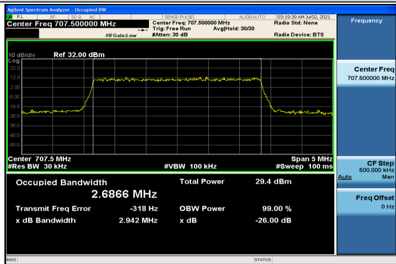
Band12-3MHz-16QAM-23095-15RB#0-2.6866
