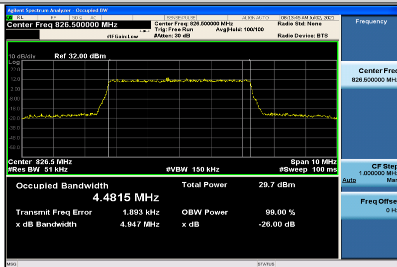
Band26-5MHz-16QAM-26815-25RB#0-4.4815
