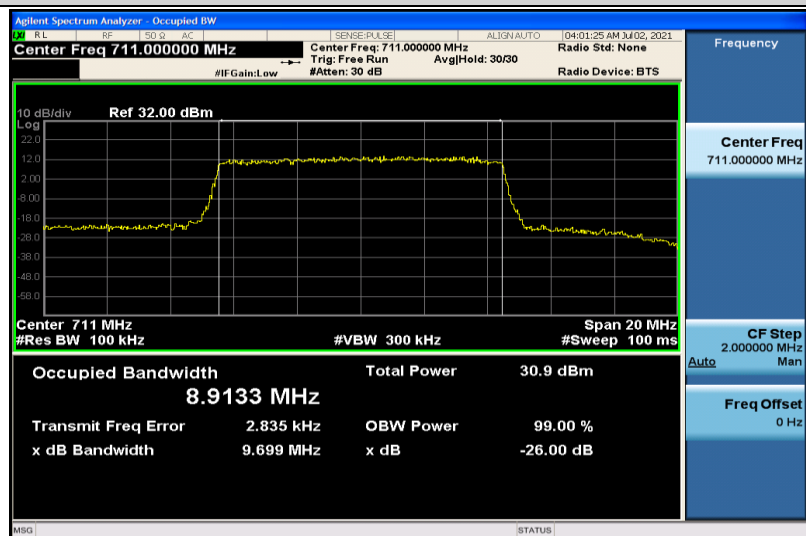
Band12-10MHz-QPSK-23130-50RB#0-8.9133
