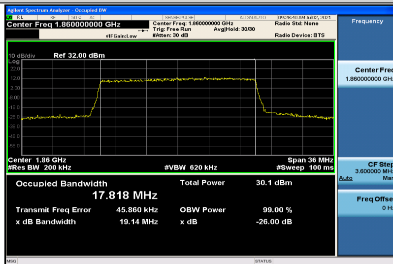
Band25-20MHz-16QAM-26140-100RB#0-17.818
