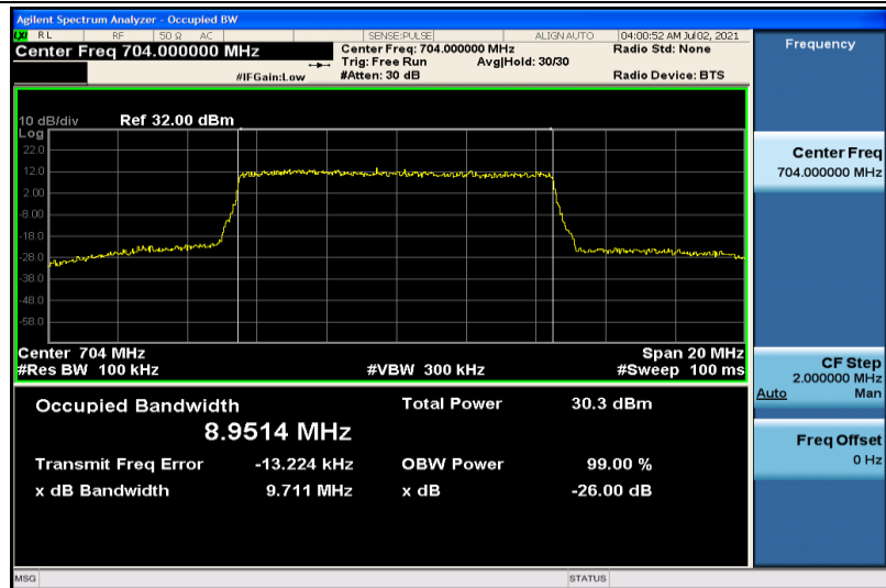
Band12-10MHz-16QAM-23060-50RB#0-8.9514
