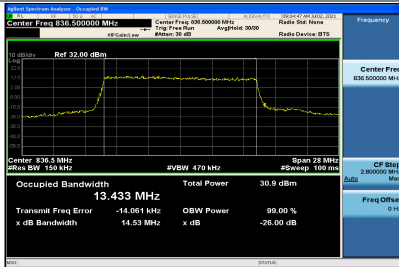
Band26-15MHz-QPSK-26915-75RB#0-13.433
