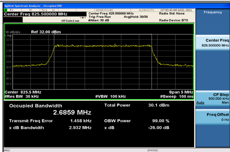
Band26-3MHz-QPSK-26805-15RB#0-2.6859
