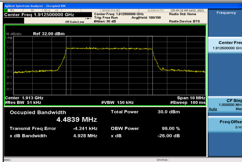
Band25-5MHz-QPSK-26665-25RB#0-4.4839
