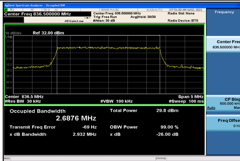
Band26-3MHz-QPSK-26915-15RB#0-2.6876
