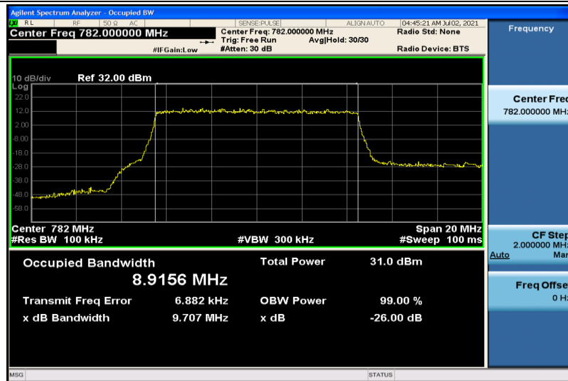
Band13-10MHz-QPSK-23230-50RB#0-8.9156
