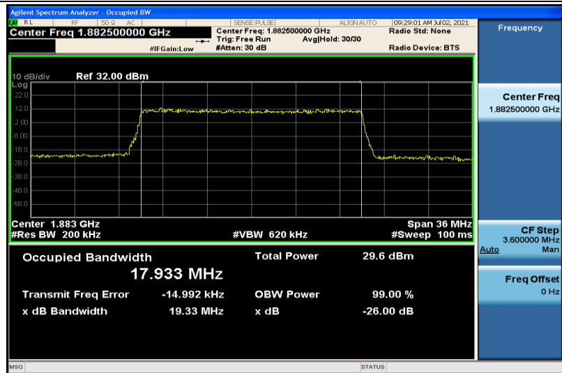
Band25-20MHz-16QAM-26365-100RB#0-17.933
