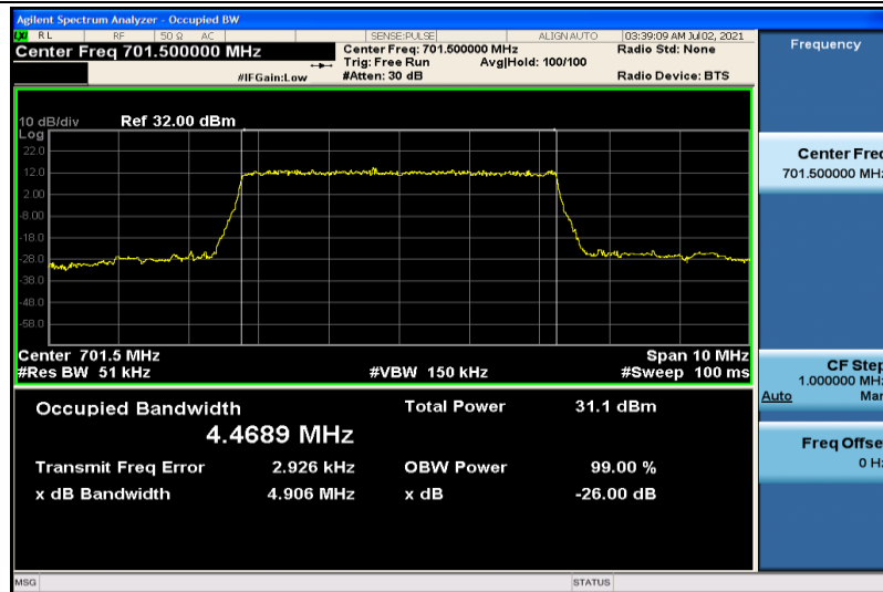
Band12-5MHz-QPSK-23035-25RB#0-4.4689
