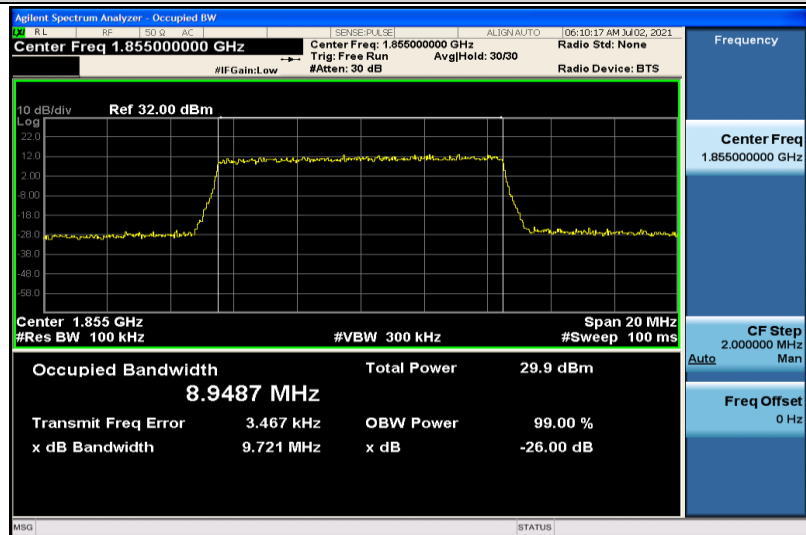
Band25-10MHz-16QAM-26090-50RB#0-8.9487
