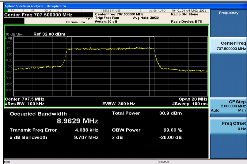
Band12-10MHz-QPSK-23095-50RB#0-8.9629
