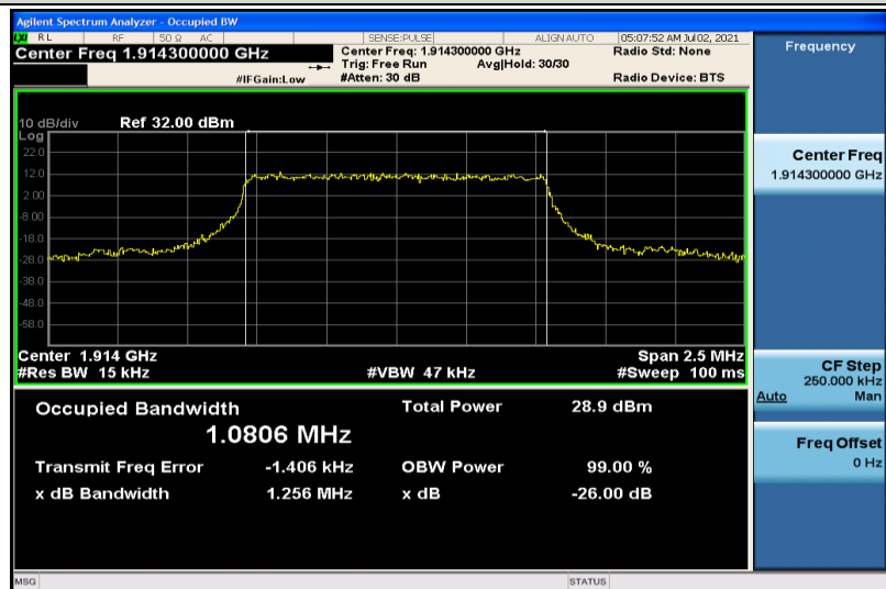
Band25-1.4MHz-QPSK-26683-6RB#0-1.0806
