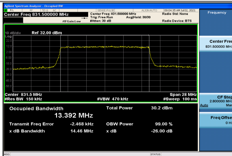
Band26-15MHz-16QAM-26865-75RB#0-13.392
