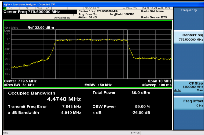
Band13-5MHz-16QAM-23205-25RB#0-4.4740
