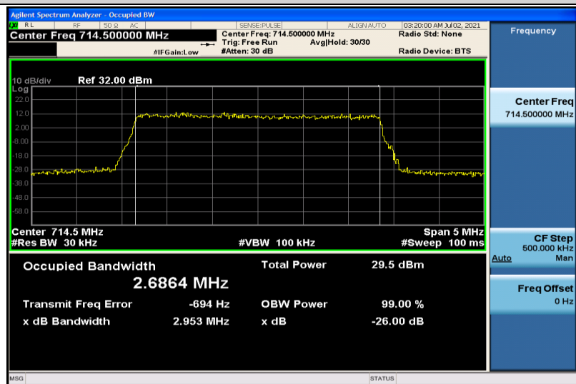
Band12-3MHz-16QAM-23165-15RB#0-2.6864
