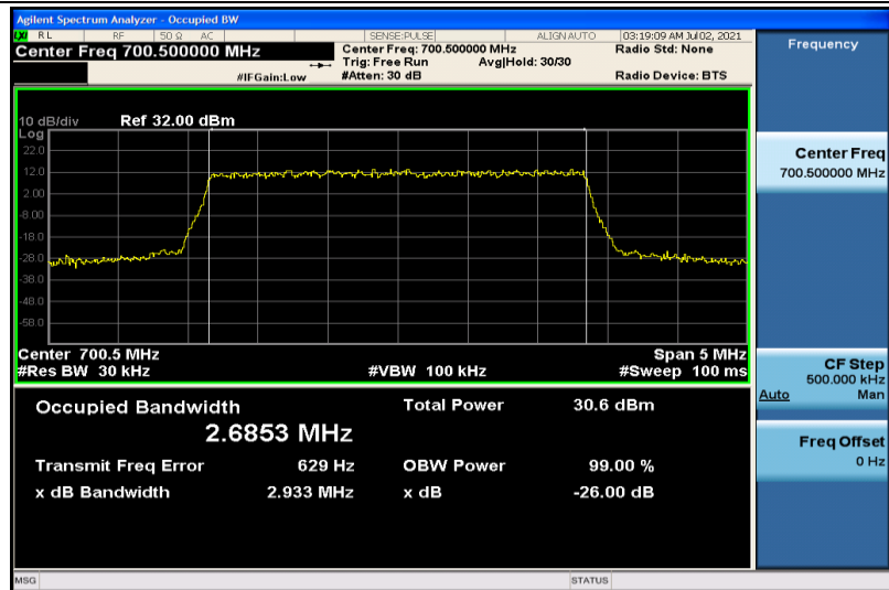
Band12-3MHz-QPSK-23025-15RB#0-2.6853
