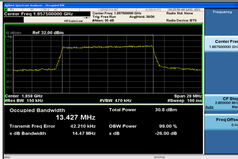
Band25-15MHz-QPSK-26115-75RB#0-13.427
