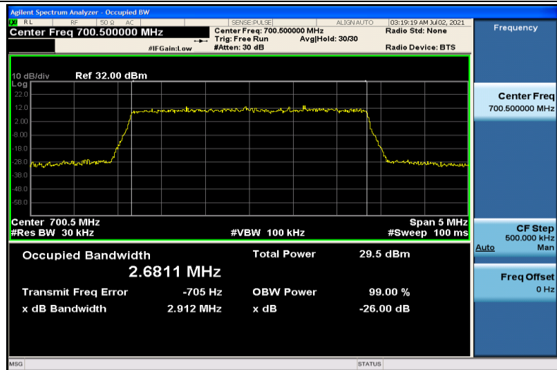
Band12-3MHz-16QAM-23025-15RB#0-2.6811
