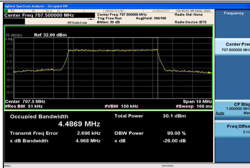
Band12-5MHz-16QAM-23095-25RB#0-4.4869
