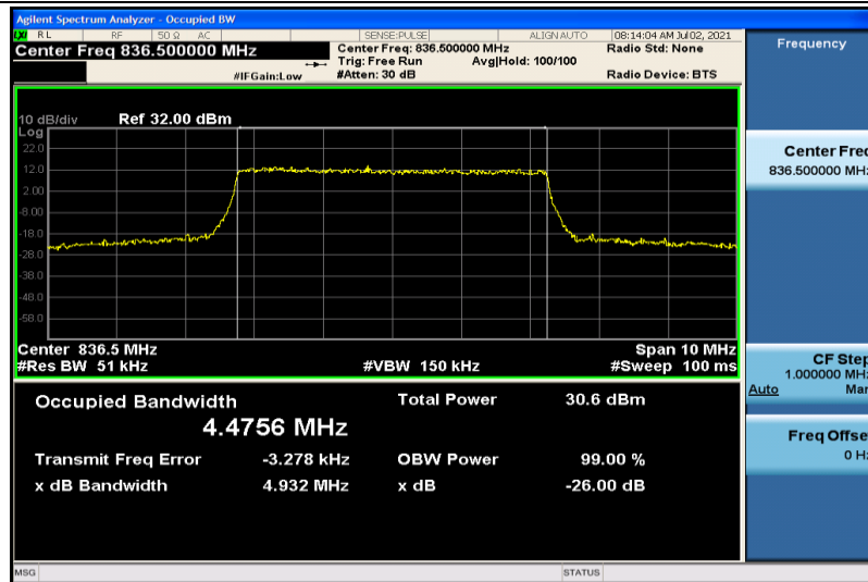
Band26-5MHz-QPSK-26915-25RB#0-4.4756
