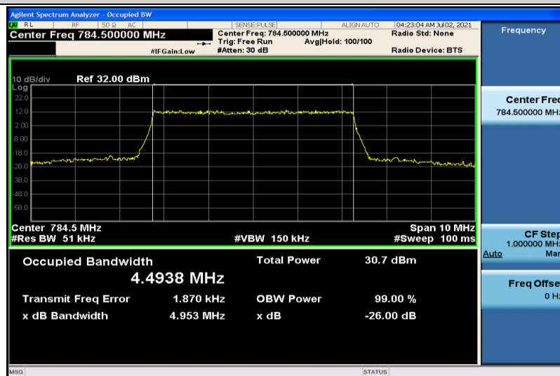
Band13-5MHz-QPSK-23255-25RB#0-4.4938
