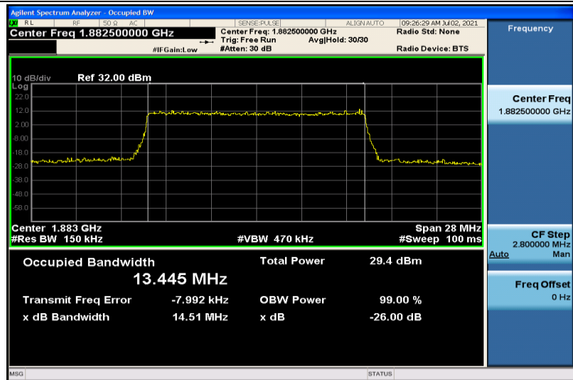
Band25-15MHz-16QAM-26365-75RB#0-13.445
