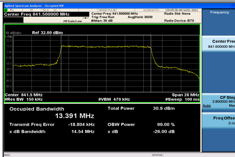
Band26-15MHz-QPSK-26965-75RB#0-13.391
