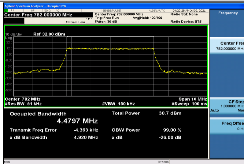
Band13-5MHz-QPSK-23230-25RB#0-4.4797
