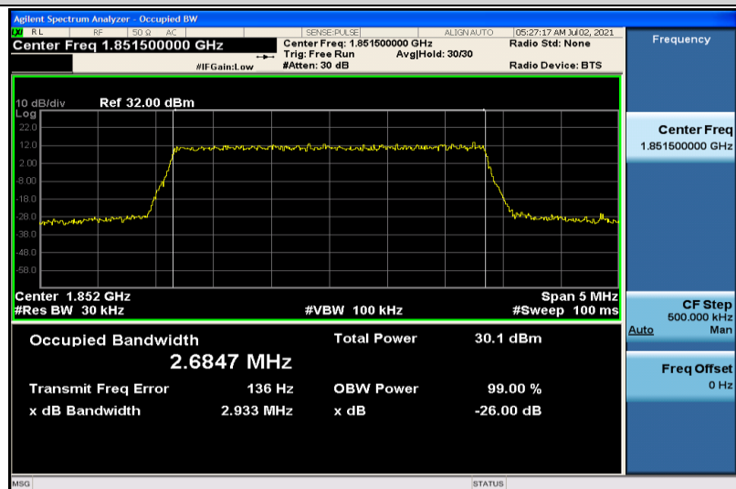
Band25-3MHz-QPSK-26055-15RB#0-2.6847
