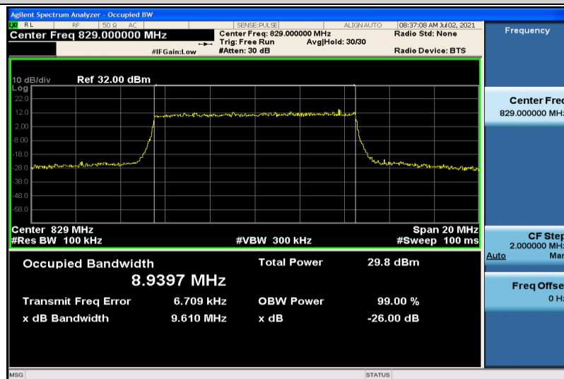
Band26-10MHz-16QAM-26840-50RB#0-8.9397
