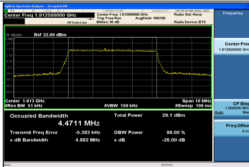
Band25-5MHz-16QAM-26665-25RB#0-4.4711
