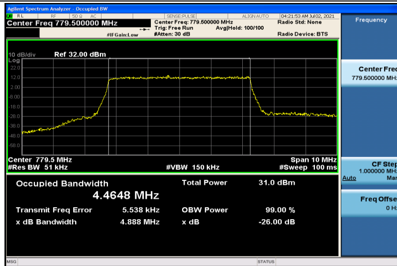
Band13-5MHz-QPSK-23205-25RB#0-4.4648
