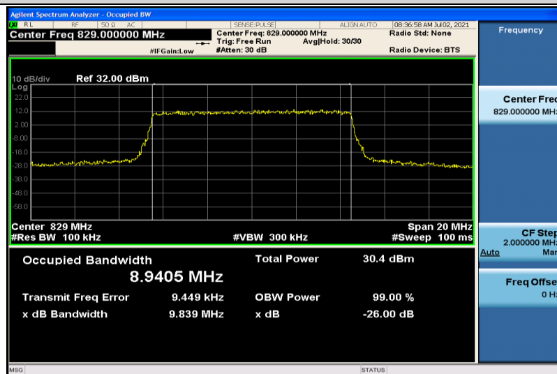
Band26-10MHz-QPSK-26840-50RB#0-8.9405
