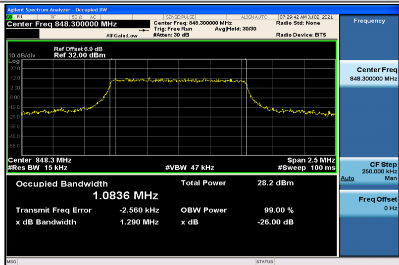
Band26-1.4MHz-16QAM-27033-6RB#0-1.0836
