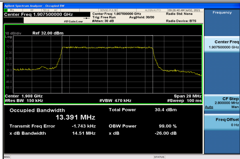
Band25-15MHz-QPSK-26615-75RB#0-13.391
