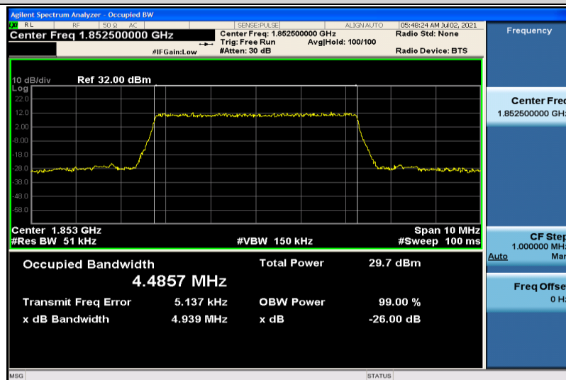
Band25-5MHz-16QAM-26065-25RB#0-4.4857
