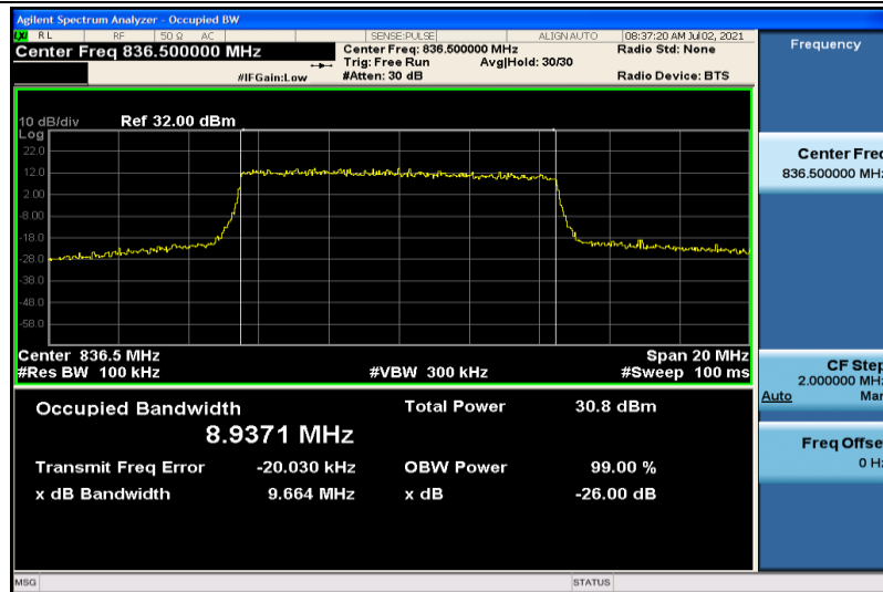
Band26-10MHz-QPSK-26915-50RB#0-8.9371
