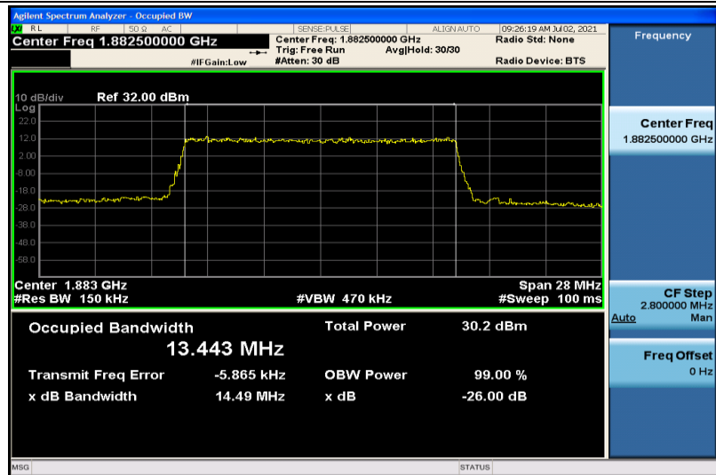
Band25-15MHz-QPSK-26365-75RB#0-13.443
