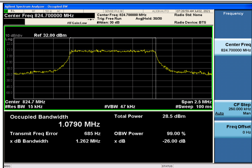
Band26-1.4MHz-16QAM-26797-6RB#0-1.0790
