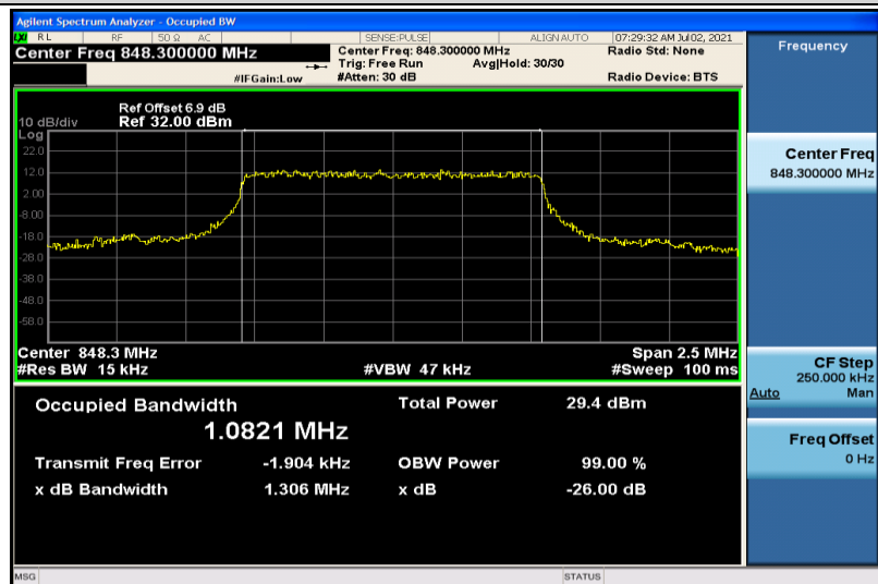
Band26-1.4MHz-QPSK-27033-6RB#0-1.0821
