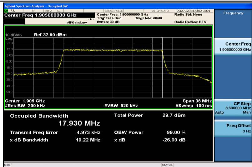
Band25-20MHz-16QAM-26590-100RB#0-17.930
