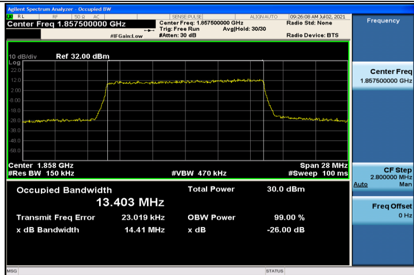
Band25-15MHz-16QAM-26115-75RB#0-13.403
