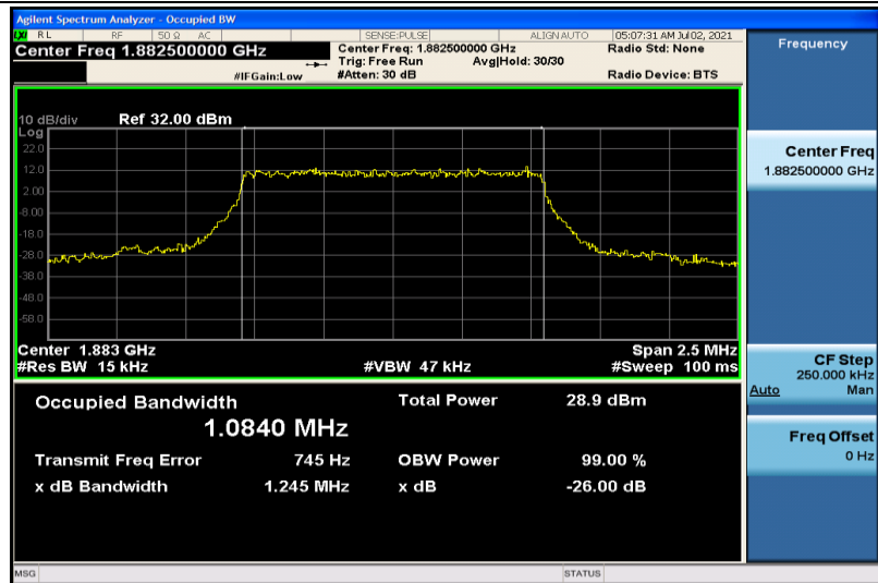
Band25-1.4MHz-QPSK-26365-6RB#0-1.0840
