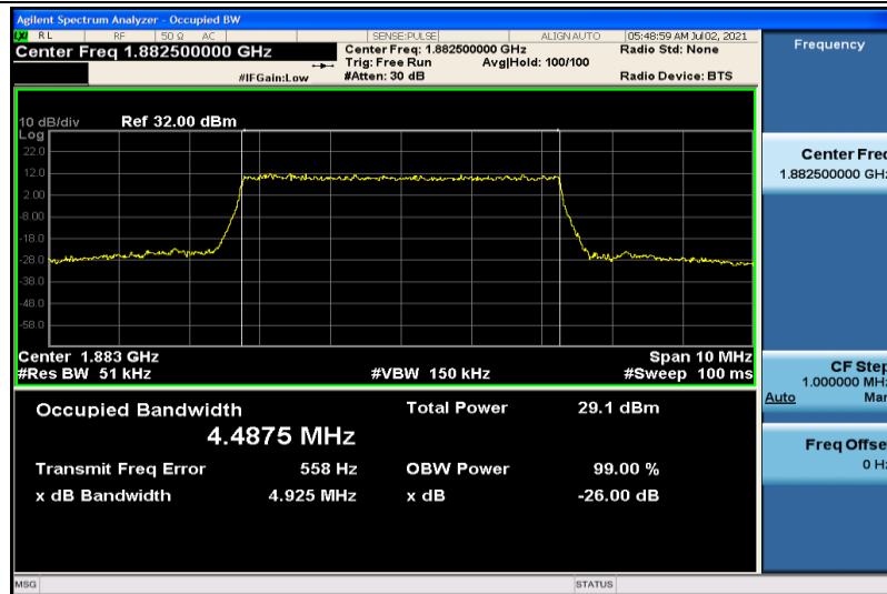
Band25-5MHz-16QAM-26365-25RB#0-4.4875
