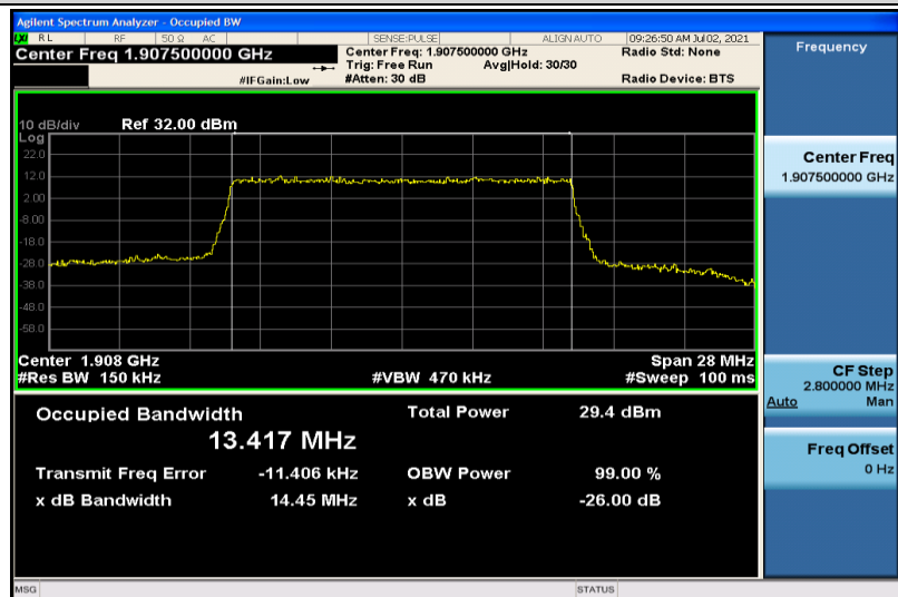
Band25-15MHz-16QAM-26615-75RB#0-13.417
