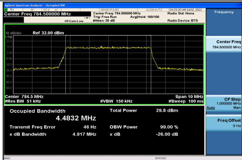
Band13-5MHz-16QAM-23255-25RB#0-4.4832
