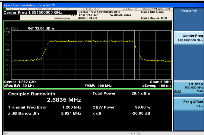
Band25-3MHz-16QAM-26055-15RB#0-2.6835
