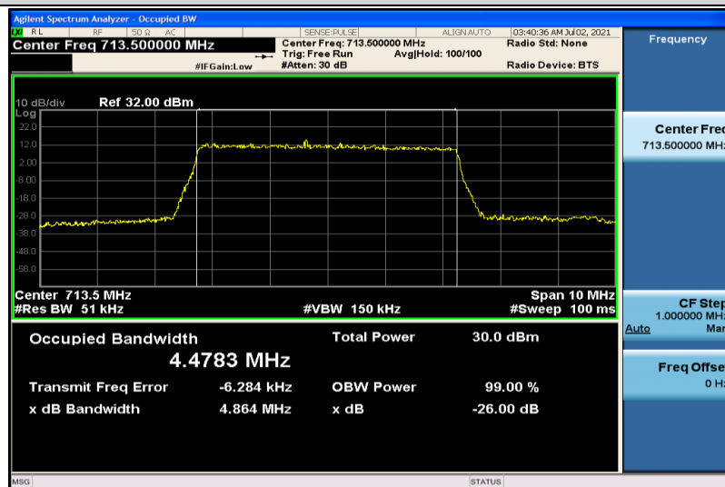
Band12-5MHz-16QAM-23155-25RB#0-4.4783
