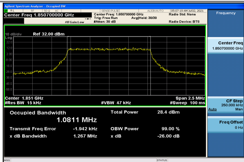
Band25-1.4MHz-16QAM-26047-6RB#0-1.0811
