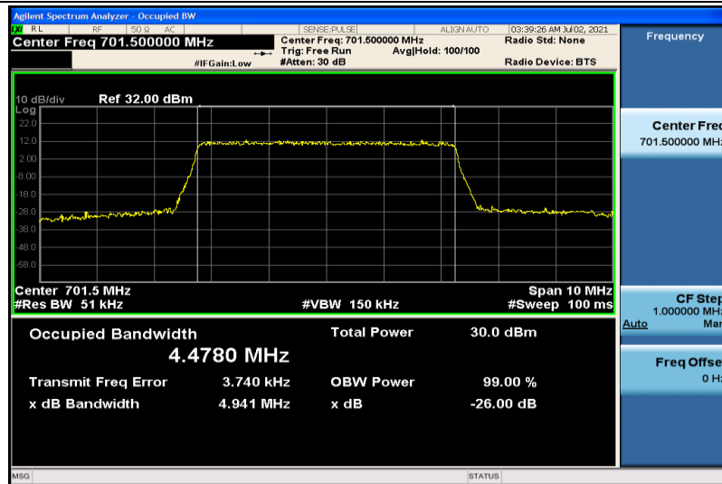
Band12-5MHz-16QAM-23035-25RB#0-4.4780
