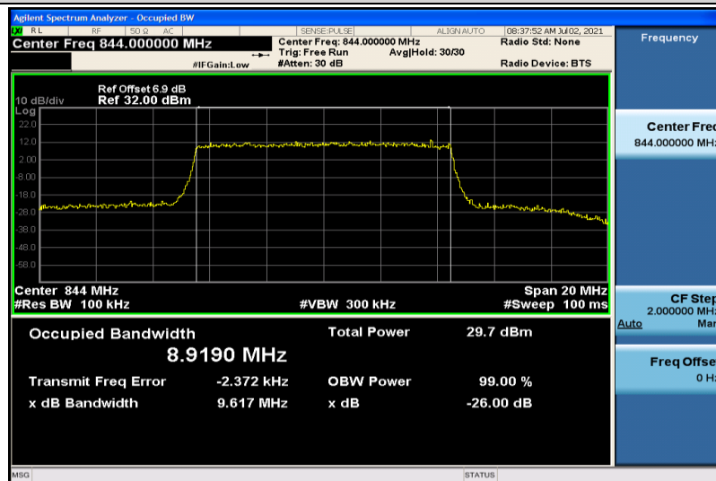
Band26-10MHz-16QAM-26990-50RB#0-8.9190
