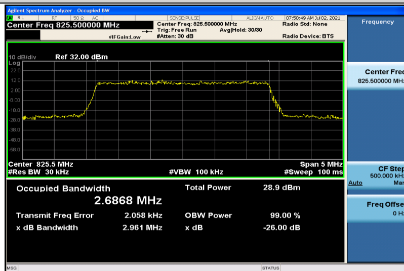
Band26-3MHz-16QAM-26805-15RB#0-2.6868
