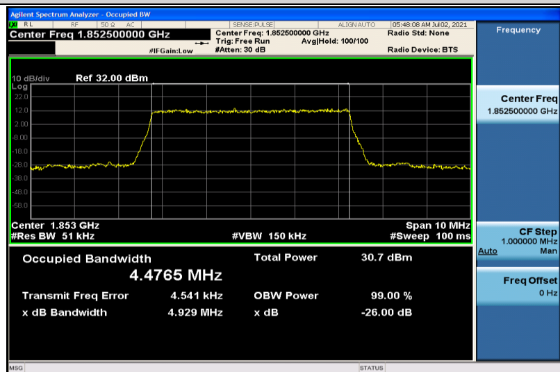
Band25-5MHz-QPSK-26065-25RB#0-4.4765
