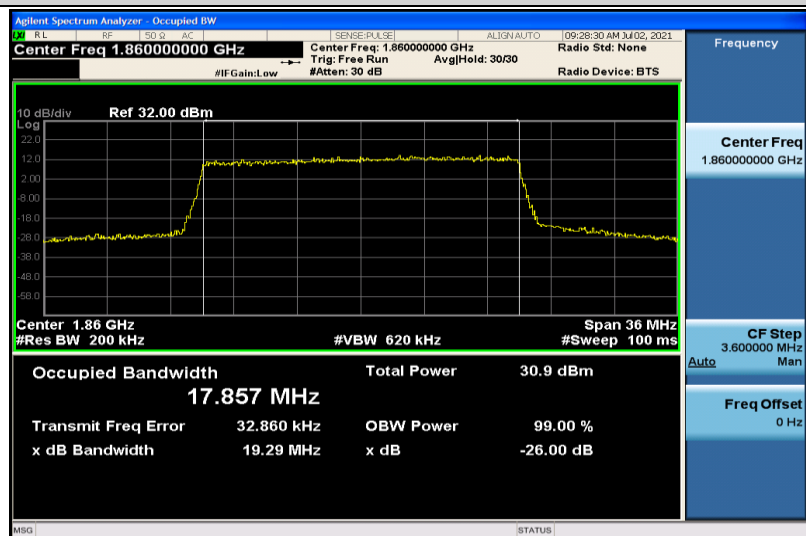
Band25-20MHz-QPSK-26140-100RB#0-17.857
