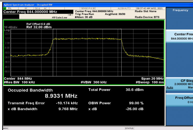
Band26-10MHz-QPSK-26990-50RB#0-8.9331
