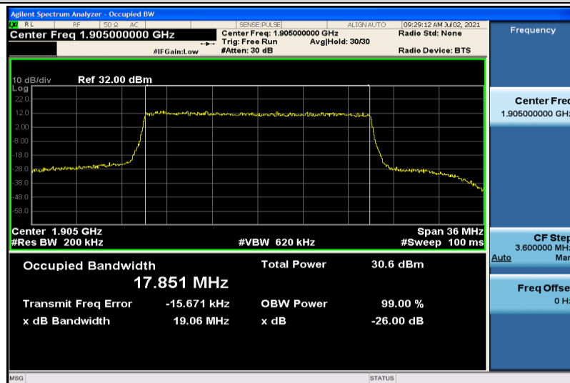
Band25-20MHz-QPSK-26590-100RB#0-17.851
