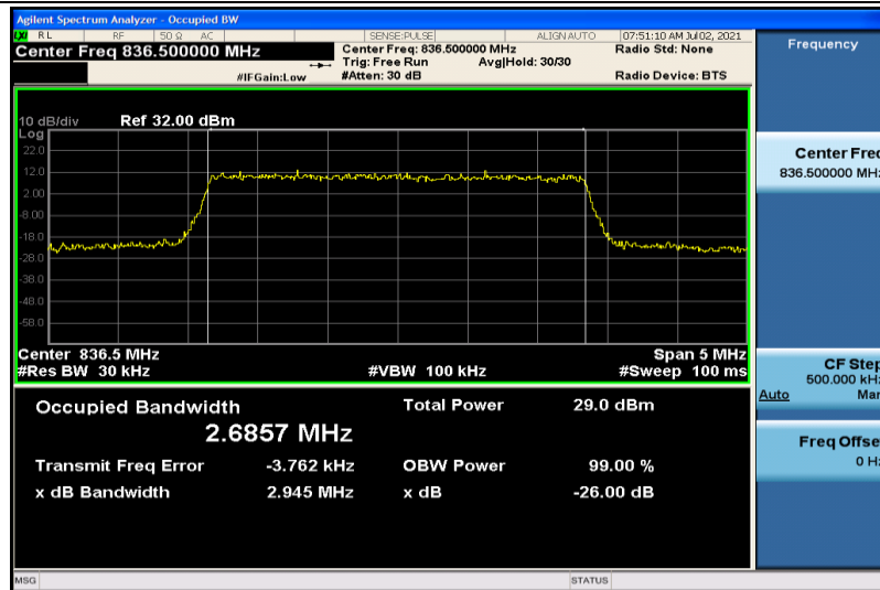
Band26-3MHz-16QAM-26915-15RB#0-2.6857
