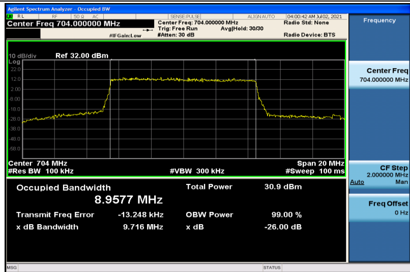
Band12-10MHz-QPSK-23060-50RB#0-8.9577
