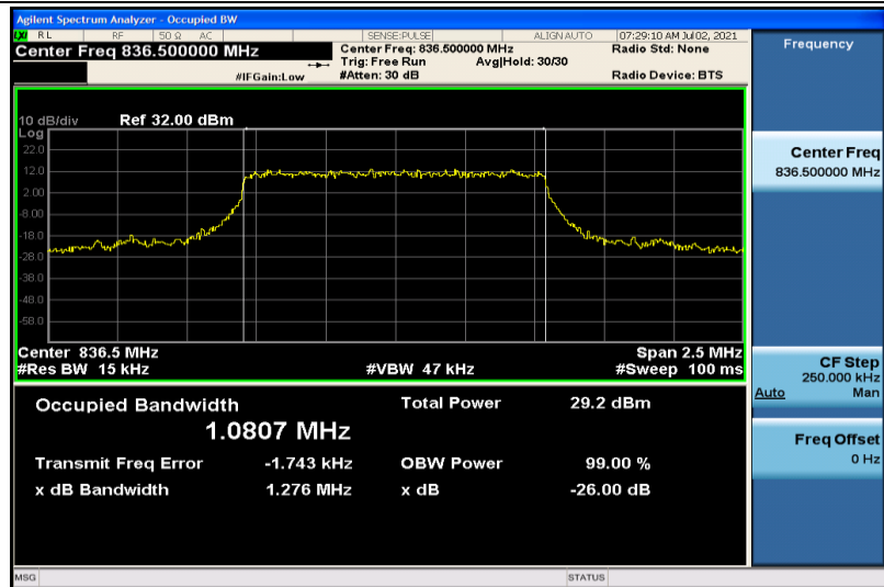
Band26-1.4MHz-QPSK-26915-6RB#0-1.0807
