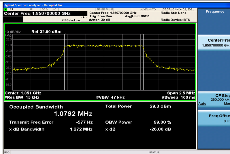
Band25-1.4MHz-QPSK-26047-6RB#0-1.0792
