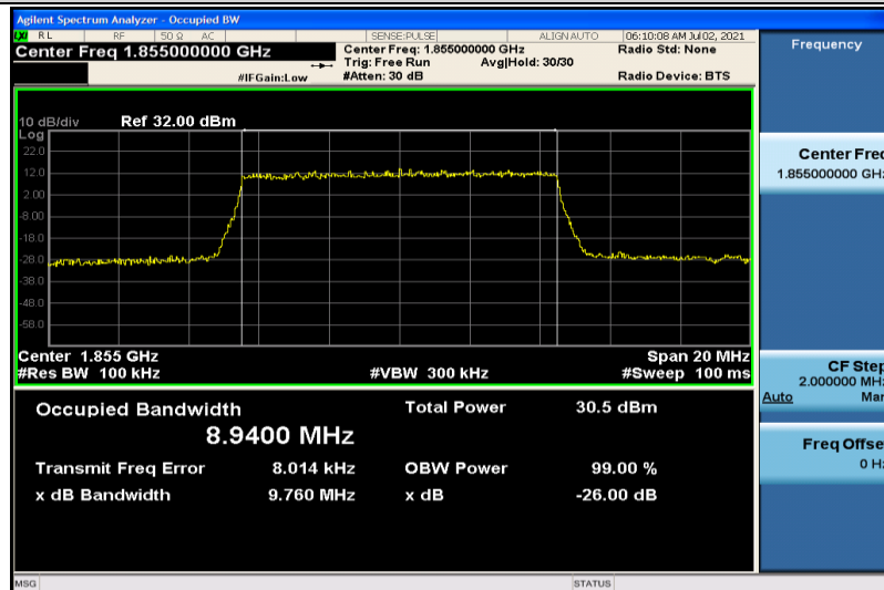
Band25-10MHz-QPSK-26090-50RB#0-8.9400
