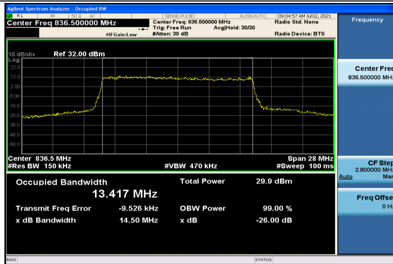
Band26-15MHz-16QAM-26915-75RB#0-13.417
