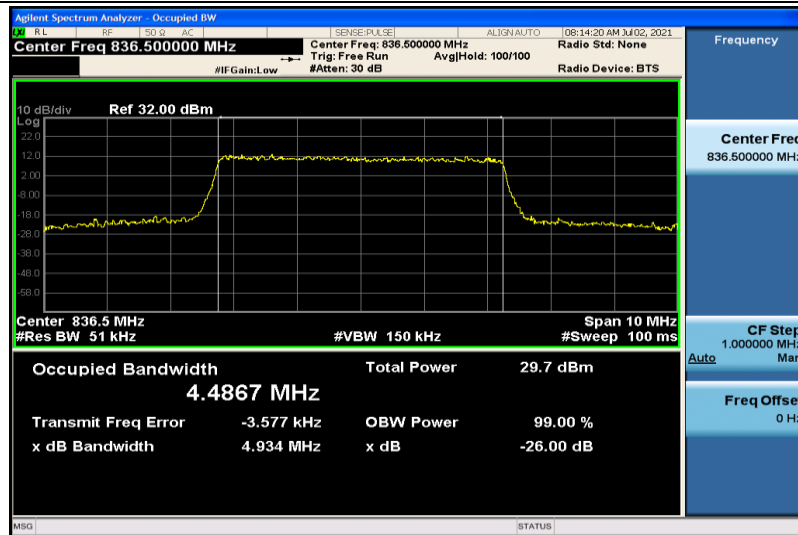
Band26-5MHz-16QAM-26915-25RB#0-4.4867
