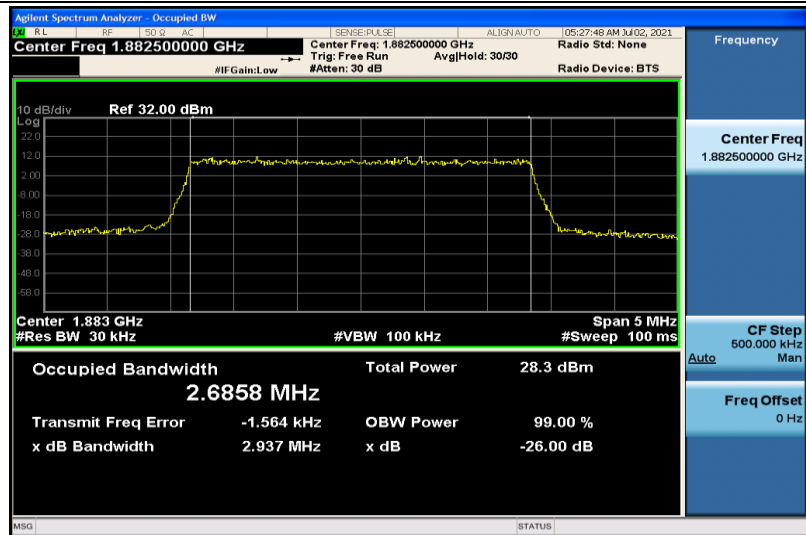
Band25-3MHz-16QAM-26365-15RB#0-2.6858
