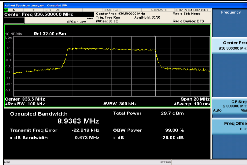
Band26-10MHz-16QAM-26915-50RB#0-8.9363
