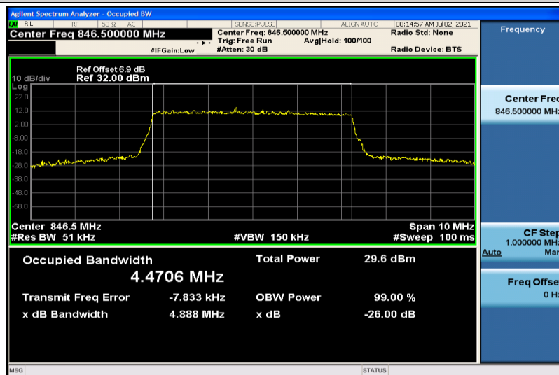
Band26-5MHz-16QAM-27015-25RB#0-4.4706
