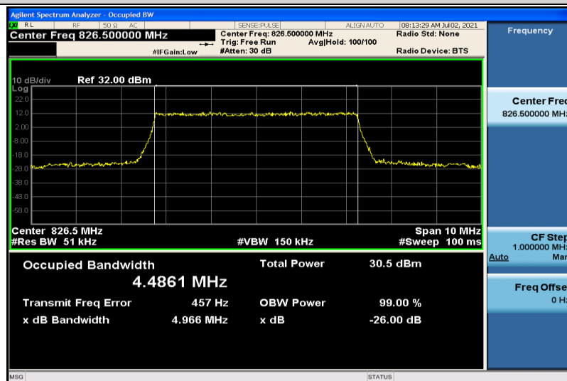
Band26-5MHz-QPSK-26815-25RB#0-4.4861
