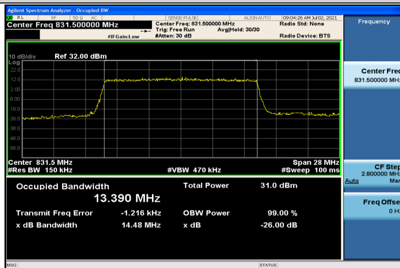
Band26-15MHz-QPSK-26865-75RB#0-13.390
