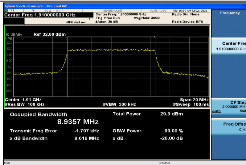
Band25-10MHz-16QAM-26640-50RB#0-8.9357
