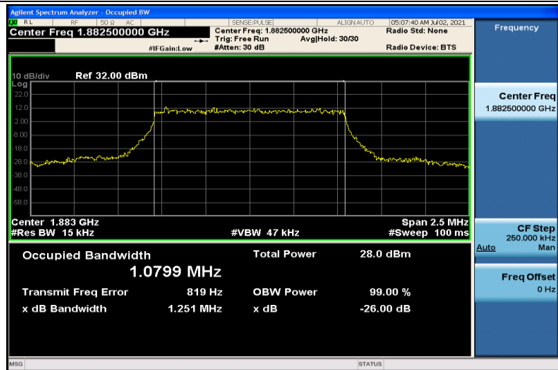
Band25-1.4MHz-16QAM-26365-6RB#0-1.0799
