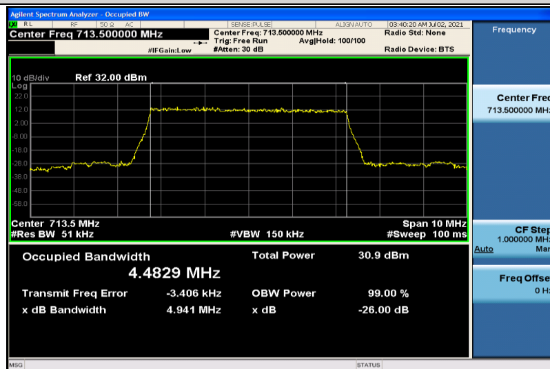
Band12-5MHz-QPSK-23155-25RB#0-4.4829
