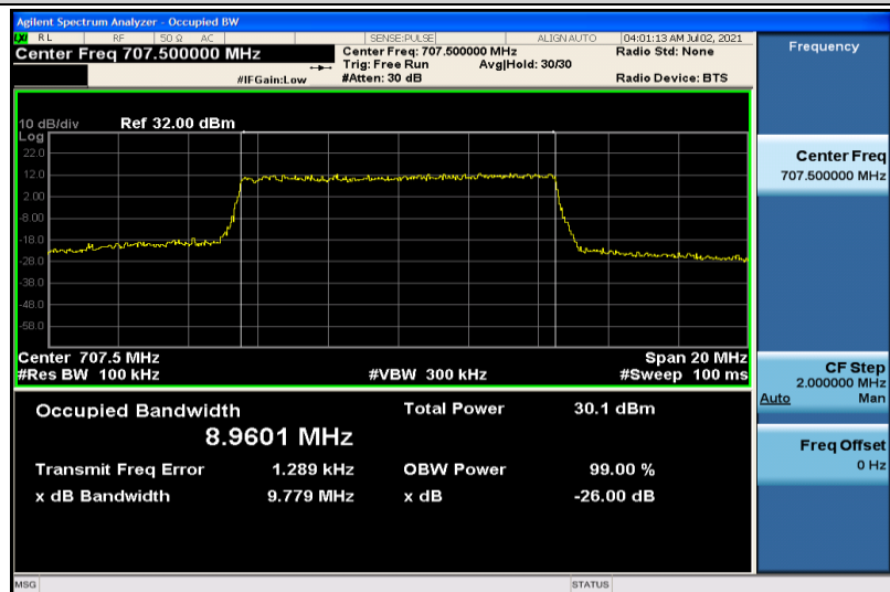
Band12-10MHz-16QAM-23095-50RB#0-8.9601
