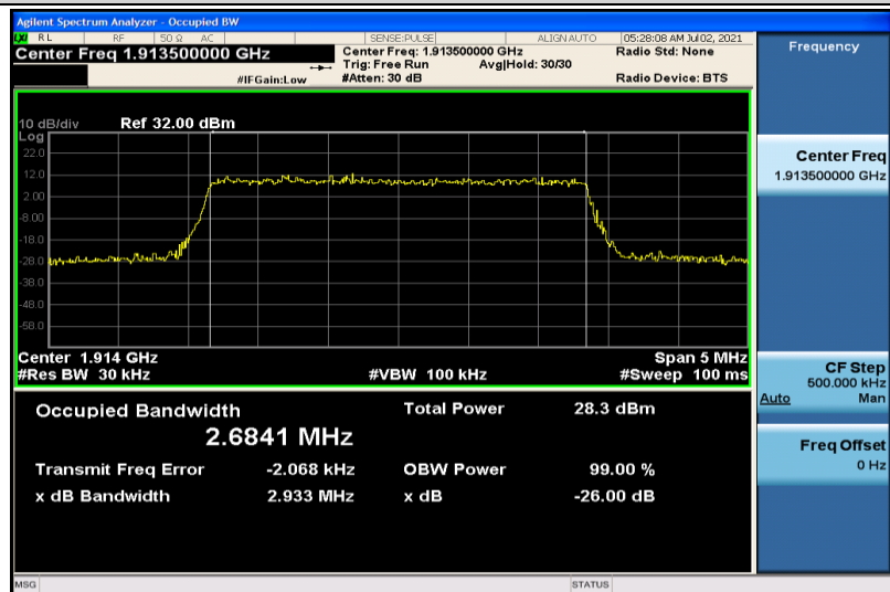
Band25-3MHz-16QAM-26675-15RB#0-2.6841
