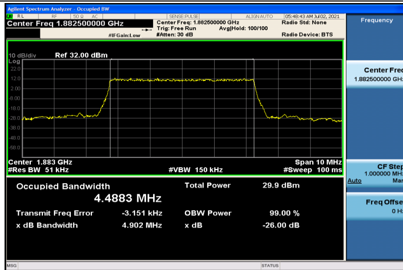
Band25-5MHz-QPSK-26365-25RB#0-4.4883
