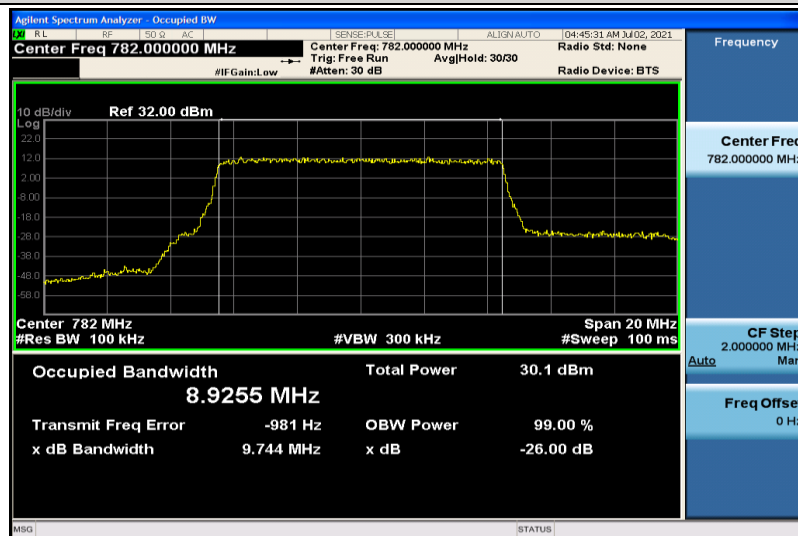
Band13-10MHz-16QAM-23230-50RB#0-8.9255
