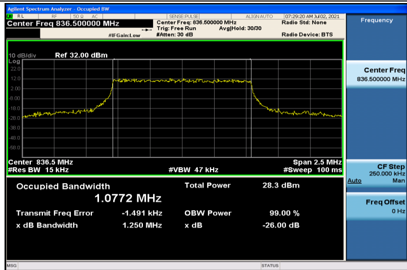
Band26-1.4MHz-16QAM-26915-6RB#0-1.0772
