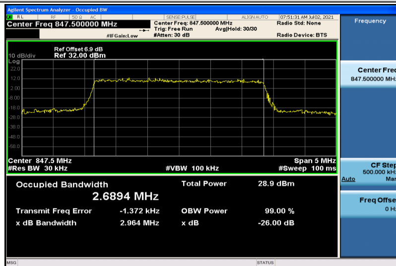
Band26-3MHz-16QAM-27025-15RB#0-2.6894
