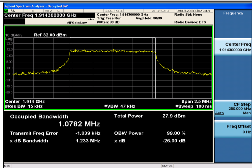
Band25-1.4MHz-16QAM-26683-6RB#0-1.0782
