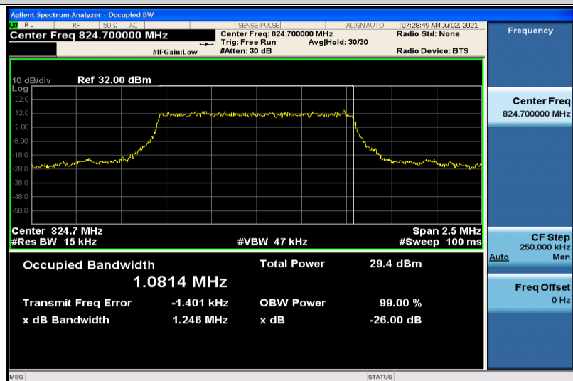
Band26-1.4MHz-QPSK-26797-6RB#0-1.0814
