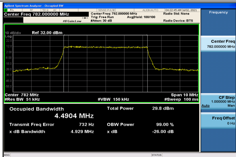
Band13-5MHz-16QAM-23230-25RB#0-4.4904
