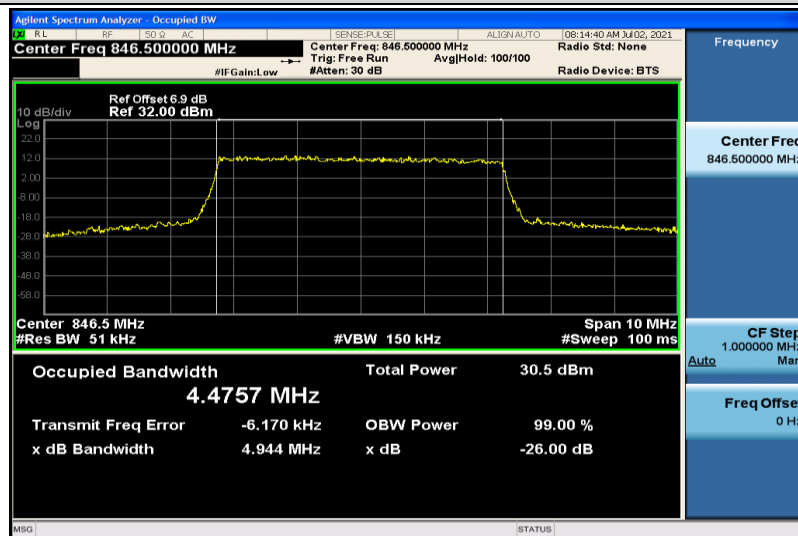
Band26-5MHz-QPSK-27015-25RB#0-4.4757
