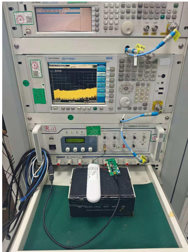
RF Conducted test setup photo
