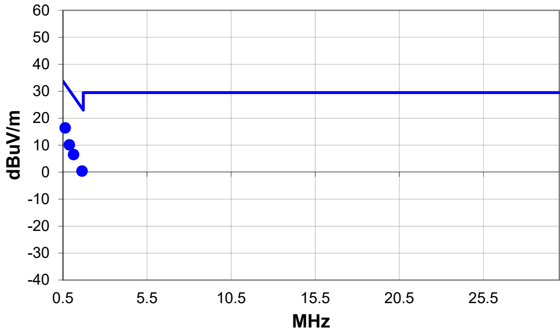
490 kHz-30 MHz Maximised
