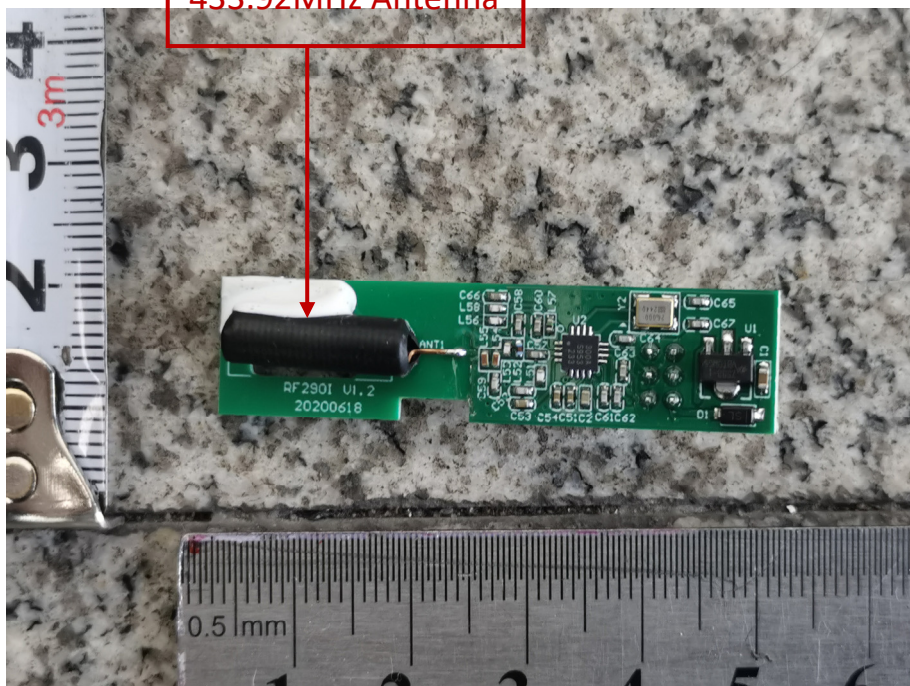
433.92MHz Antenna
