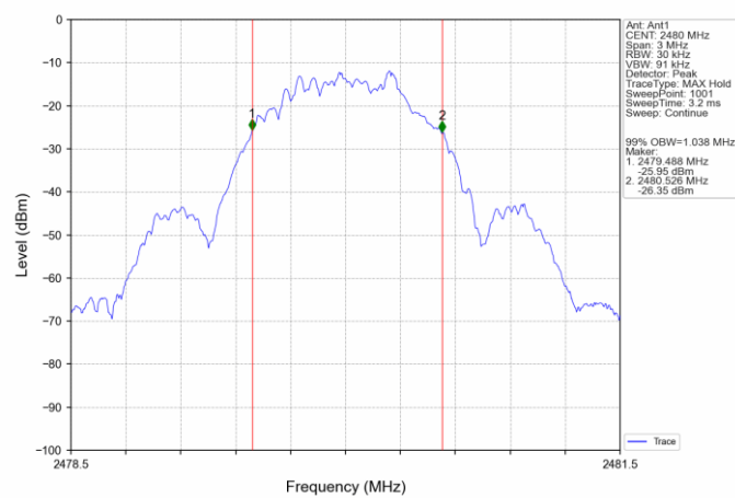
1M_HCH_2480MHz_Ant1_NTNV
