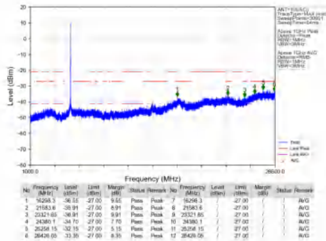
802.11a_LCH_5180MHz_Ant1_NTNV
