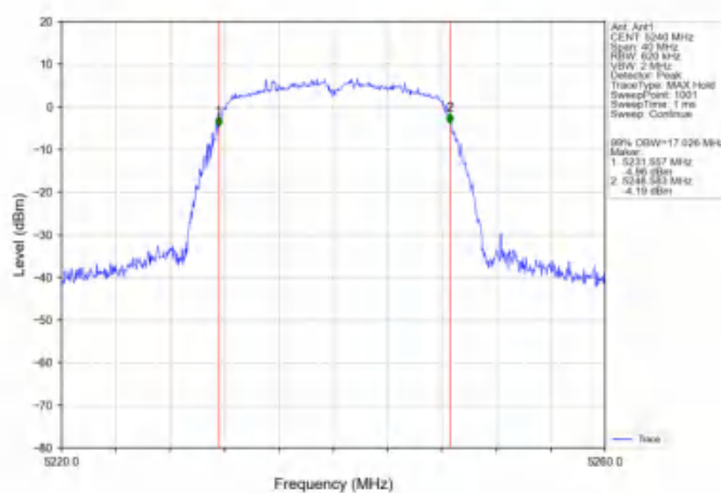
802.11a_HCH_5240MHz_Ant1_NTNV
