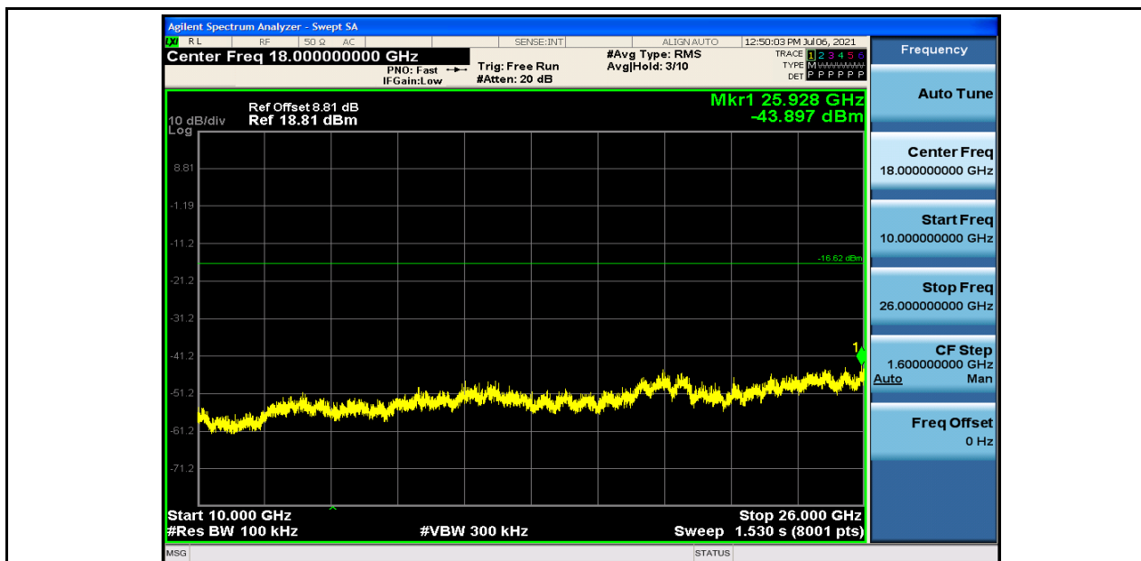
RF Conducted Spurious Emissions_BLE_2440_1M
