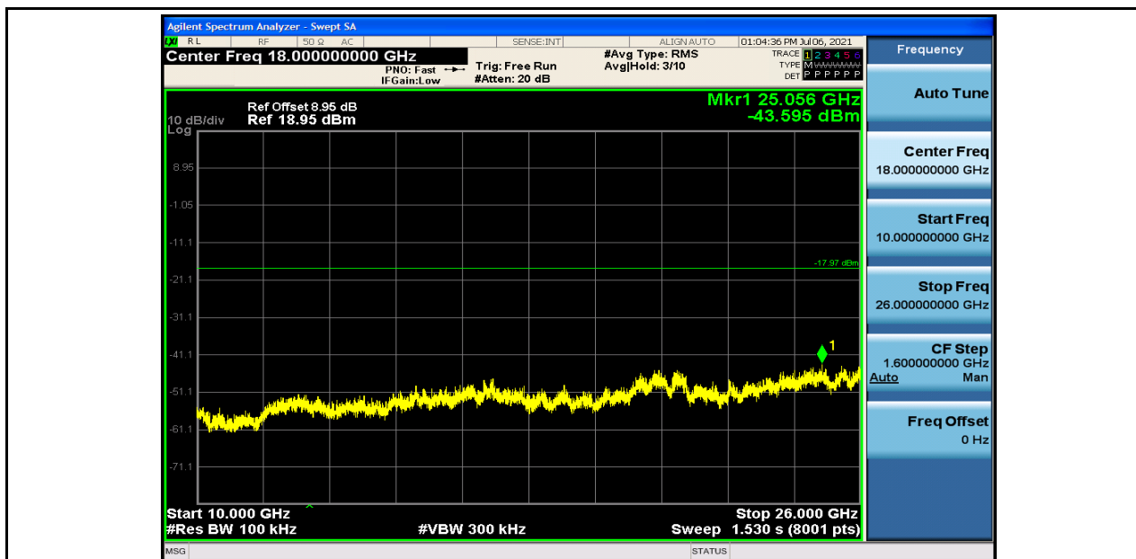
RF Conducted Spurious Emissions_BLE_2480_2M
