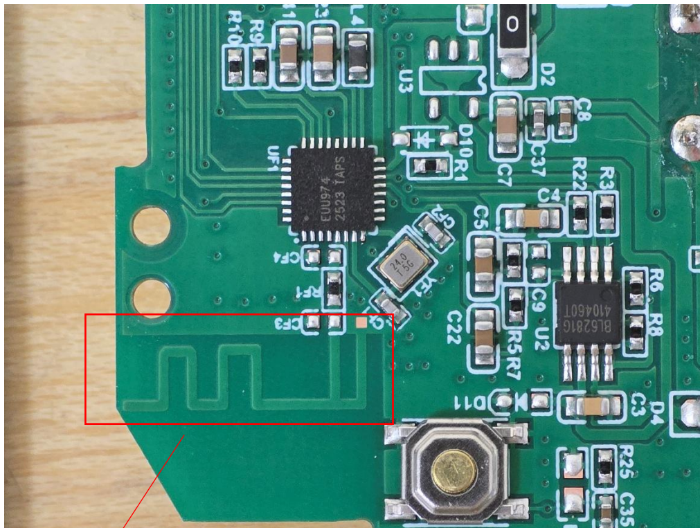
PCB Antenna
