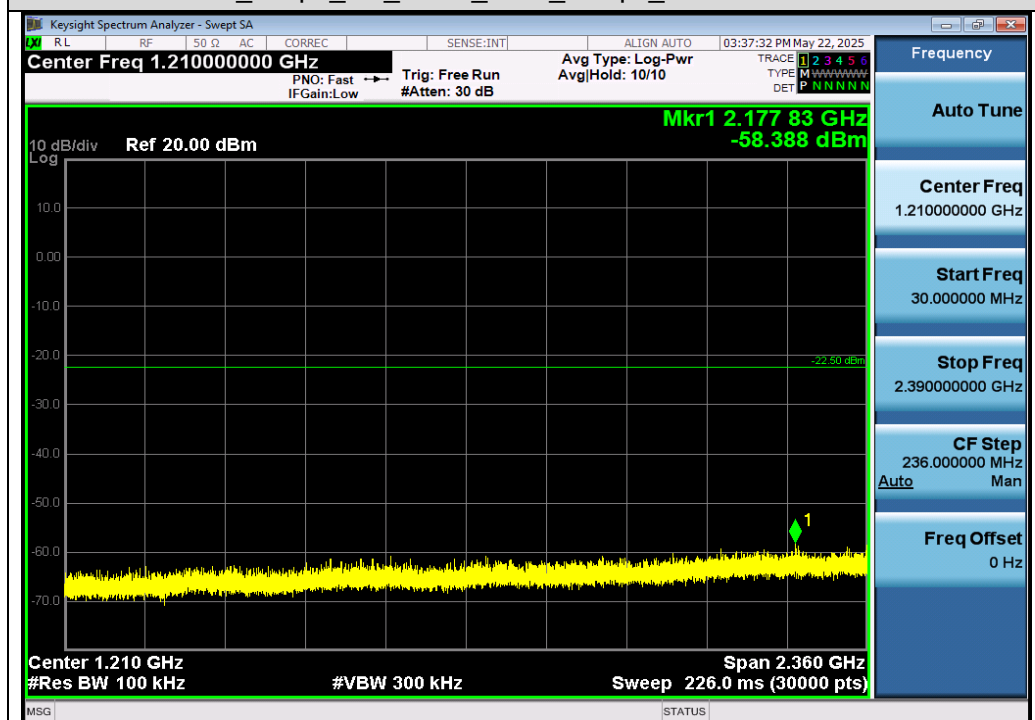
Test_Graph_BR_ANT1_2402_1Mbps_Lower Band Emissions
