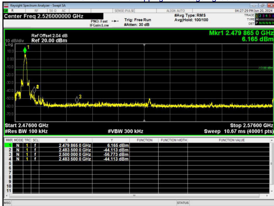
8-DPSK -3-DH1 No-hopping Band edge-right side
