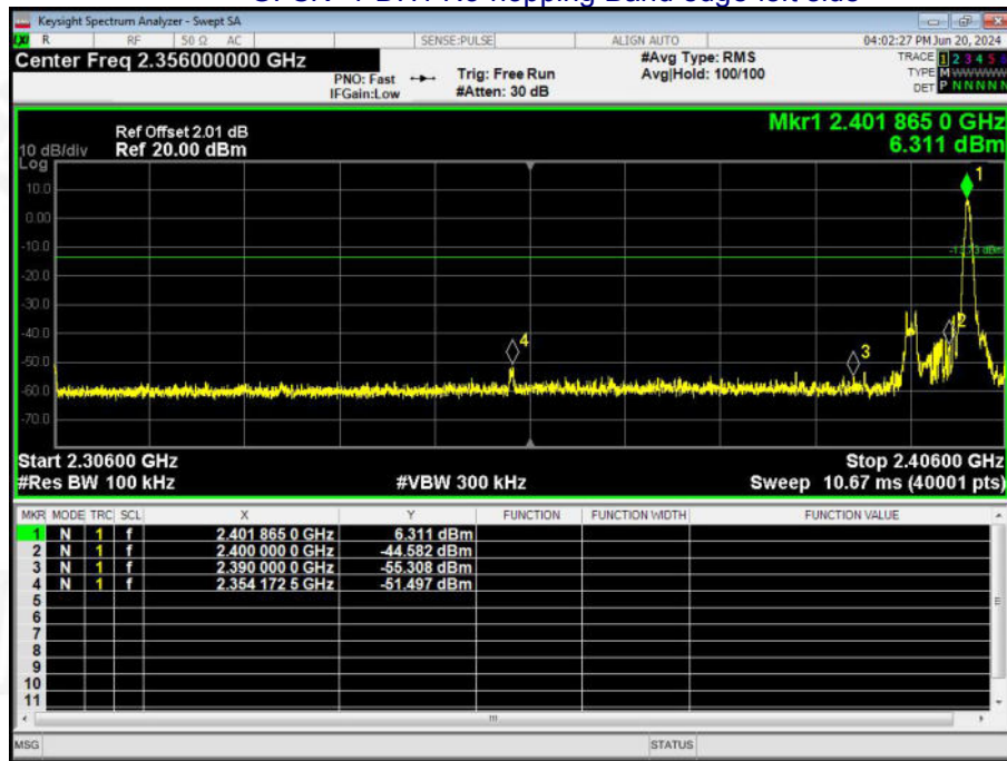
GFSK -1-DH1 No-hopping Band edge-left side
