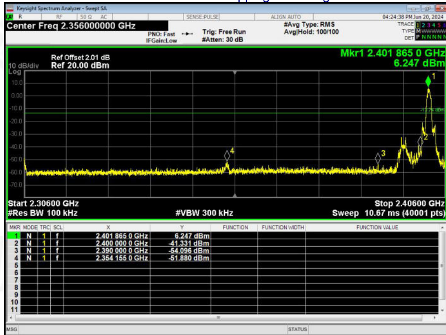
8-DPSK -3-DH1 No-hopping Band edge-left side
