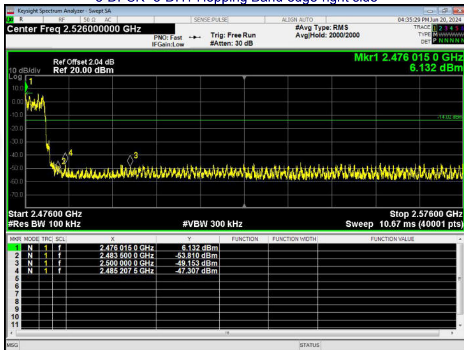
8-DPSK -3-DH1 Hopping Band edge-right side
