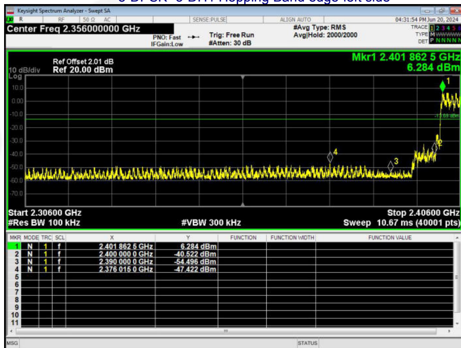
8-DPSK -3-DH1 Hopping Band edge-left side
