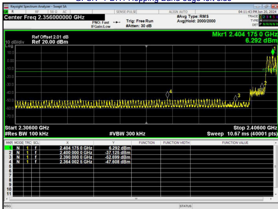
GFSK -1-DH1 Hopping Band edge-left side
