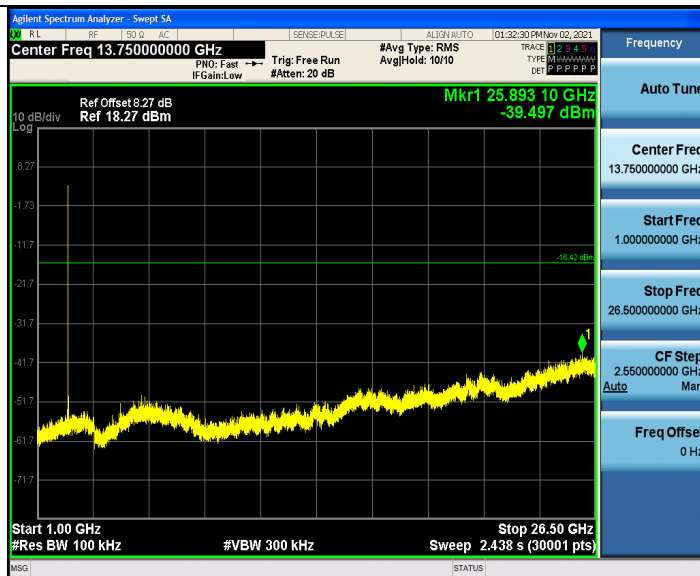
GFSK Ant1_2439_0~Reference
