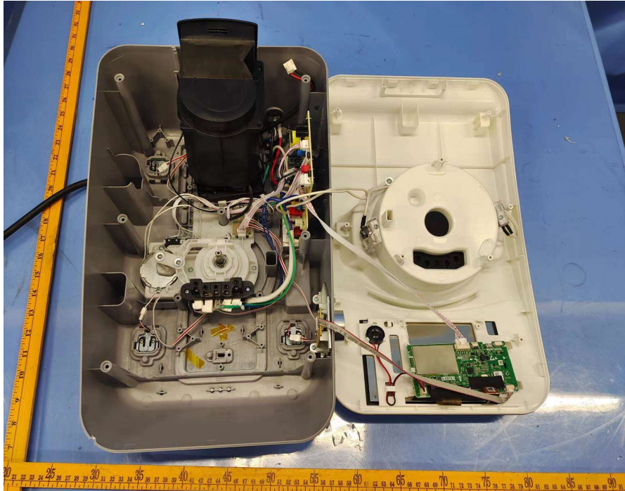
Internal view for K3302
