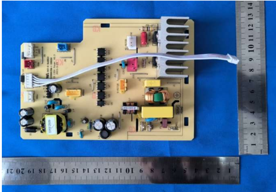
Power PCB view for both models
