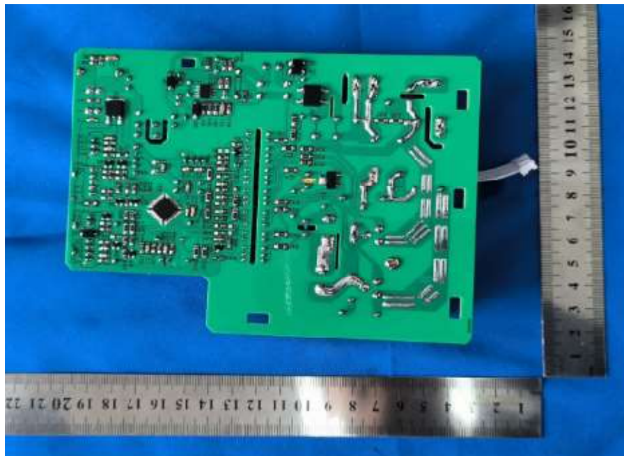
Power PCB view for both models
