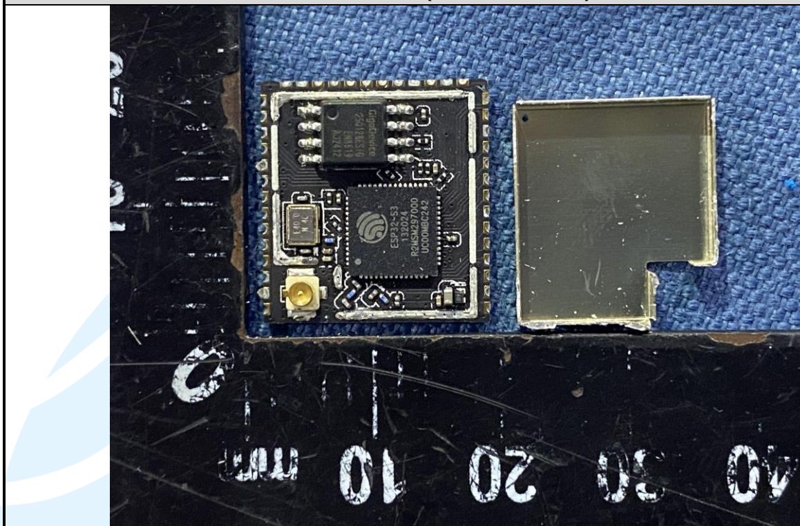
EUT Photo (BT&amp;Wi-Fi module)
