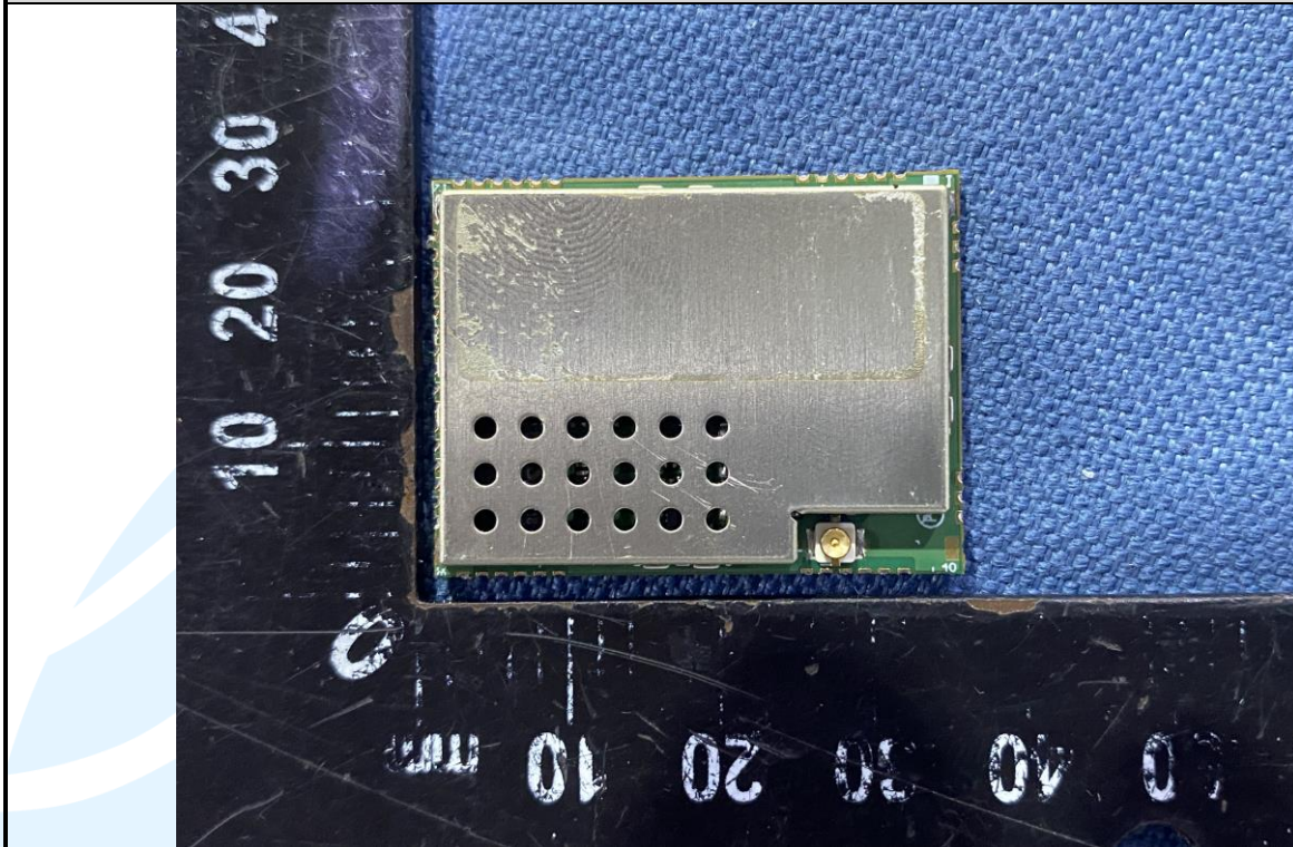
EUT Photo (902-928MHz RX module)
