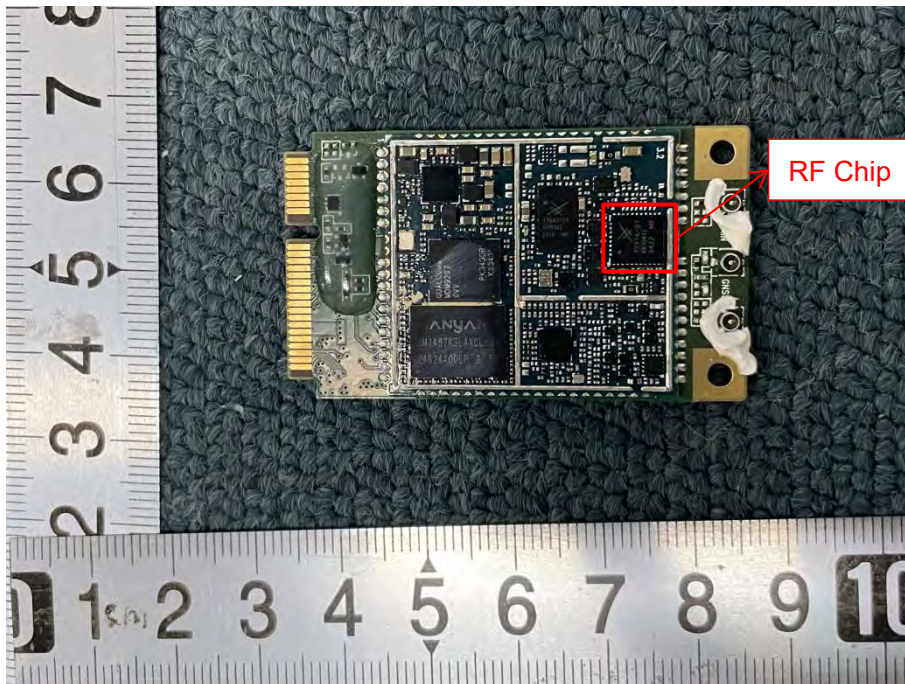
SECONDARY BOARD 6 TOP VIEW (WITHOUT SHIELDING)
