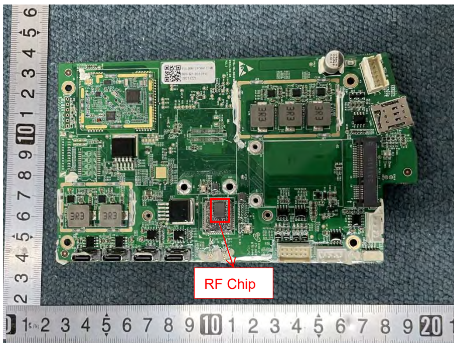
SECONDARY BOARD 7 TOP VIEW (WITHOUT SHIELDING)
