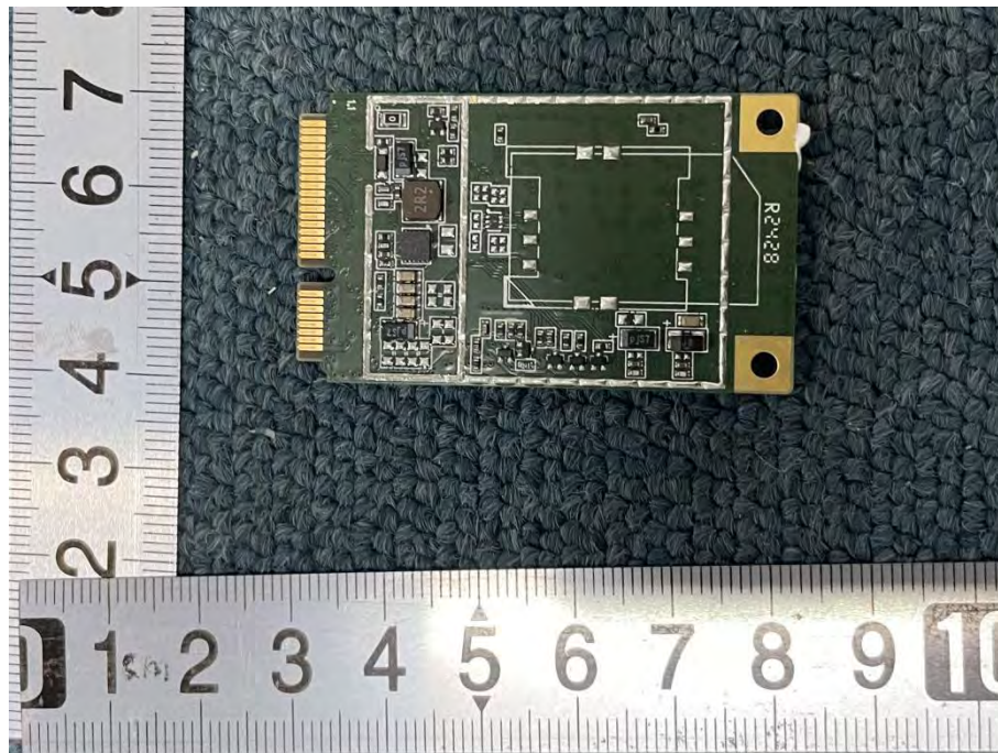
SECONDARY BOARD 6 REAR VIEW (WITHOUT SHIELDING)
