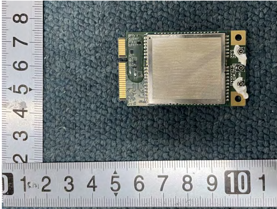
SECONDARY BOARD 6 TOP VIEW (WITH SHIELDING)
