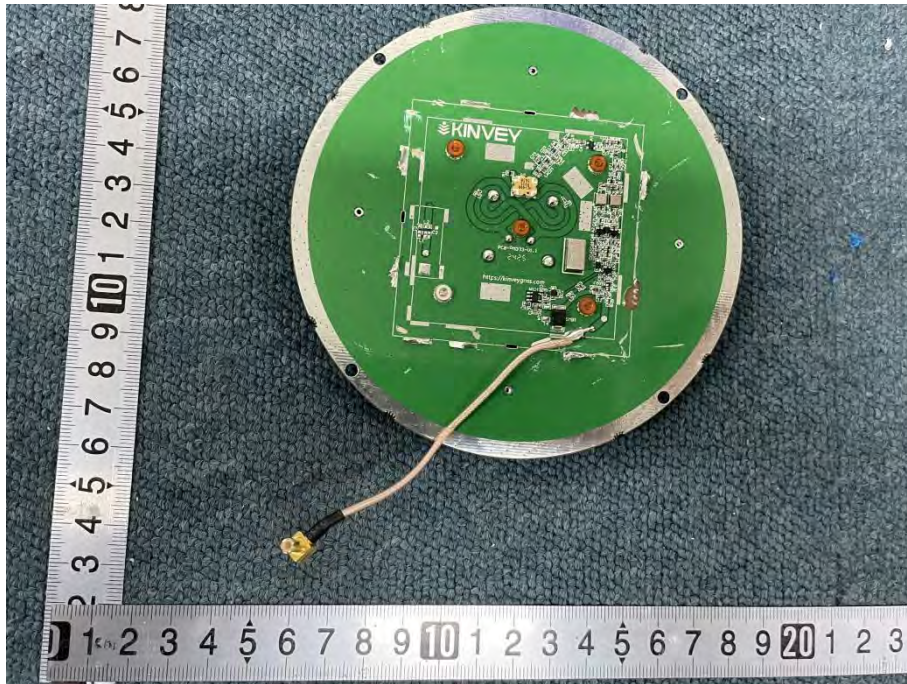
SECONDARY BOARD 8 TOP VIEW (WITHOUT SHIELDING)
