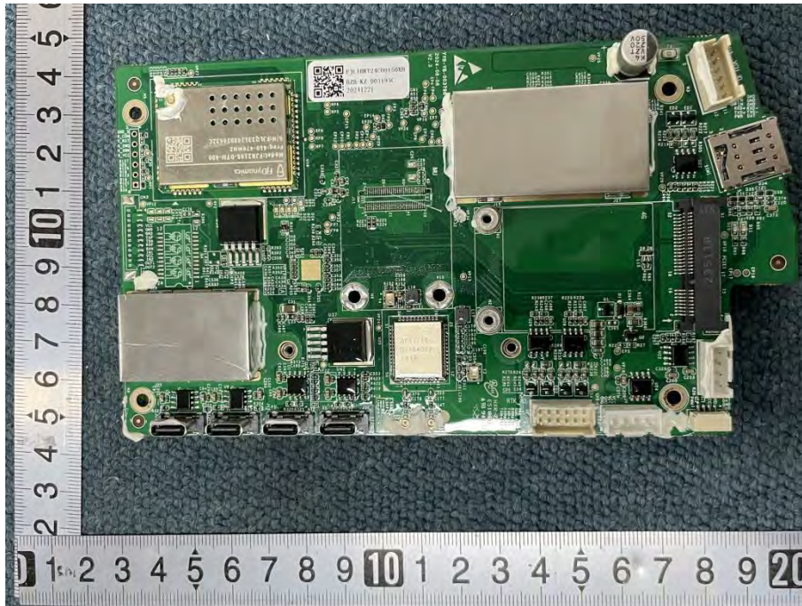
SECONDARY BOARD 7 TOP VIEW (WITH SHIELDING)
