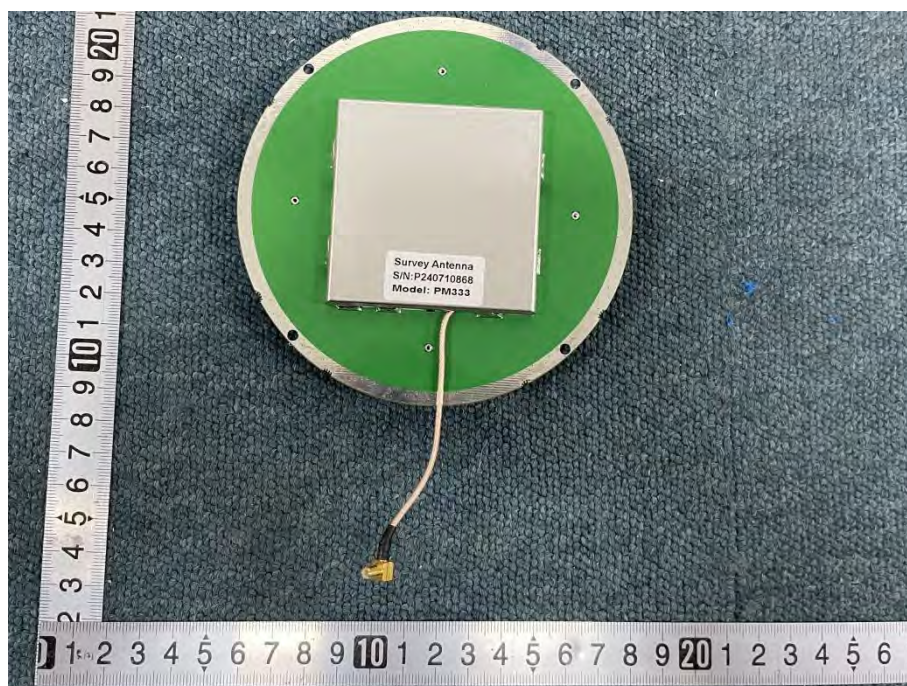
SECONDARY BOARD 8 TOP VIEW (WITH SHIELDING)
