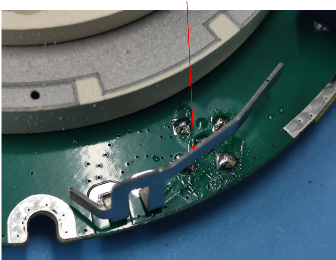
WWANAntenna
