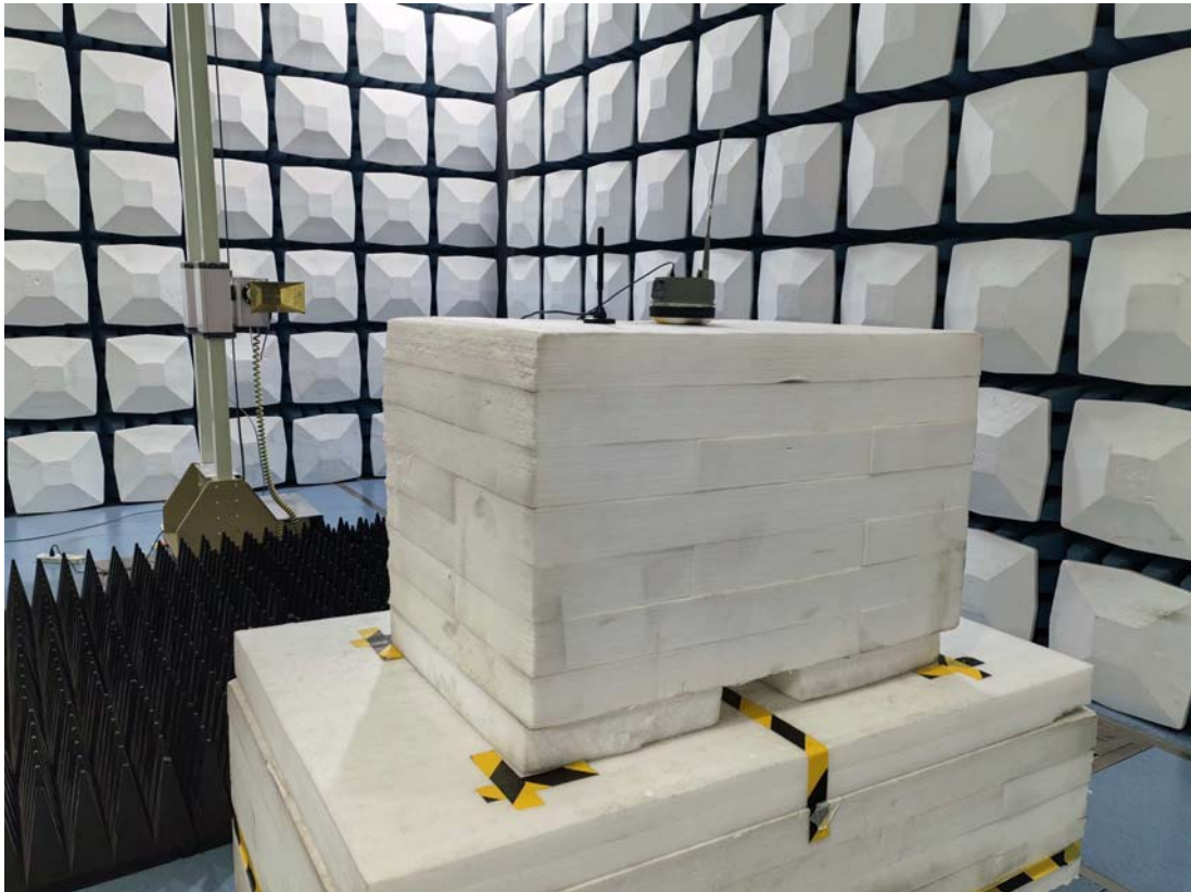
Radiated Emission 1-18GHz View
