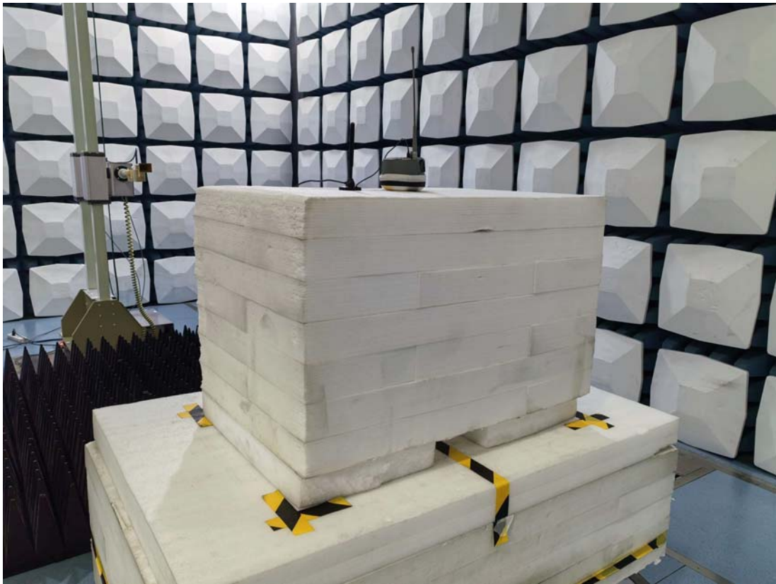
Radiated Emission 26.5-27GHz View
