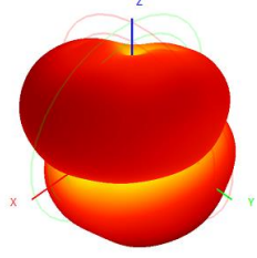
2440.0MHz H+V, Eff: 48.5%
