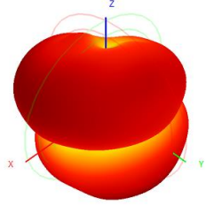
2450.0MHz H+V, Eff: 51.2%
