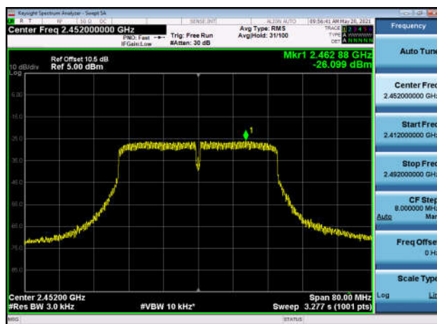
Power spectral density-802.11n(HT40) ,2452MHz
