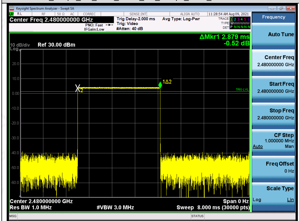
Test Graph BR HOP ANT1 NA 1Mbps 2480 Time per Burst 1 1 1 1 1 1 1 1 1 2 1 1 1 1 1 1 1 1 3 1 1 1 1 1 1 1 1 4 1 1 1 1 1 1 1 1 5 1 1 1 1 1 1 1 1 6 1 1 1 1 1 1 1 1 7 1 1 1 1 1 1 1 1 8 1 1 1 1 1 1 1 1 9 1 1 1 1 1 1 1 1 10 1 1 1 1 1 1 1 1 11 1 1 1 1 1 1 1 1 12 1 1 1 1 1 1 1 1 13 1 1 1 1 1 1 1 1 14 1 1 1 1 1 1 1 1 15 1 1 1 1 1 1 1 1 16 1 1 1 1 1 1 1 1 17 1 1 1 1 1 1 1 1 18 1 1 1 1 1 1 1 1 19 1 1 1 1 1 1 1 1 20 1 1 1 1 1 1 1 1 21 1 1 1 1 1 1 1 1 22 1 1 1 1 1 1 1 1 23 1 1 1 1 1 1 1 1 24 1 1 1 1 1 1 1 1 25 1 1 1 1 1 1 1 1 26 1 1 1 1 1 1 1 1 27 1 1 1 1 1 1 1 1 28 1 1 1 1 1 1 1 1 29 1 1 1 1 1 1 1 1 30 1 1 1 1 1 1 1 1 31 1 1 1 1 1 1 1 1 32 1 1 1 1 1 1 1 1 33 1 1 1 1 1 1 1 1 34 1 1 1 1 1 1 1 1 35 1 1 1 1 1 1 1 1 36 1 1 1 1 1 1 1 1 37 1 1 1 1 1 1 1 1 38 1 1 1 1 1 1 1 1 39 1 1 1 1 1 1 1 1 40 1 1 1 1 1 1 1 1 41 1 1 1 1 1 1 1 1 42 1 1 1 1 1 1 1 1 43 1 1 1 1 1 1 1 1 44 1 1 1 1 1 1 1 1 45 1 1 1 1 1 1 1 1 46 1 1 1 1 1 1 1 1 47 1 1 1 1 1 1 1 1 48 1 1 1 1 1 1 1 1 49 1 1 1 1 1 1 1 1 50 1 1 1 1 1 1 1 1 51 1 1 1 1 1 1 1 1 52 1 1 1 1 1 1 1 1 53 1 1 1 1 1 1 1 1 54 1 1 1 1 1 1 1 1 55 1 1 1 1 1 1 1 1 56 1 1 1 1 1 1 1 1 57 1 1 1 1</
