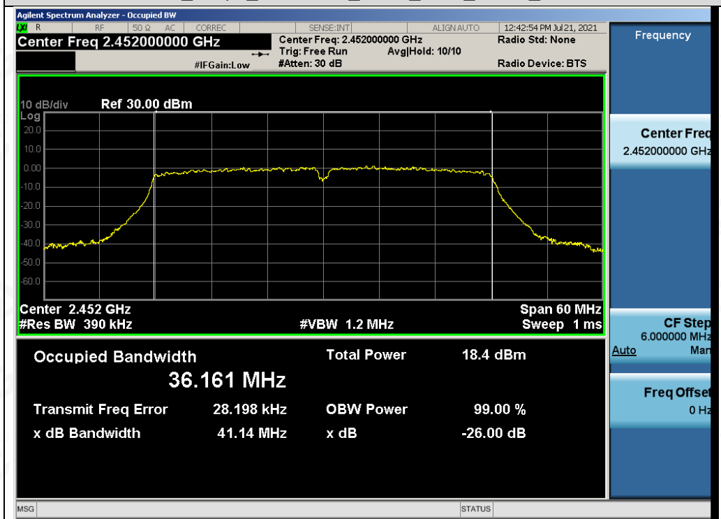
Test_Graph_802.11n40_ANT2_2452_MCS0_OBW
