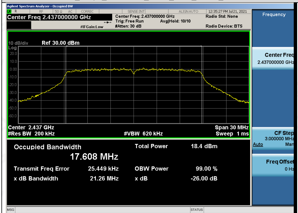
Test_Graph_802.11n20_ANT2_2437_MCS0_OBW
