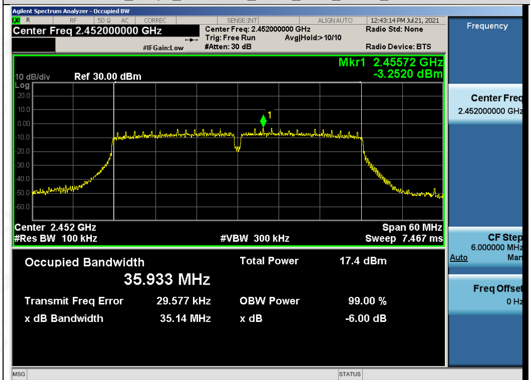
Test_Graph_802.11n40_ANT2_2452_MCS0_DTSBW
