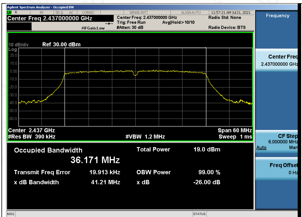
Test_Graph_802.11n40_ANT1_2437_MCS0_OBW
