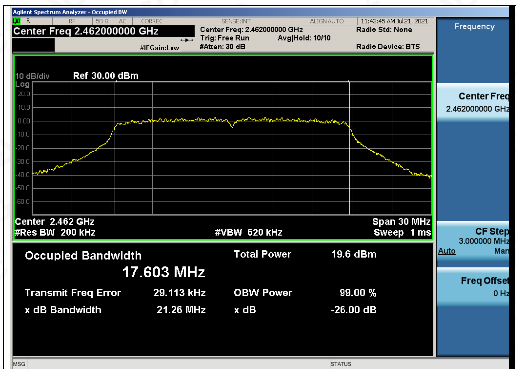
Test_Graph_802.11n20_ANT1_2462_MCS0_OBW
