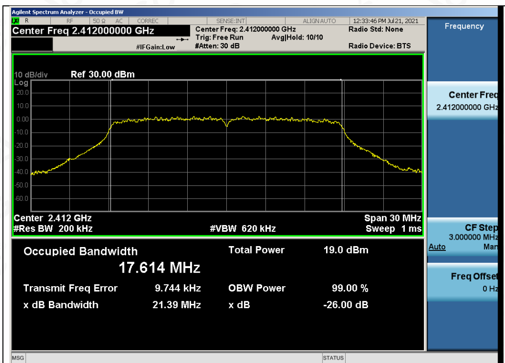
Test_Graph_802.11n20_ANT2_2412_MCS0_OBW
