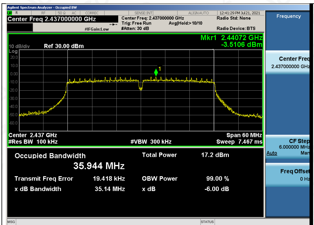
Test_Graph_802.11n40_ANT2_2437_MCS0_DTSBW
