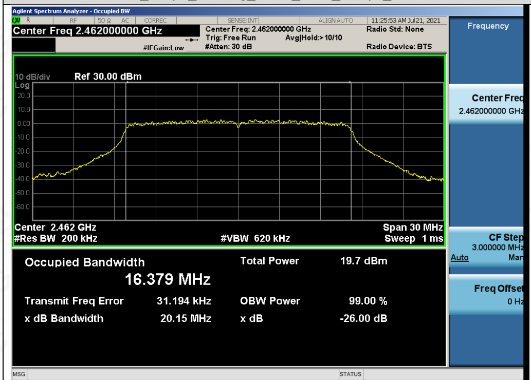
Test_Graph_802.11g_ANT1_2462_6Mbps_OBW
