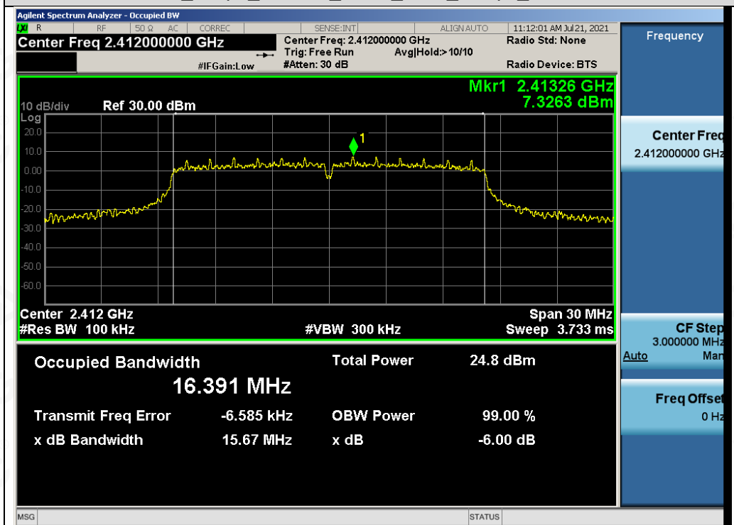
Test_Graph_802.11g_ANT1_2412_6Mbps_DTSBW
