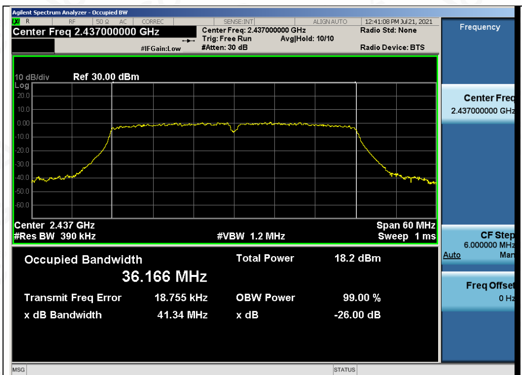
Test_Graph_802.11n40_ANT2_2437_MCS0_OBW
