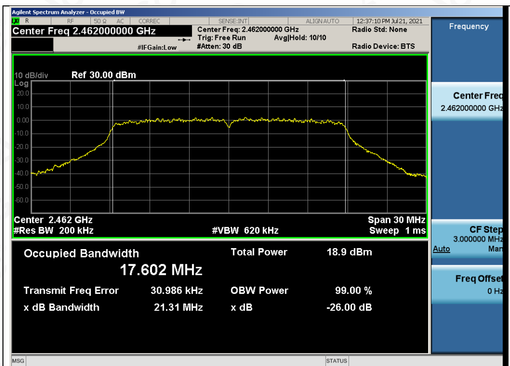
Test_Graph_802.11n20_ANT2_2462_MCS0_OBW
