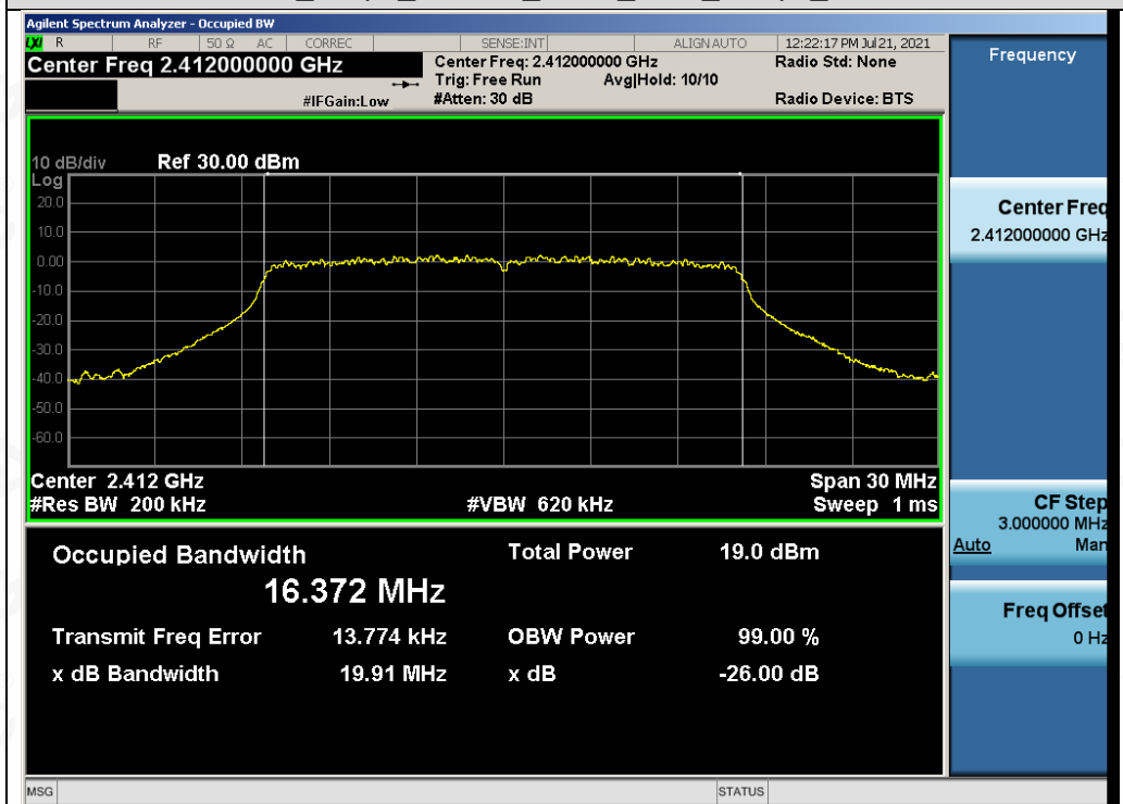
Test_Graph_802.11g_ANT2_2412_6Mbps_OBW
