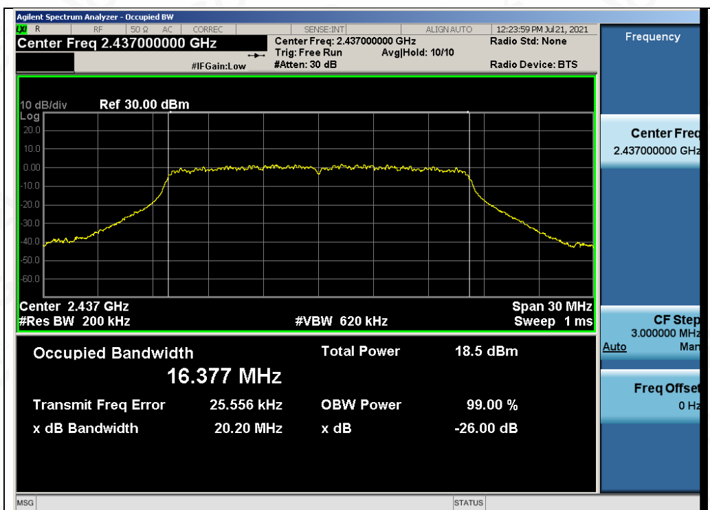
Test_Graph_802.11g_ANT2_2437_6Mbps_OBW
