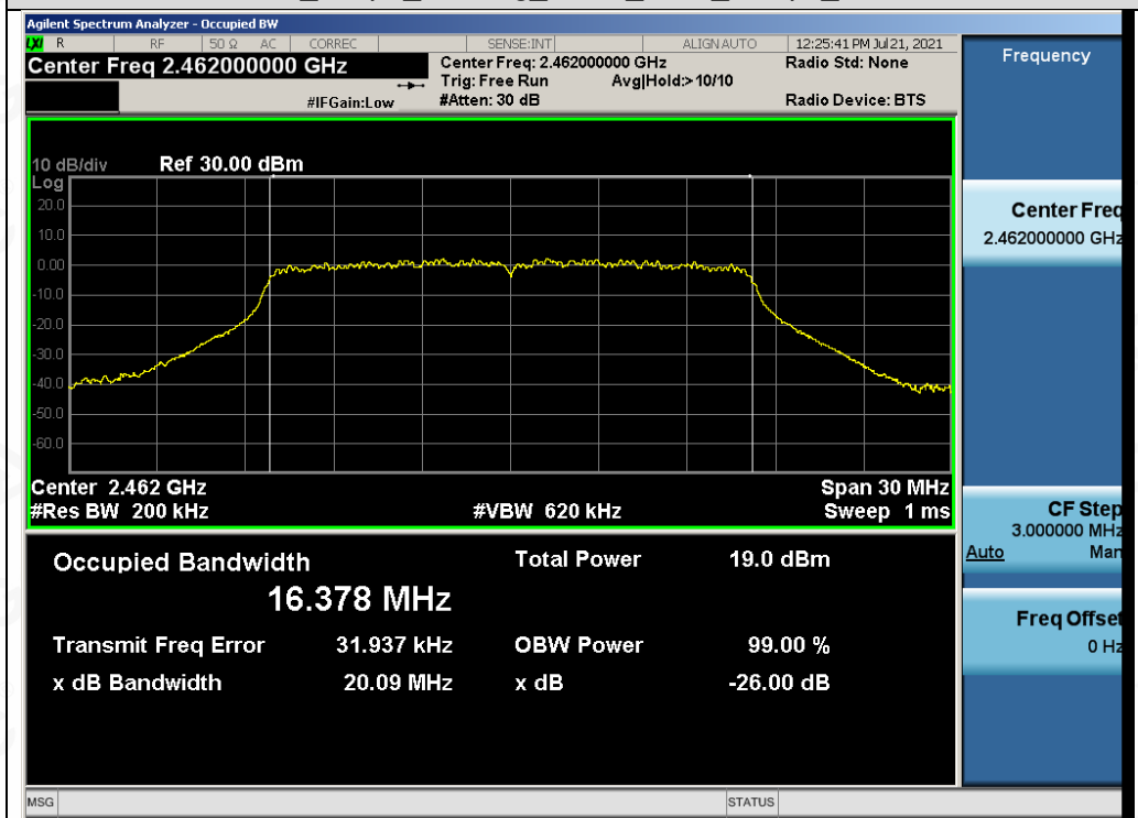
Test_Graph_802.11g_ANT2_2462_6Mbps_OBW
