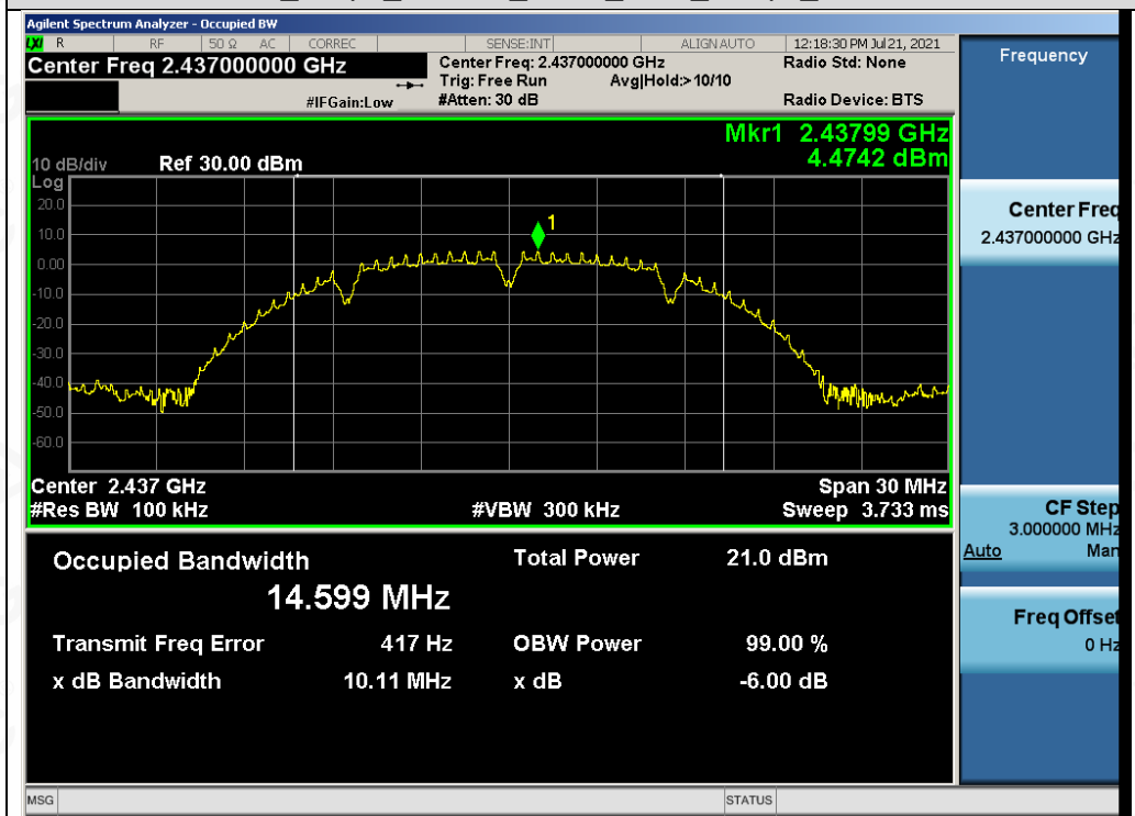
Test_Graph_802.11b_ANT2_2437_1Mbps_DTSBW
