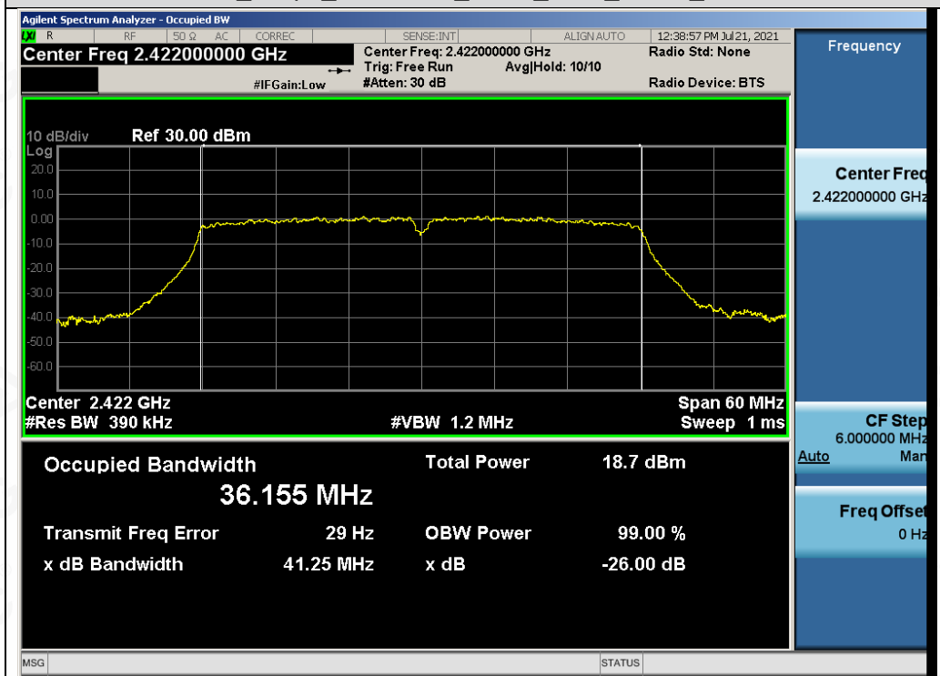
Test_Graph_802.11n40_ANT2_2422_MCS0_OBW
