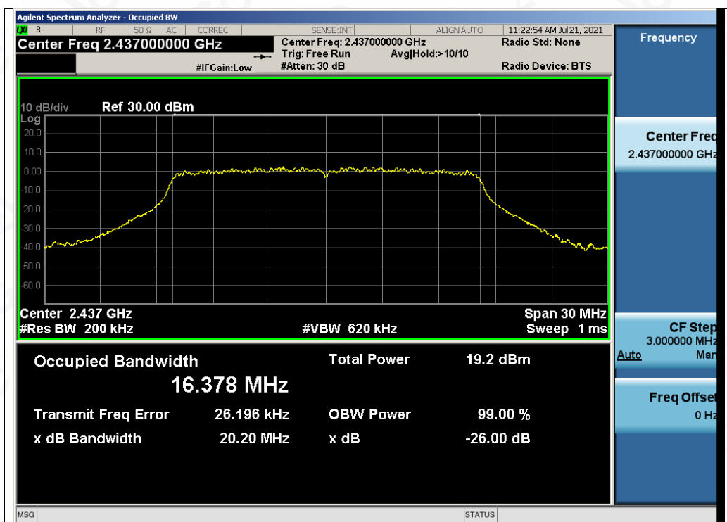
Test_Graph_802.11g_ANT1_2437_6Mbps_OBW
