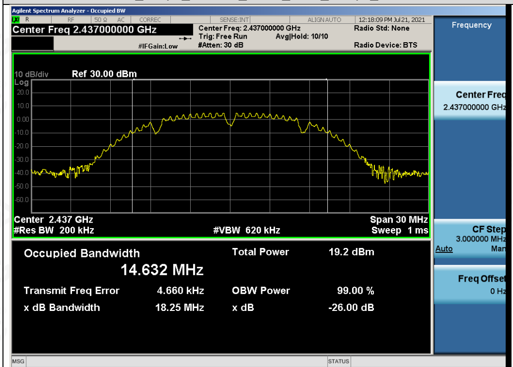
Test_Graph_802.11b_ANT2_2437_1Mbps_OBW
