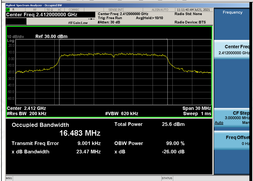
Test_Graph_802.11g_ANT1_2412_6Mbps_OBW
