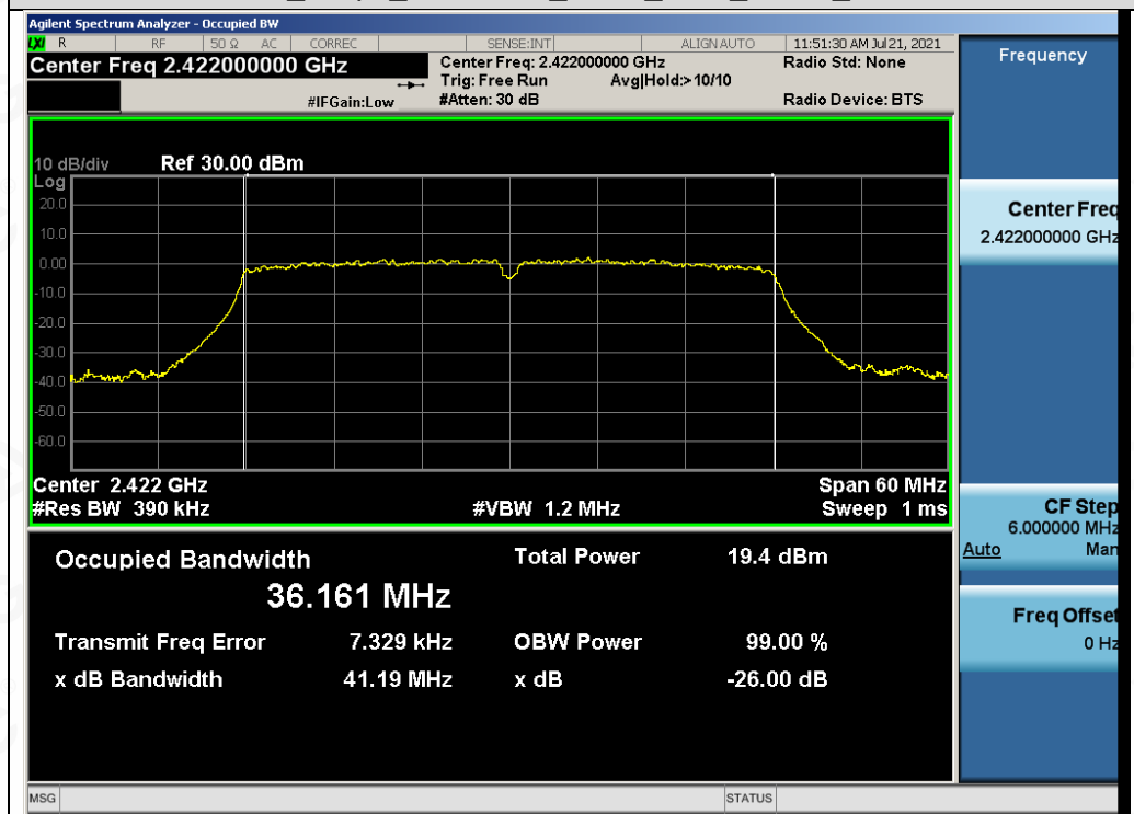
Test_Graph_802.11n40_ANT1_2422_MCS0_OBW
