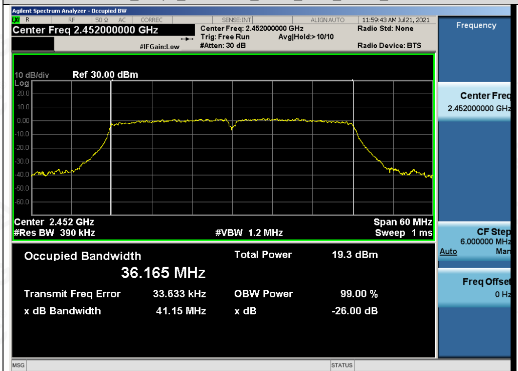
Test_Graph_802.11n40_ANT1_2452_MCS0_OBW
