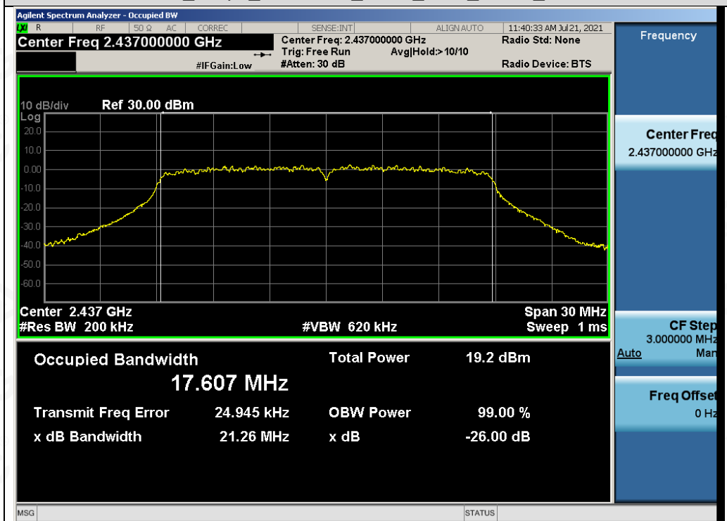
Test_Graph_802.11n20_ANT1_2437_MCS0_OBW
