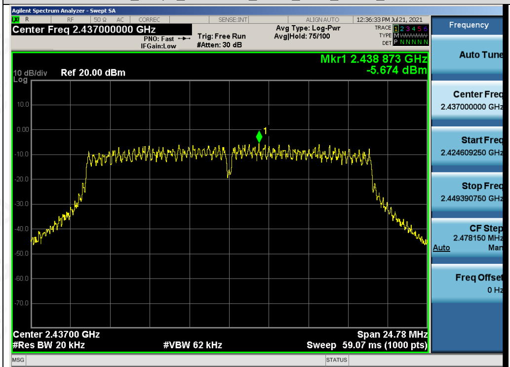
Test_Graph_802.11n20_ANT2_2437_MCS0_PSD
