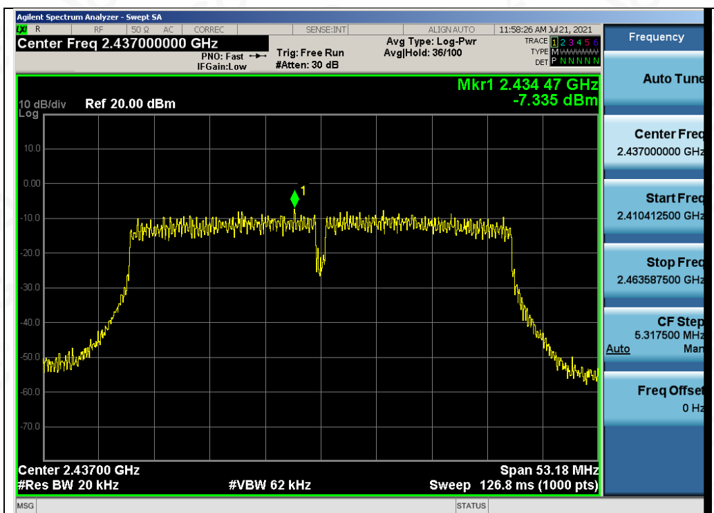
Test_Graph_802.11n40_ANT1_2437_MCS0_PSD
