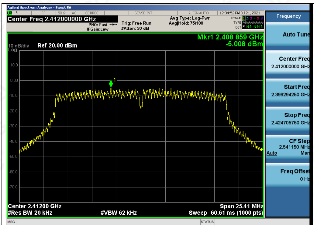
Test_Graph_802.11n20_ANT2_2412_MCS0_PSD
