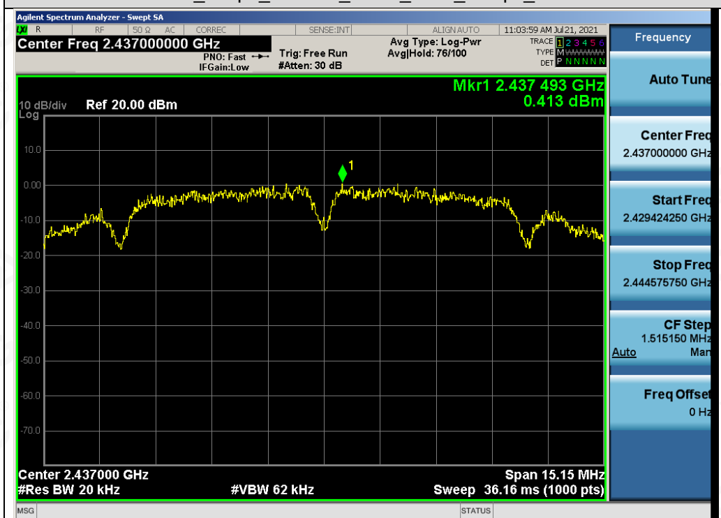
Test_Graph_802.11b_ANT1_2437_1Mbps_PSD
