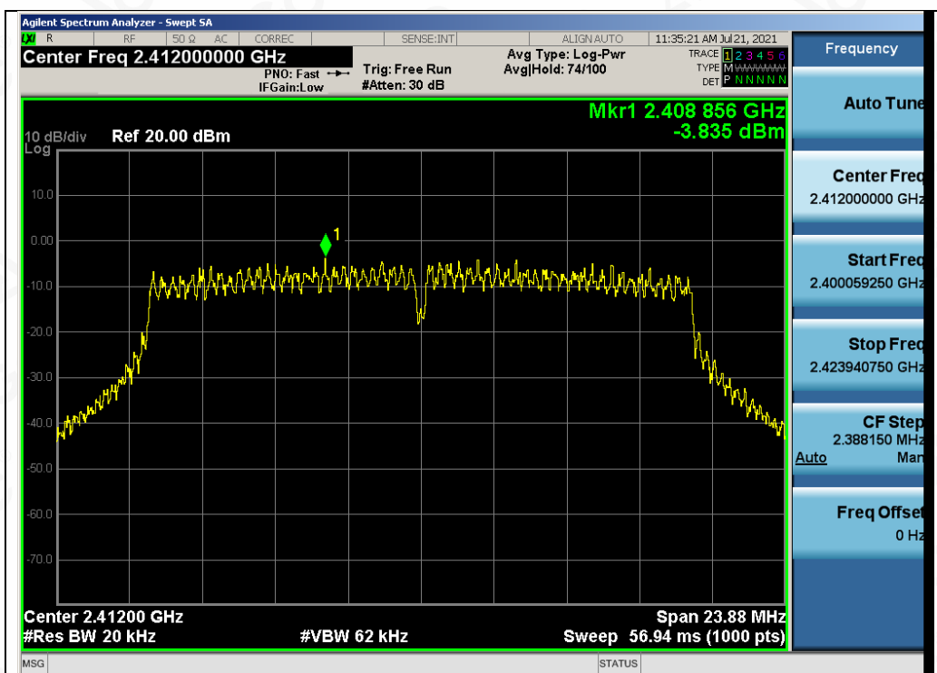
Test_Graph_802.11n20_ANT1_2412_MCS0_PSD
