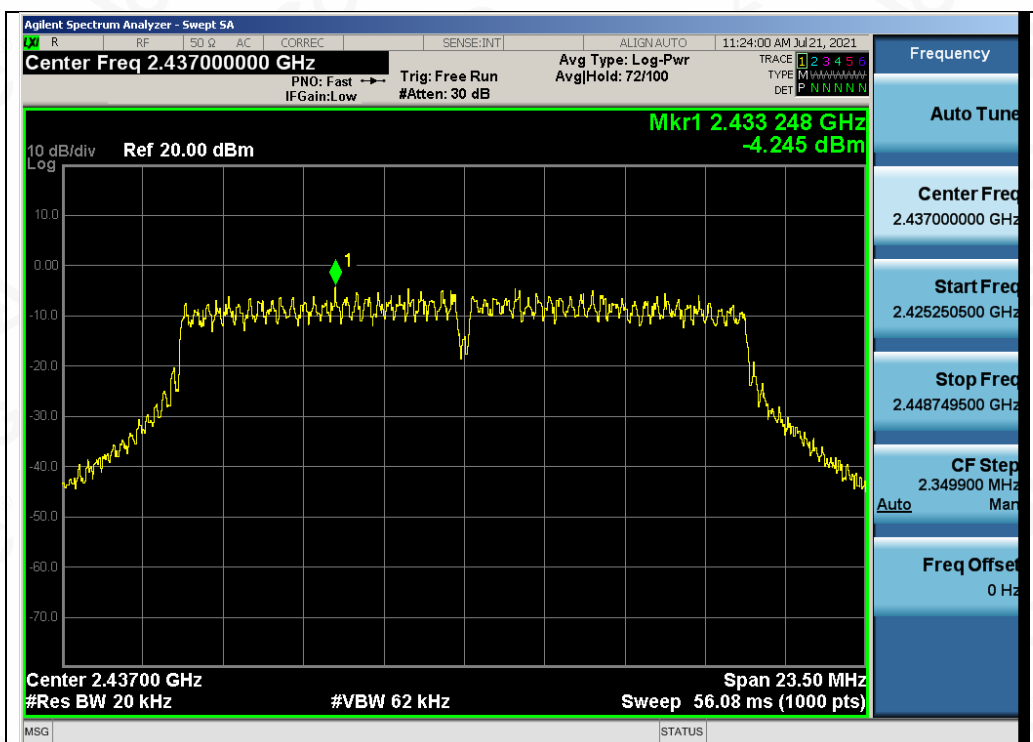
Test_Graph_802.11g_ANT1_2437_6Mbps_PSD
