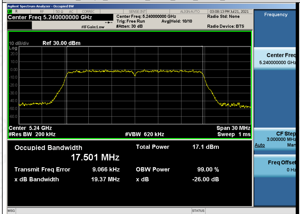
Test_Graph_802.11n20_ANT2_5240_MCS0_OBW
