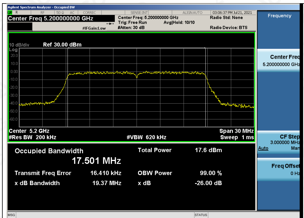
Test_Graph_802.11n20_ANT2_5200_MCS0_OBW
