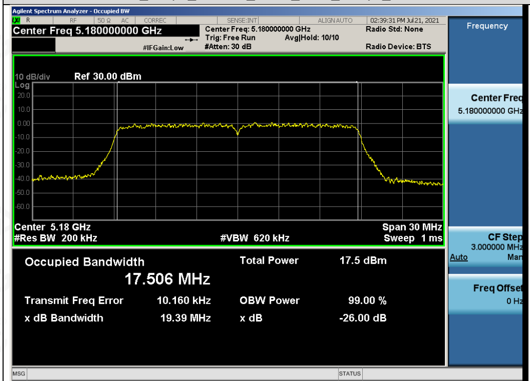
Test_Graph_802.11n20_ANT1_5180_MCS0_OBW
