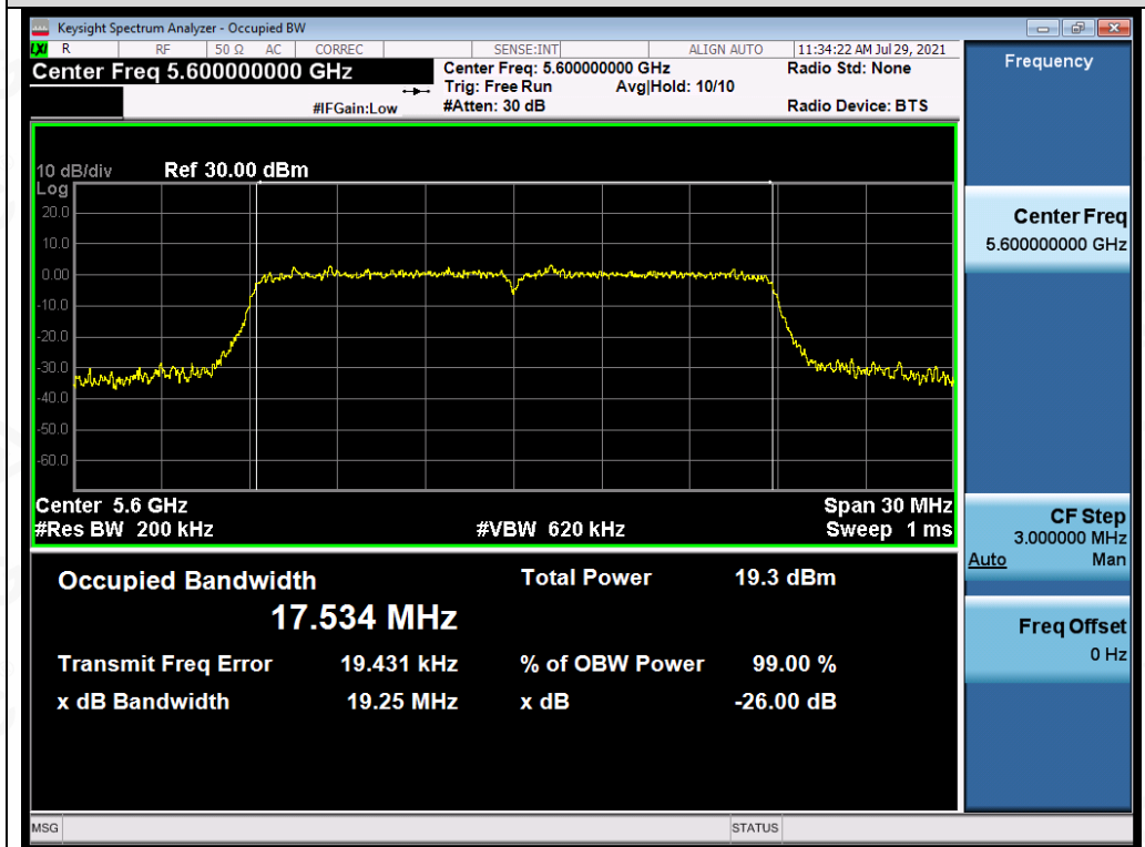
Test_Graph_802.11ac20_ANT2_5600_MCS0_OBW
