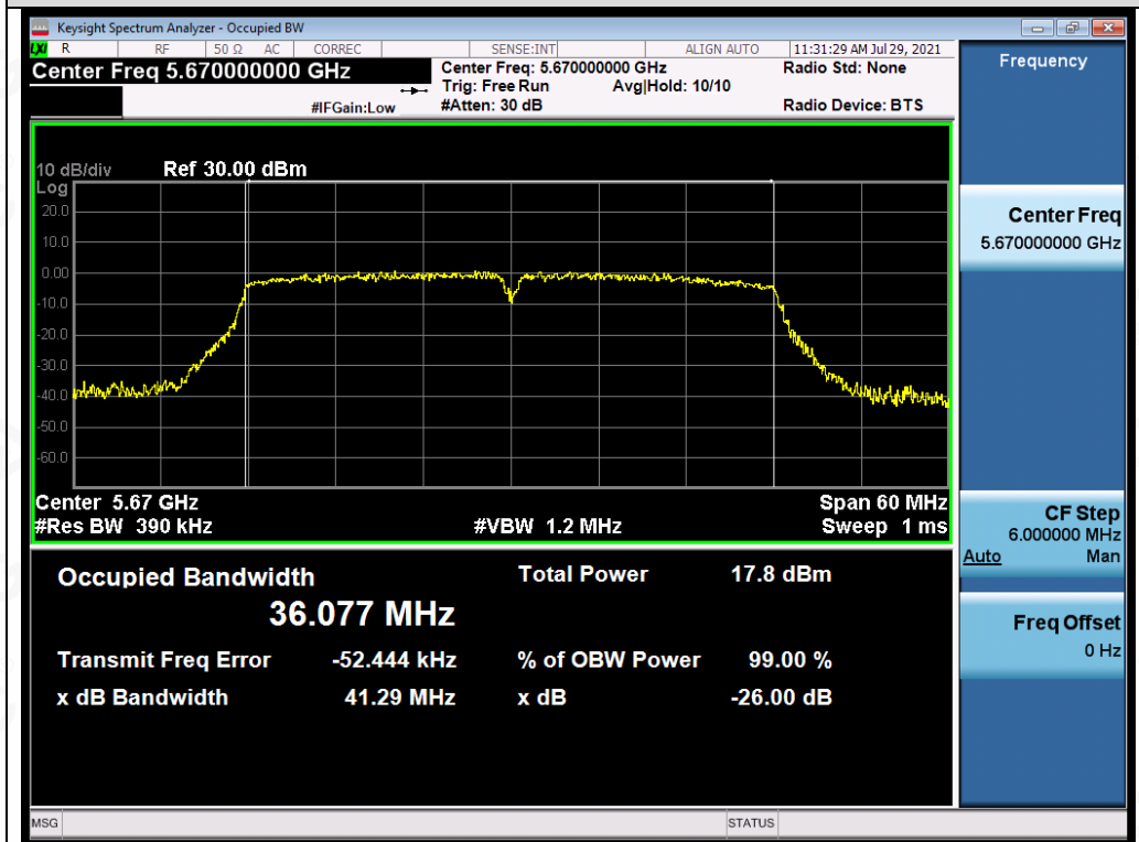
Test_Graph_802.11n40_ANT2_5670_MCS0_OBW
