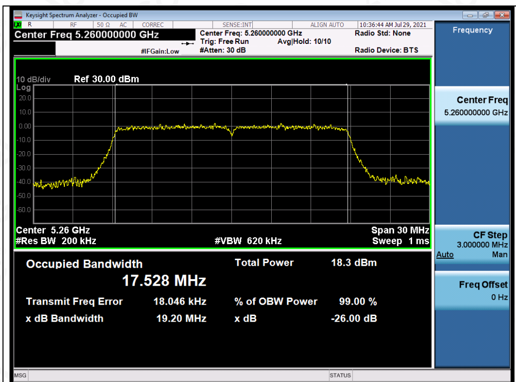
Test_Graph_802.11ac20_ANT2_5260_MCS0_OBW
