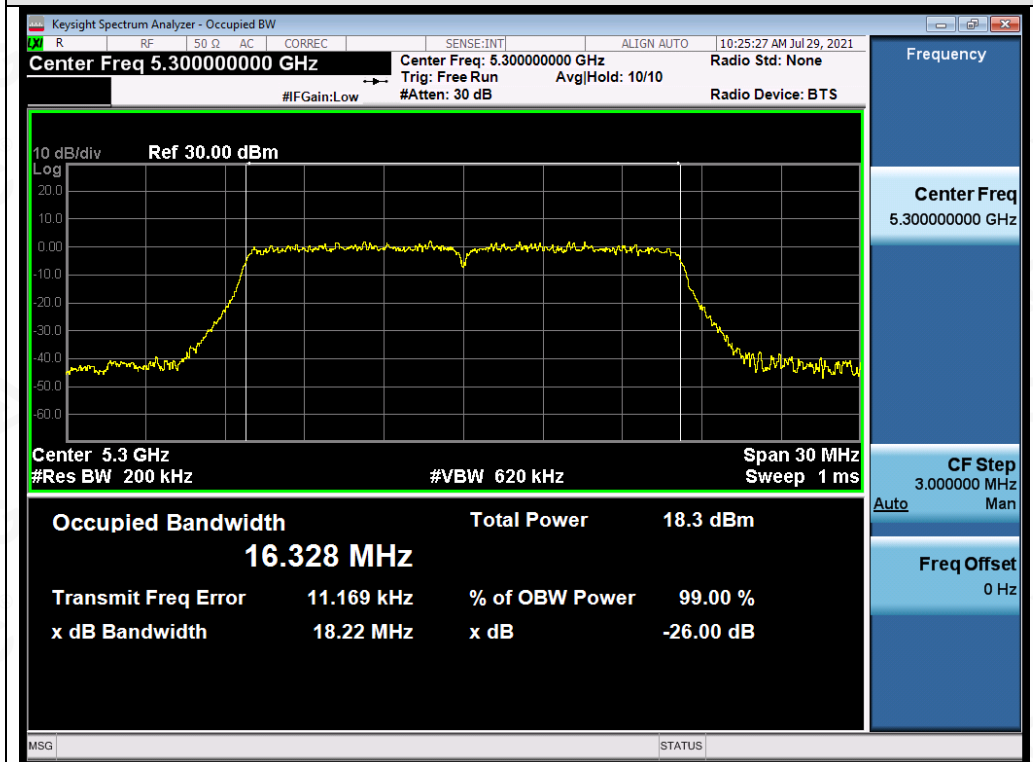
Test_Graph_802.11a_ANT2_5300_6Mbps_OBW
