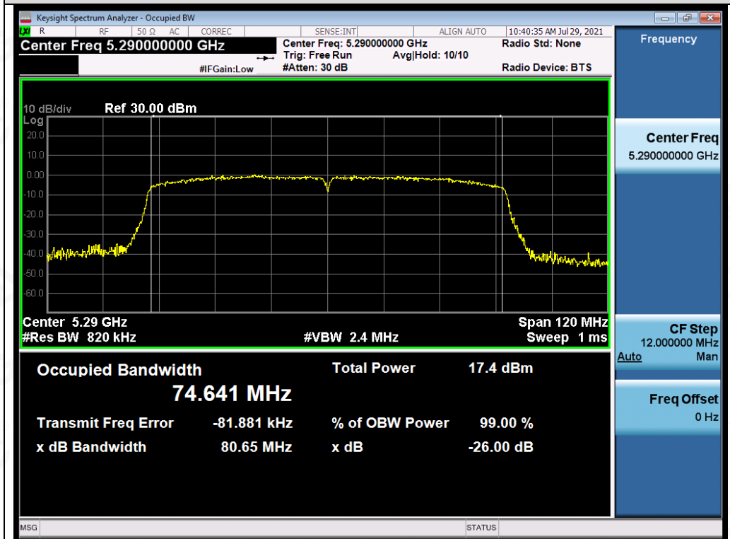
Test_Graph_802.11ac80_ANT2_5290_MCS9_OBW
