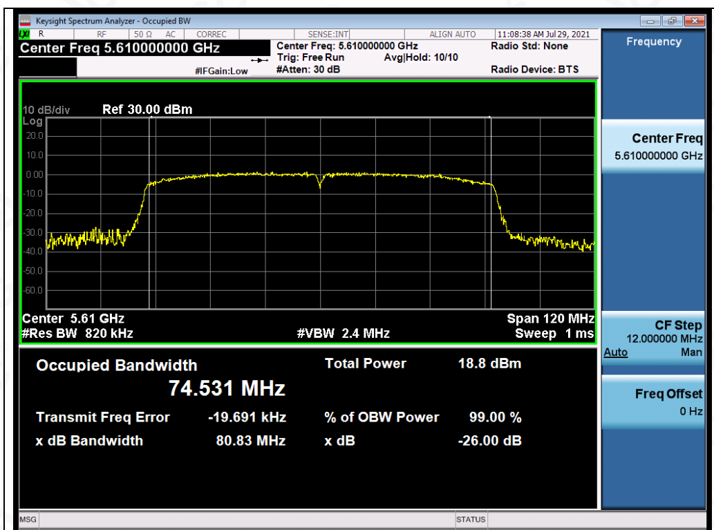
Test_Graph_802.11ac80_ANT1_5610_MCS9_OBW
