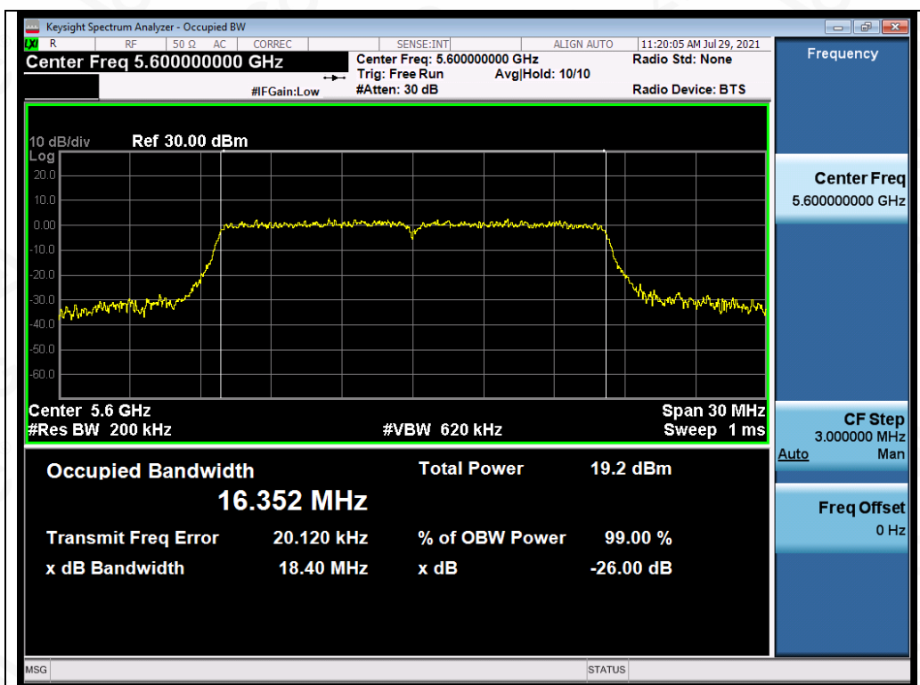
Test_Graph_802.11a_ANT2_5600_6Mbps_OBW
