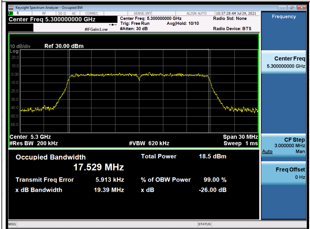
Test_Graph_802.11ac20_ANT2_5300_MCS0_OBW
