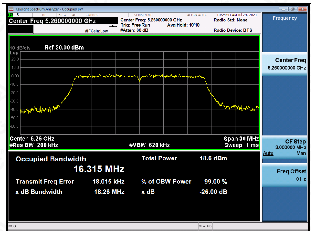
Test_Graph_802.11a_ANT2_5260_6Mbps_OBW
