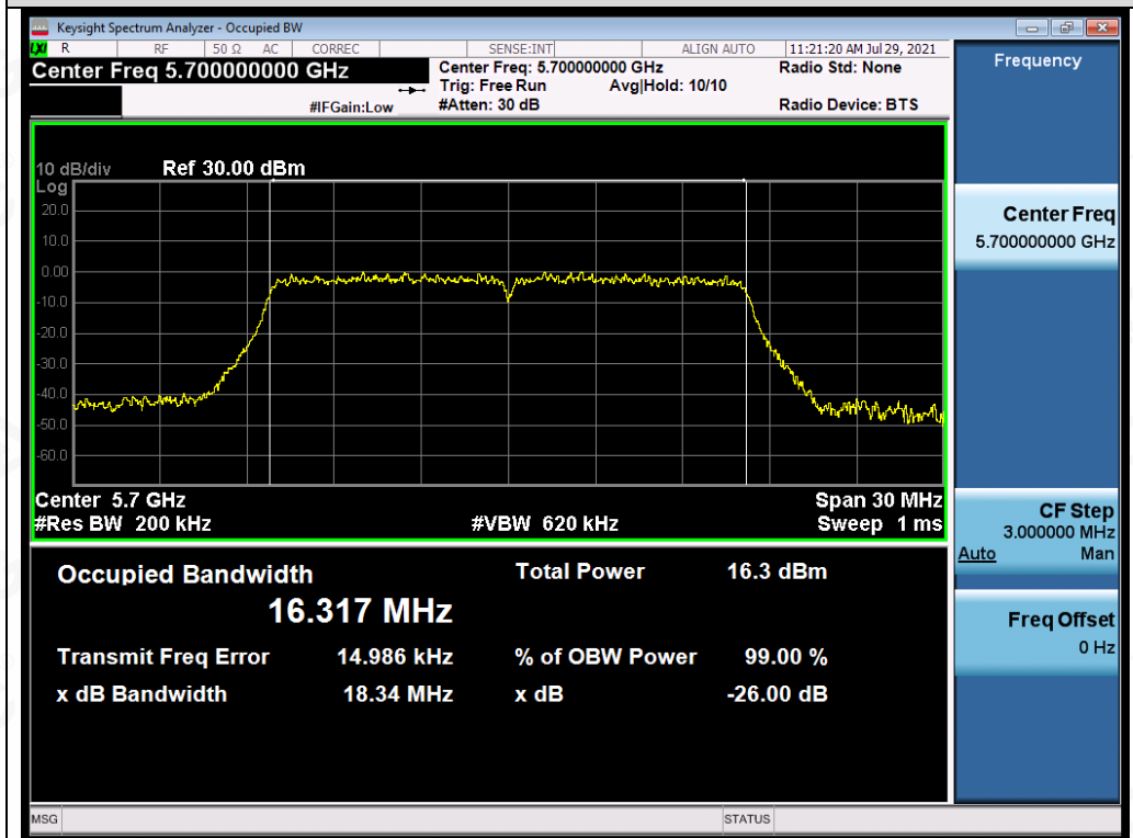
Test_Graph_802.11a_ANT2_5700_6Mbps_OBW
