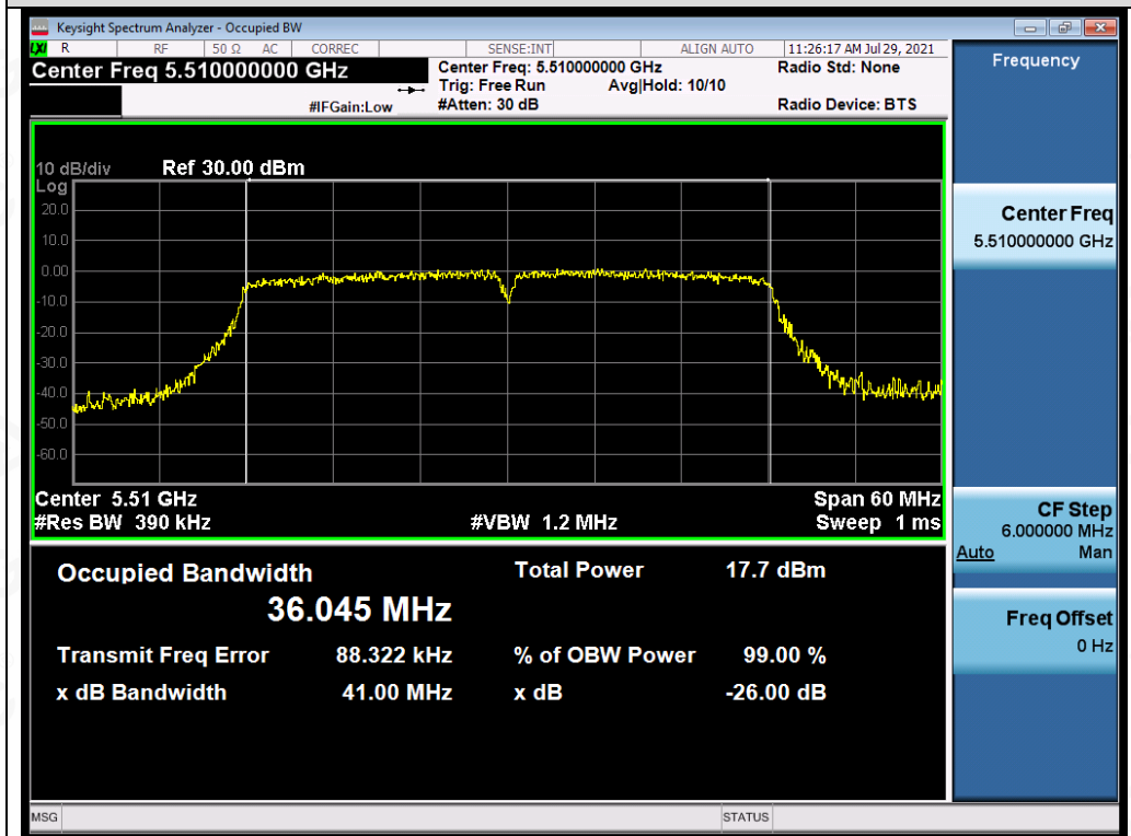
Test_Graph_802.11n40_ANT2_5510_MCS0_OBW
