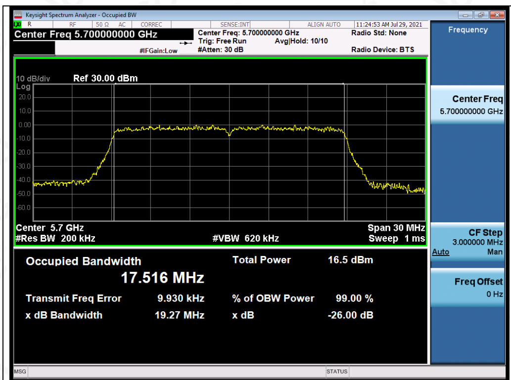
Test_Graph_802.11n20_ANT2_5700_MCS0_OBW
