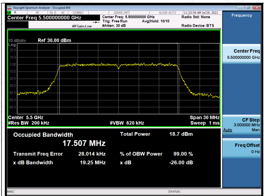
Test_Graph_802.11n20_ANT2_5500_MCS0_OBW
