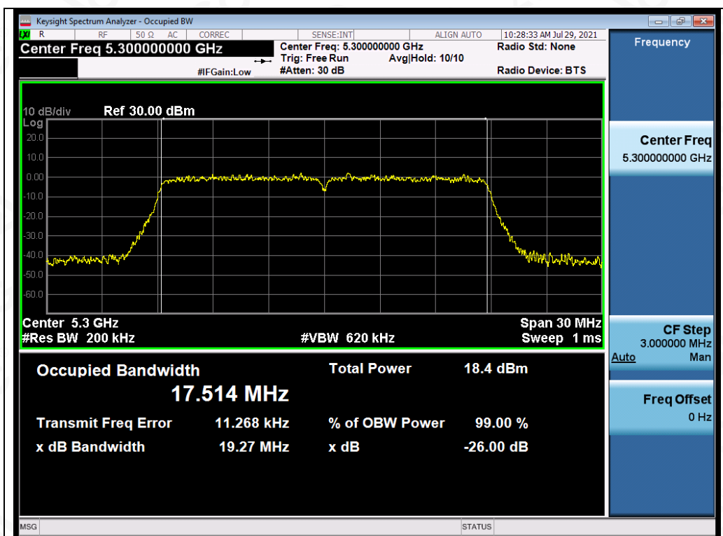
Test_Graph_802.11n20_ANT2_5300_MCS0_OBW
