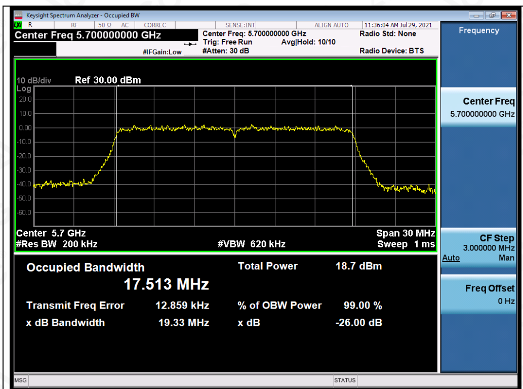
Test_Graph_802.11ac20_ANT2_5700_MCS9_OBW
