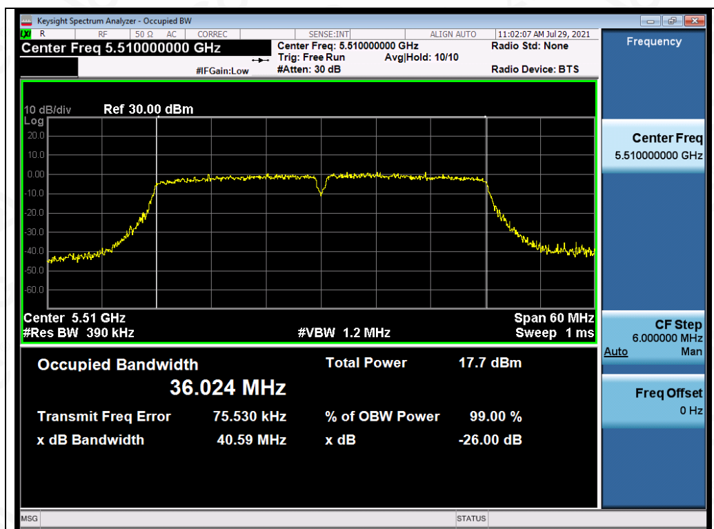
Test_Graph_802.11ac40_ANT1_5510_MCS9_OBW
