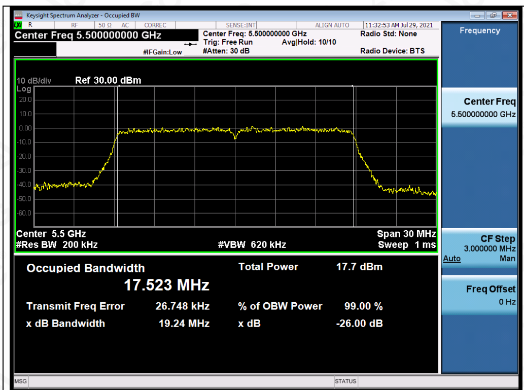
Test_Graph_802.11ac20_ANT2_5500_MCS0_OBW
