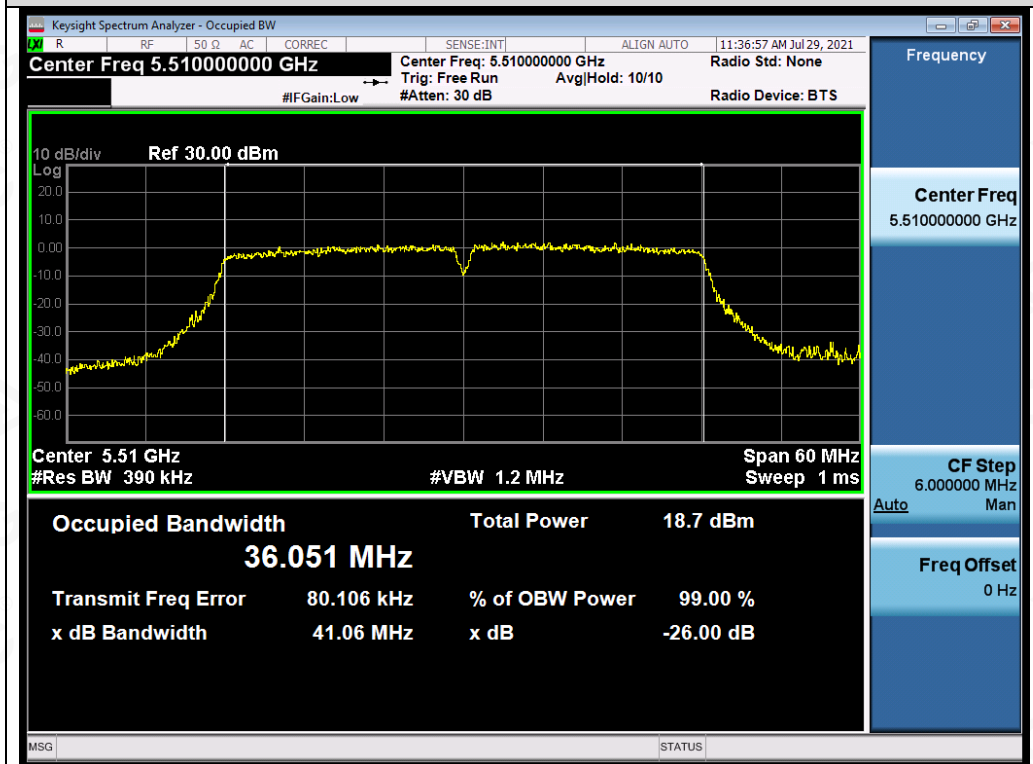
Test_Graph_802.11ac40_ANT2_5510_MCS9_OBW
