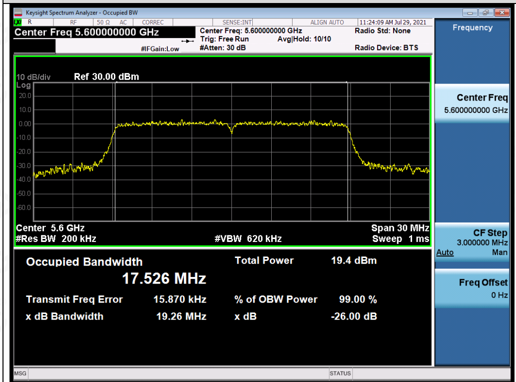
Test_Graph_802.11n20_ANT2_5600_MCS0_OBW
