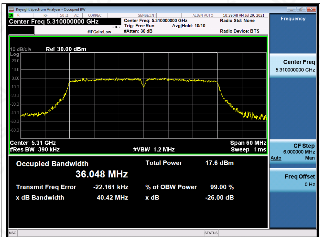
Test_Graph_802.11ac40_ANT2_5310_MCS9_OBW
