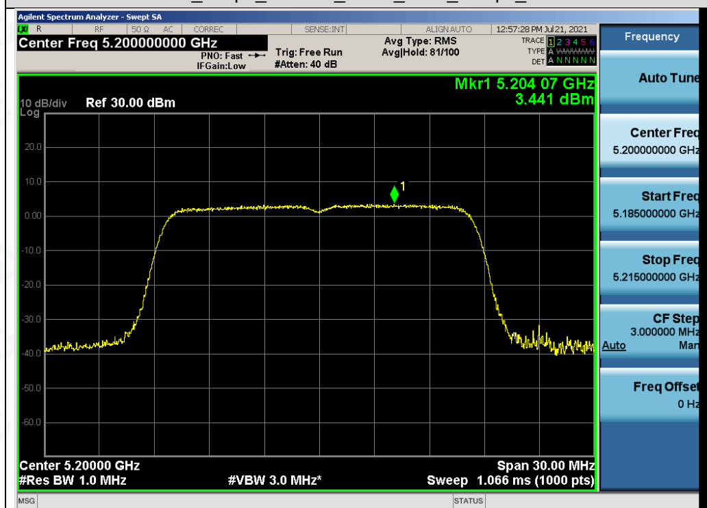
Test_Graph_802.11a_ANT1_5200_6Mbps_PSD
