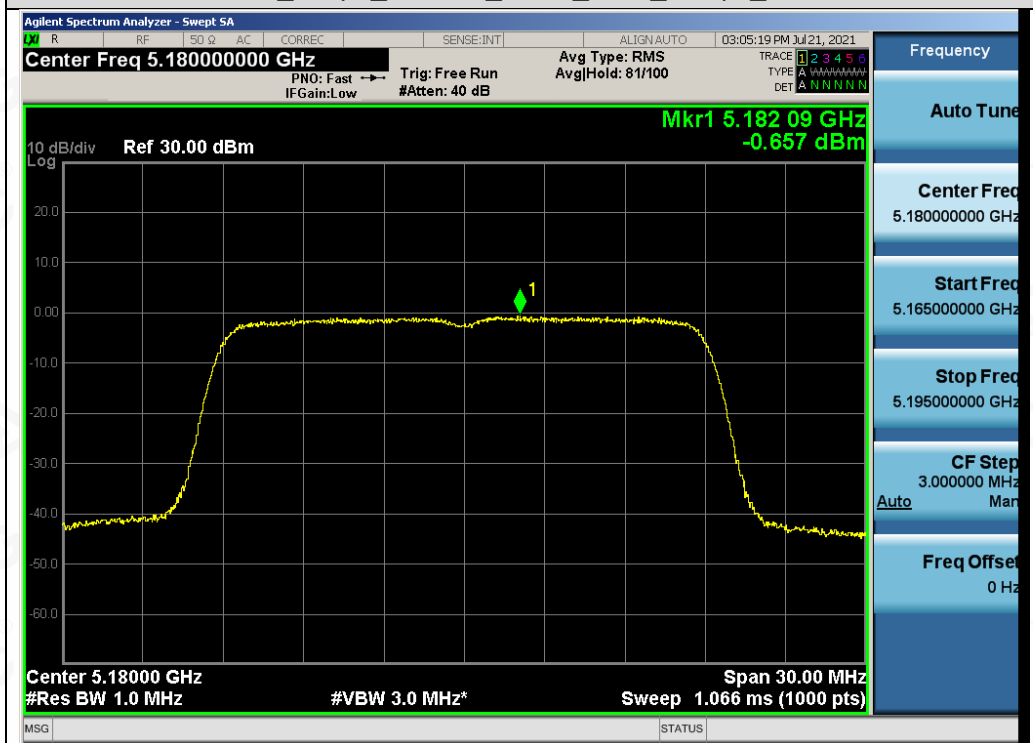
Test_Graph_802.11n20_ANT2_5180_MCS0_PSD
