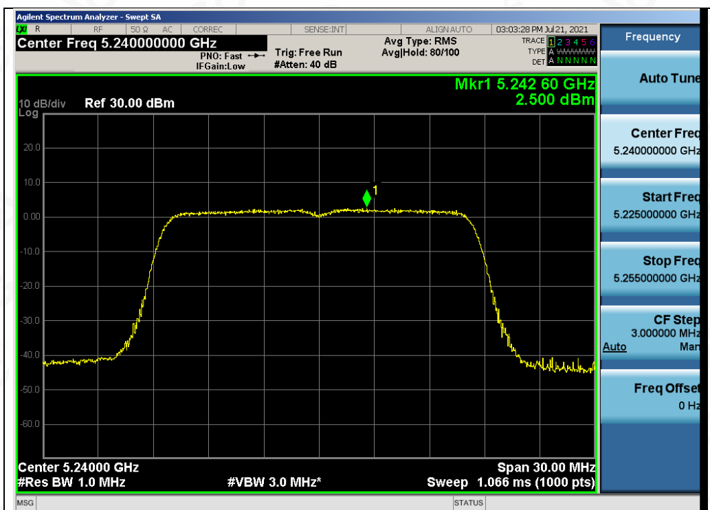
Test_Graph_802.11a_ANT2_5240_6Mbps_PSD
