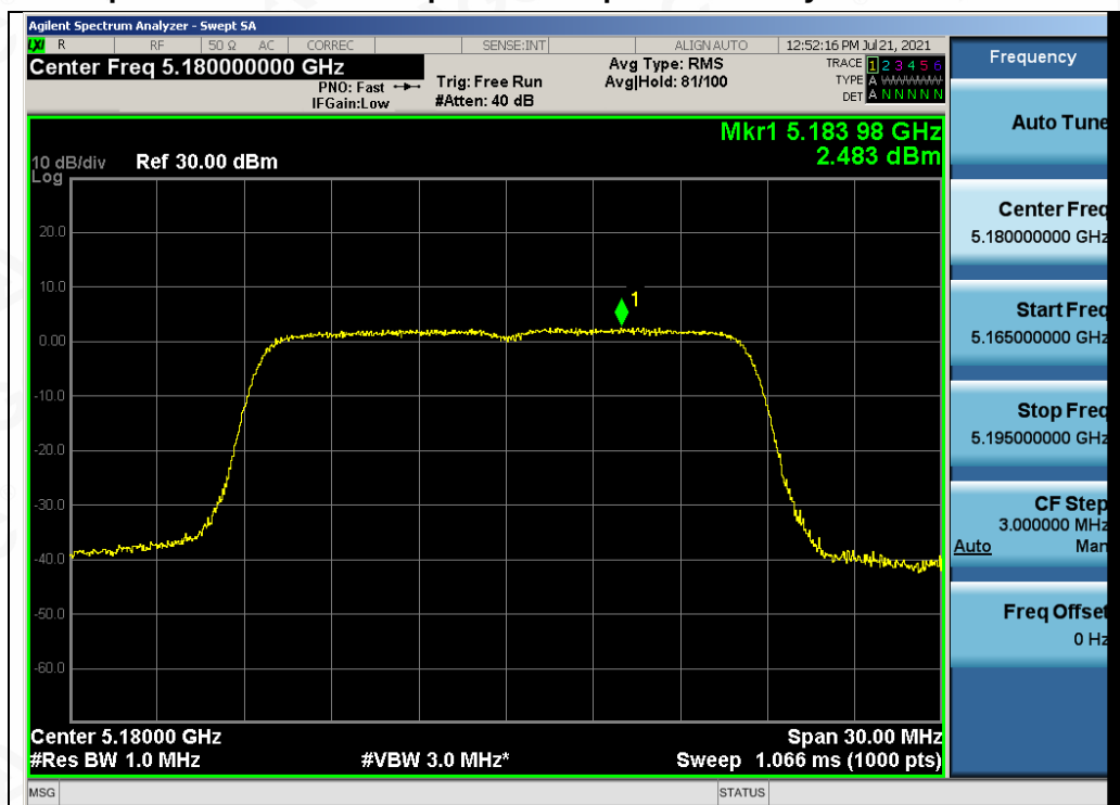
Test_Graph_802.11a_ANT1_5180_6Mbps_PSD
